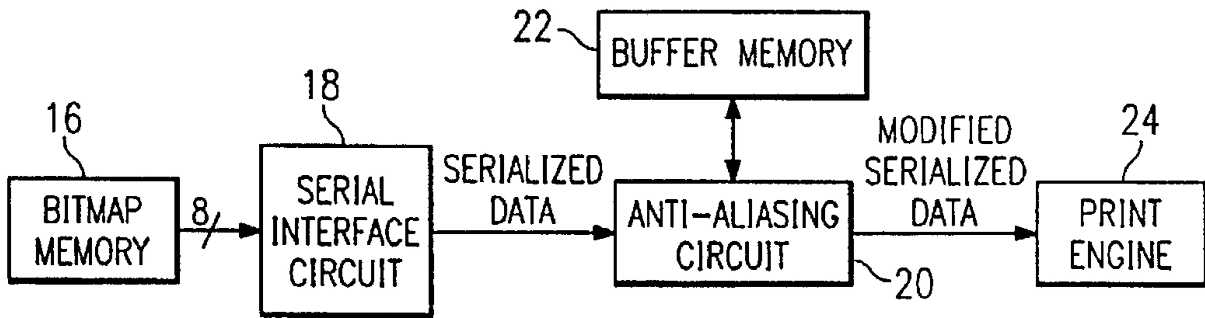
FIG. 2 (PRIOR ART)
