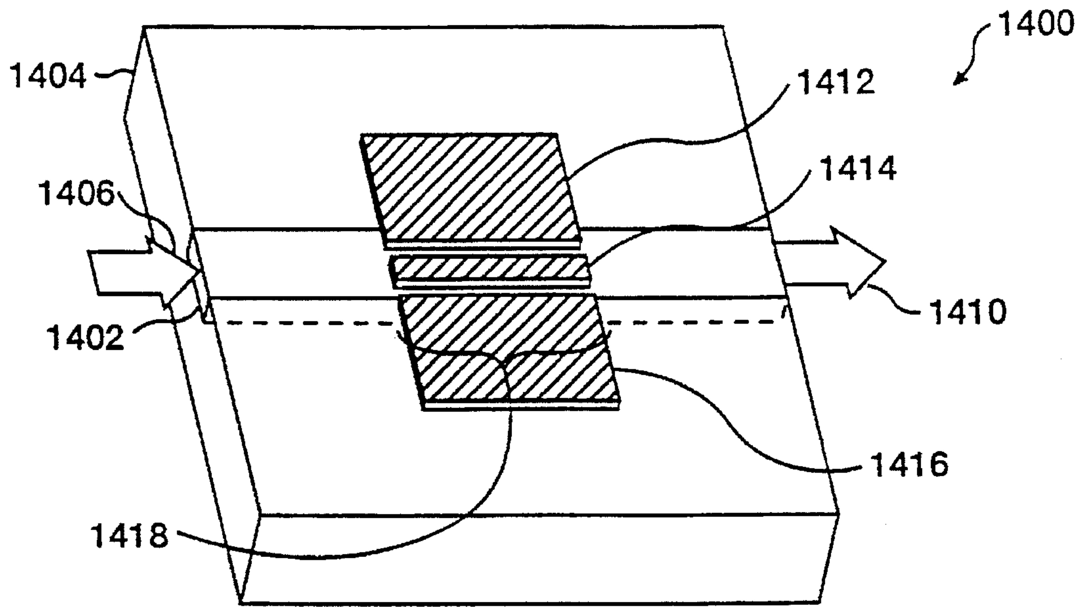
Figure 50 (Prior Art)
