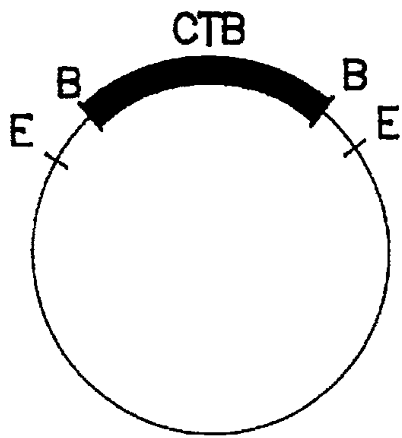
M13 mp7 B43
