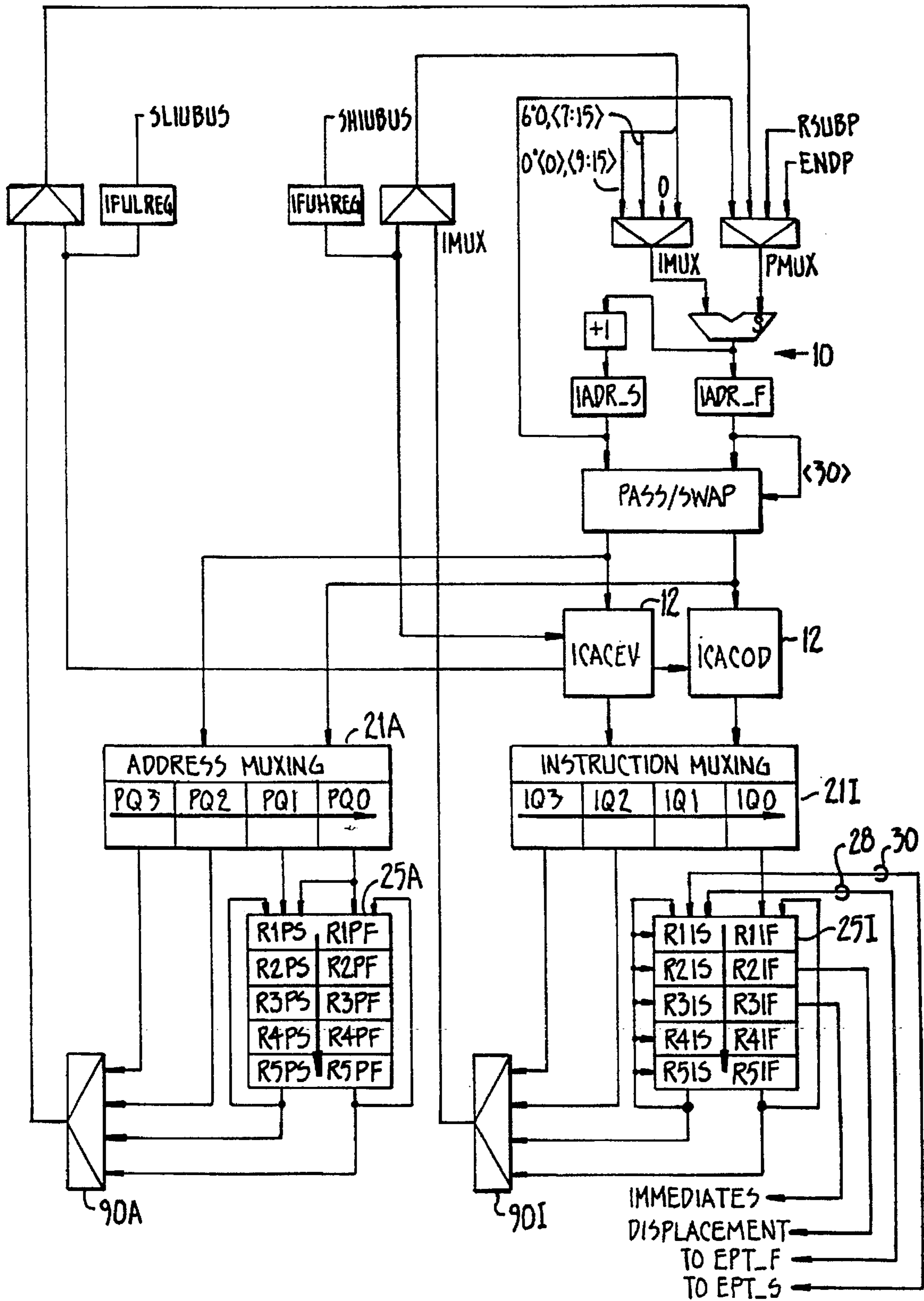
INSTRUCTION CACHE, QUEUE, AND PIPELINE
