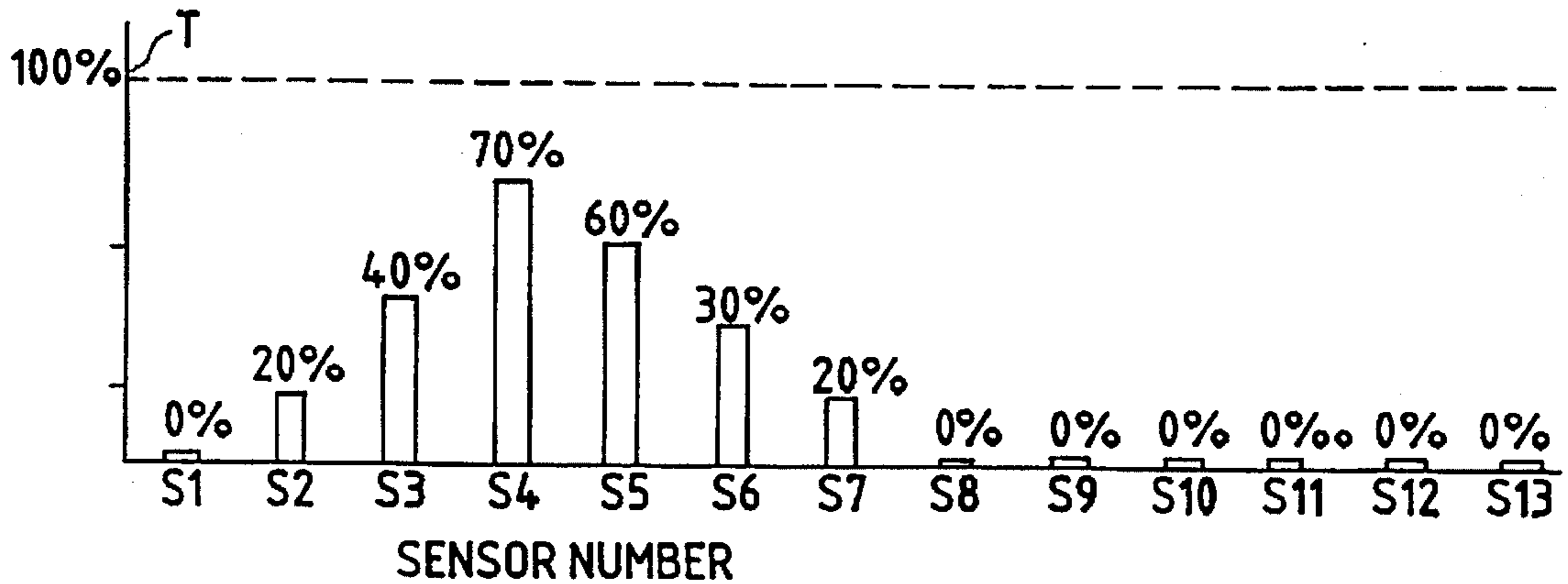
SMOKE READING % OF ALARM LEVEL
