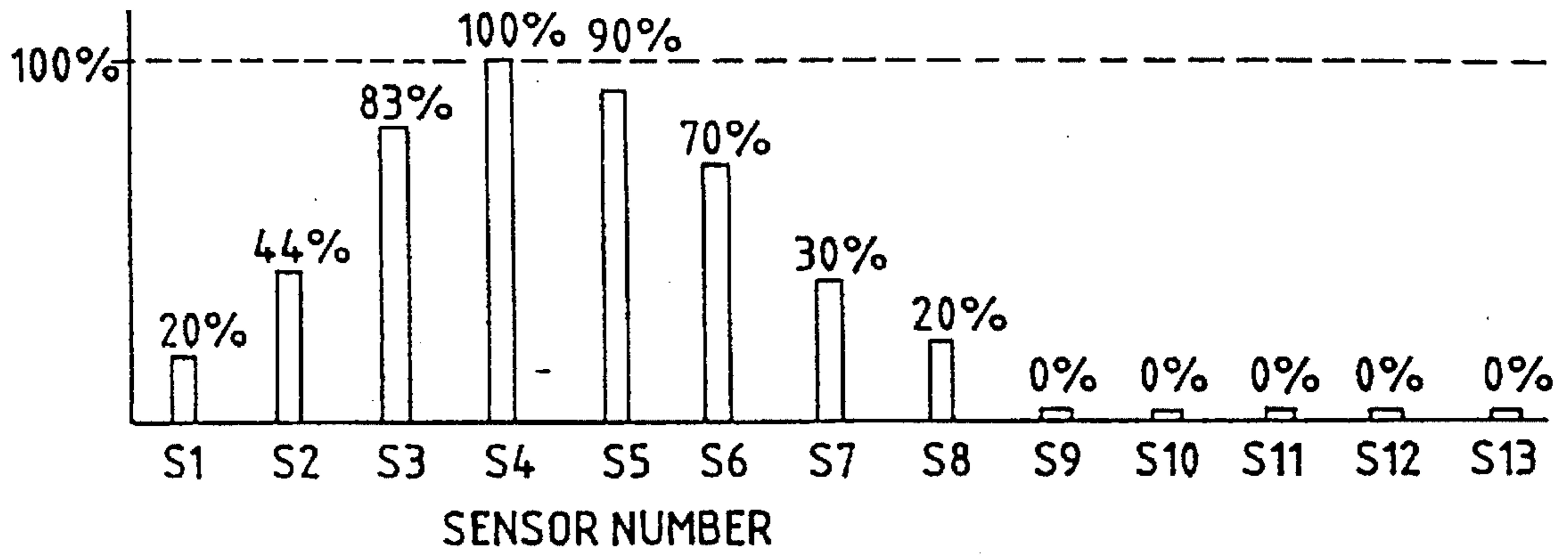
RMS COMBINED SMOKE READING (% OF ALARM)
