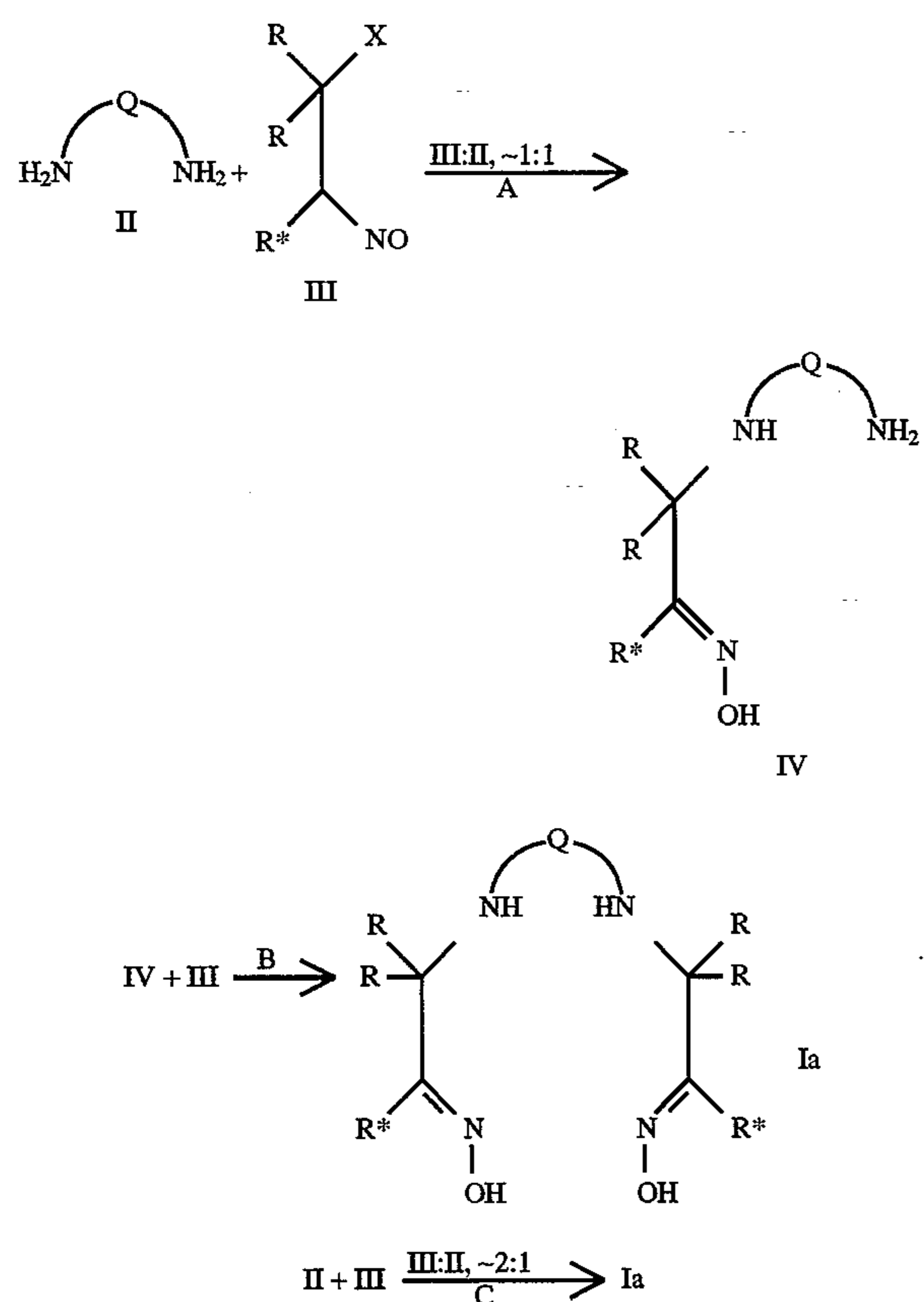
Reaction Scheme 1 Preparation of Compounds of the Formula Ia
