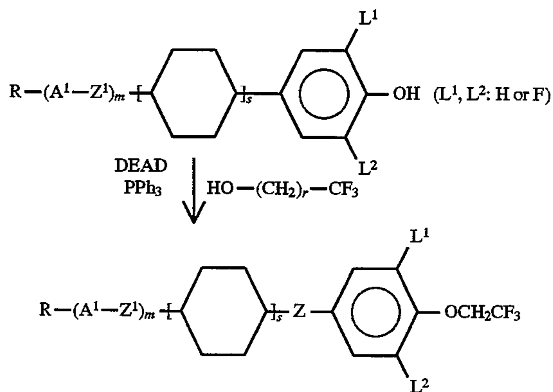
Scheme 13
