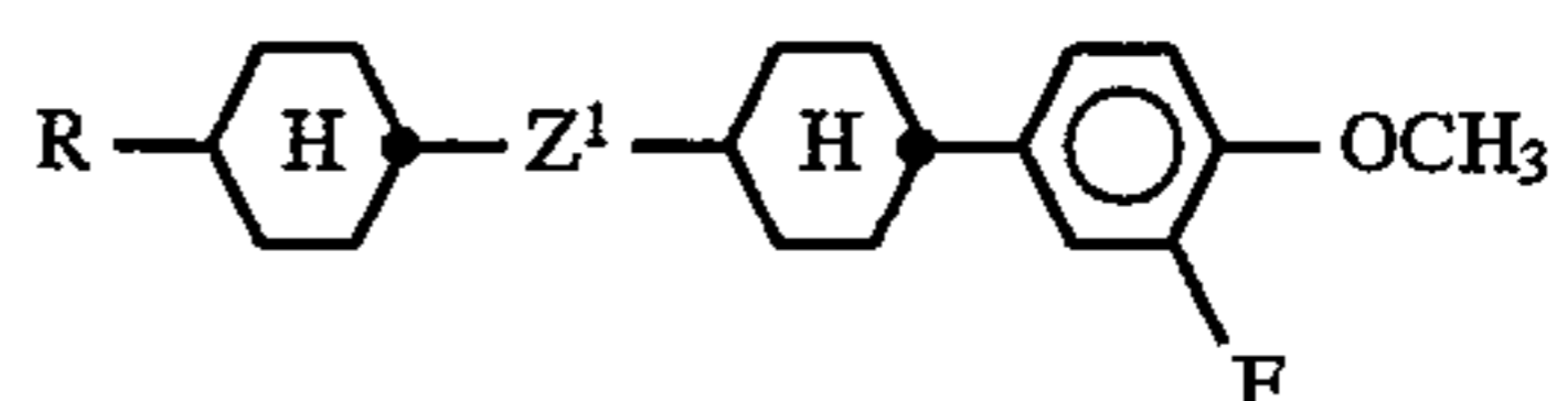
-continued Scheme 5
