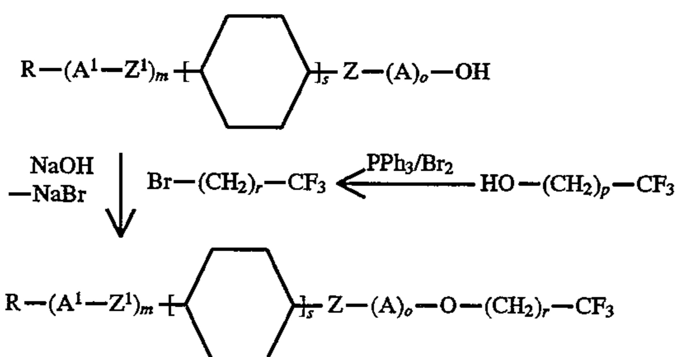
Scheme 11
