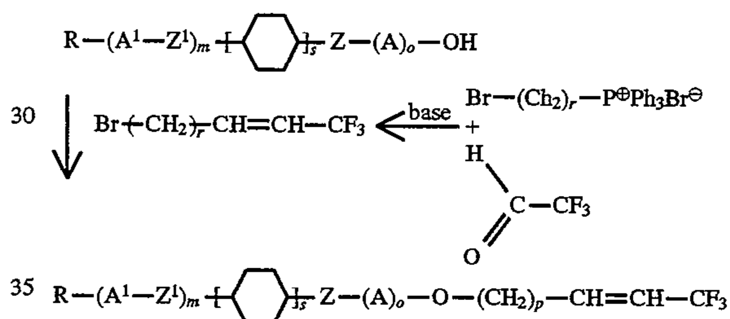
Scheme 12
