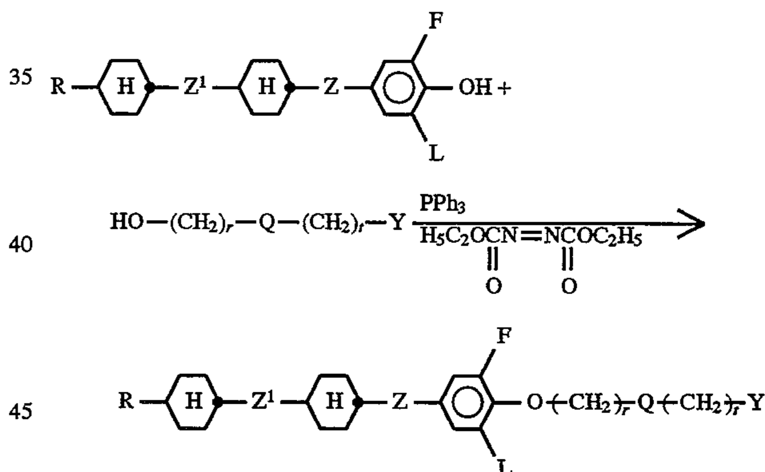
Scheme 6
