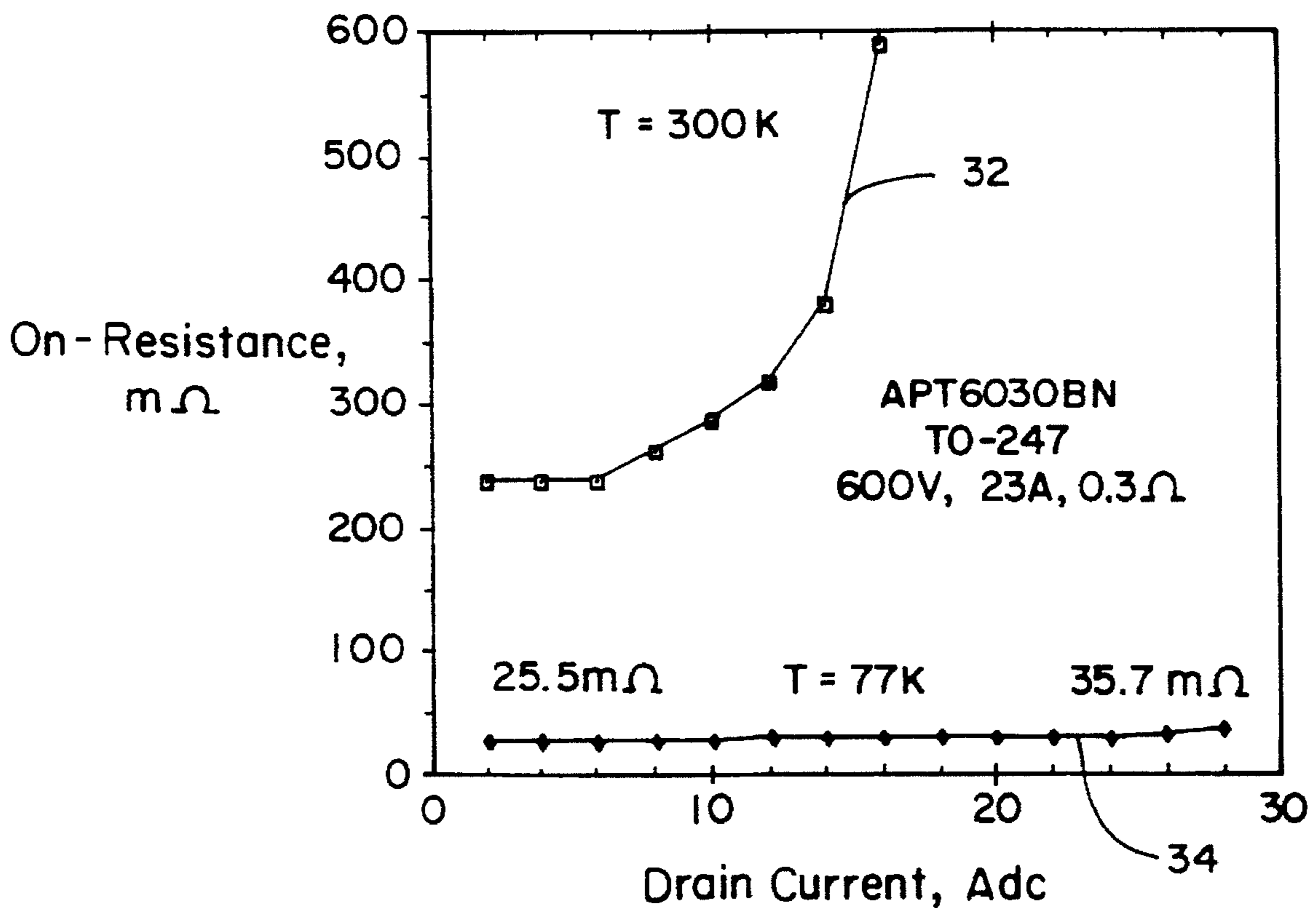
APT6030BN, On-Resistance vs Drain Current
