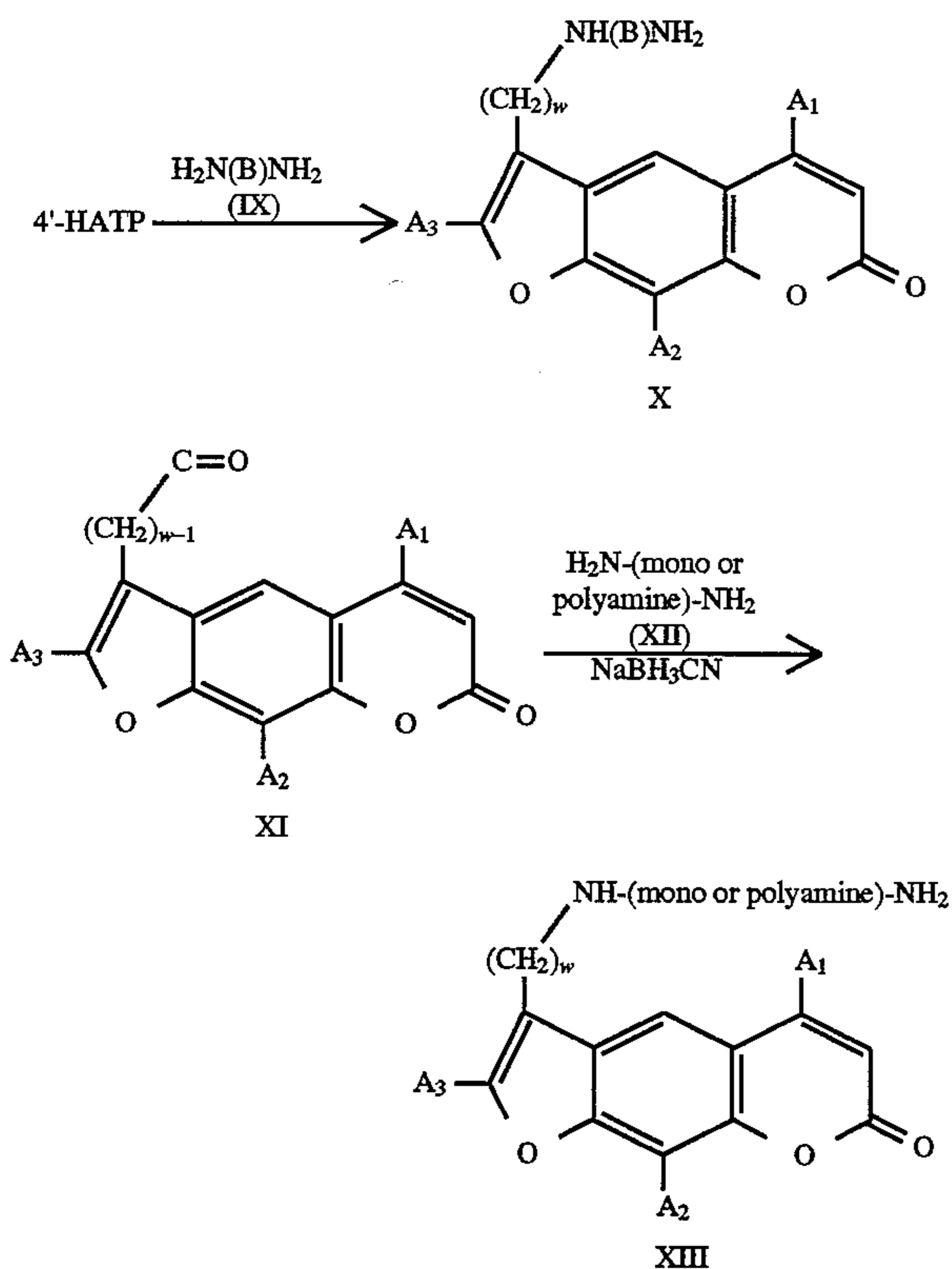
SCHEMATIC 3
