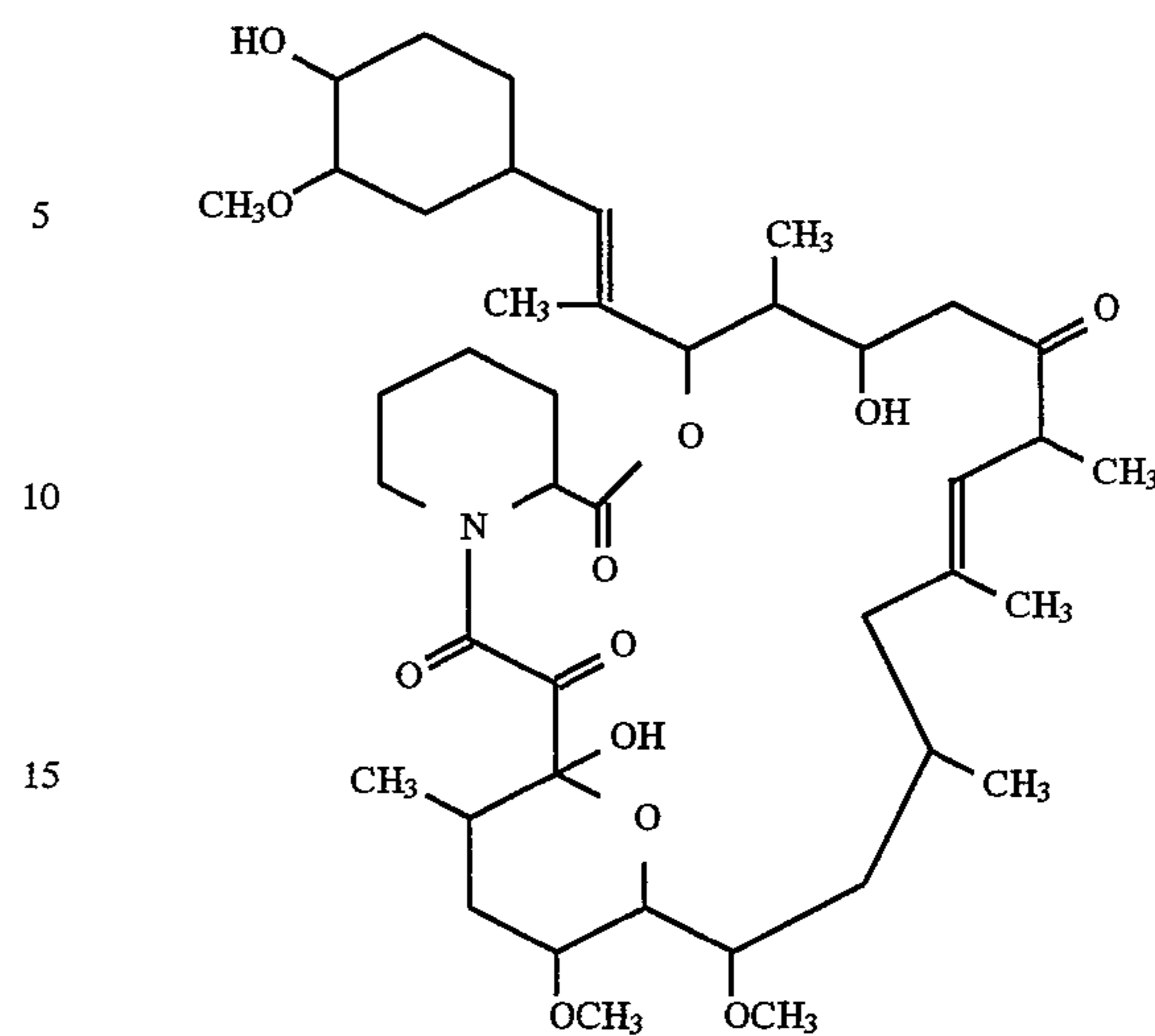
1,14-Dihydroxy-12-[2-(4-hydroxy-3-methoxycyclohexyl)-1-methylvinyl]-23,25-dimethoxy-13,19,17,21,27-pentamethyl-11,28-dioxo-4-azatricyclo[22.3.1.0 4.9 ]-octacos-18-ene-2,3,10,16-tetraone
