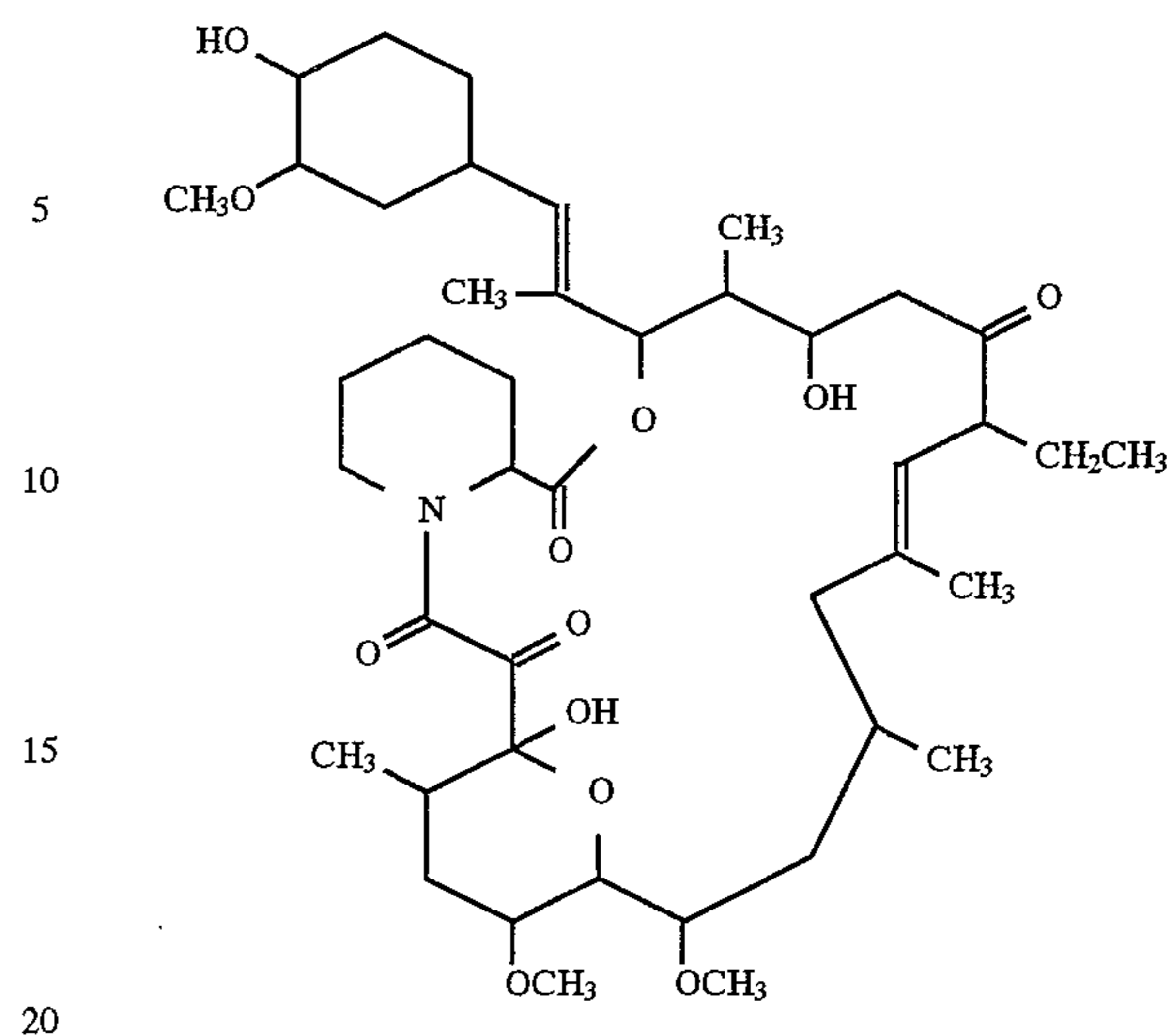
17-Ethyl-1,14-dihydroxy-12-[2-(4-hydroxy-3-methoxycyclohexyl)-1-methylvinyl]-23,25-dimethoxy-13,19,21,27-tetramethyl-11,28-dioxo-4-azatricyclo-[22.3.1.0 4,9 ]octacos-18-ene-2,3,10,16-tetraone
