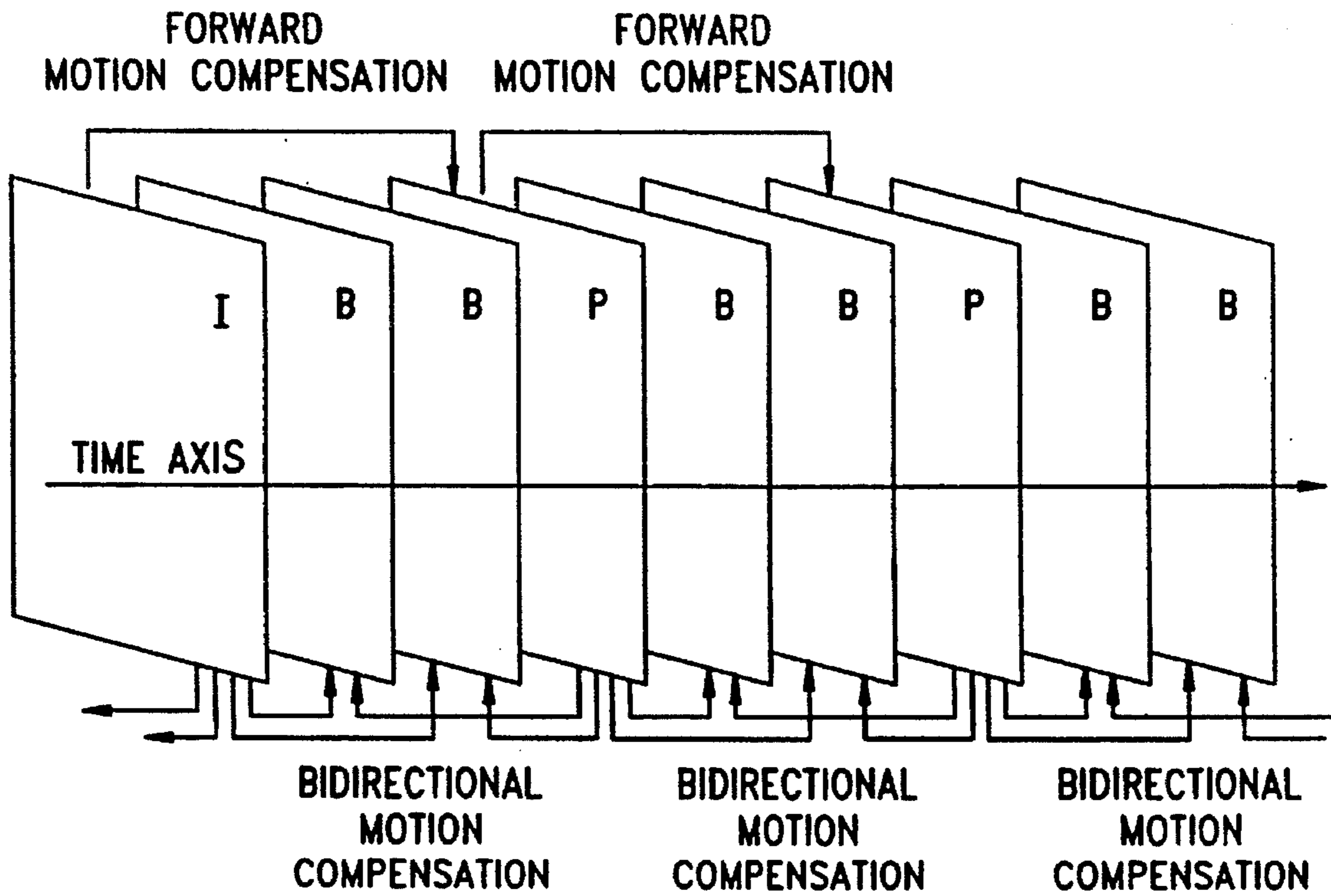
FIG. 5 PRIOR ART
