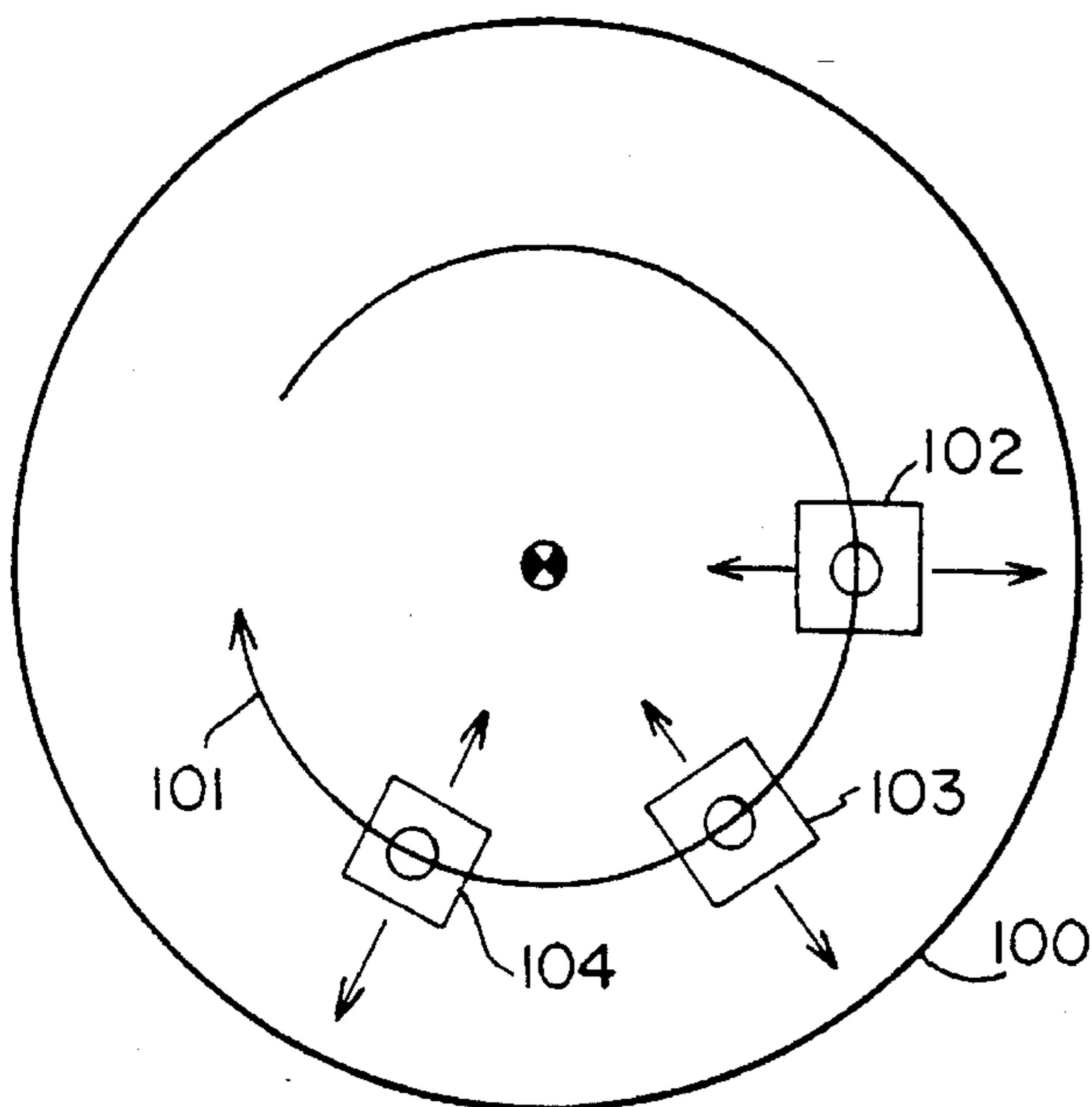
FIG. 5 PRIOR ART
