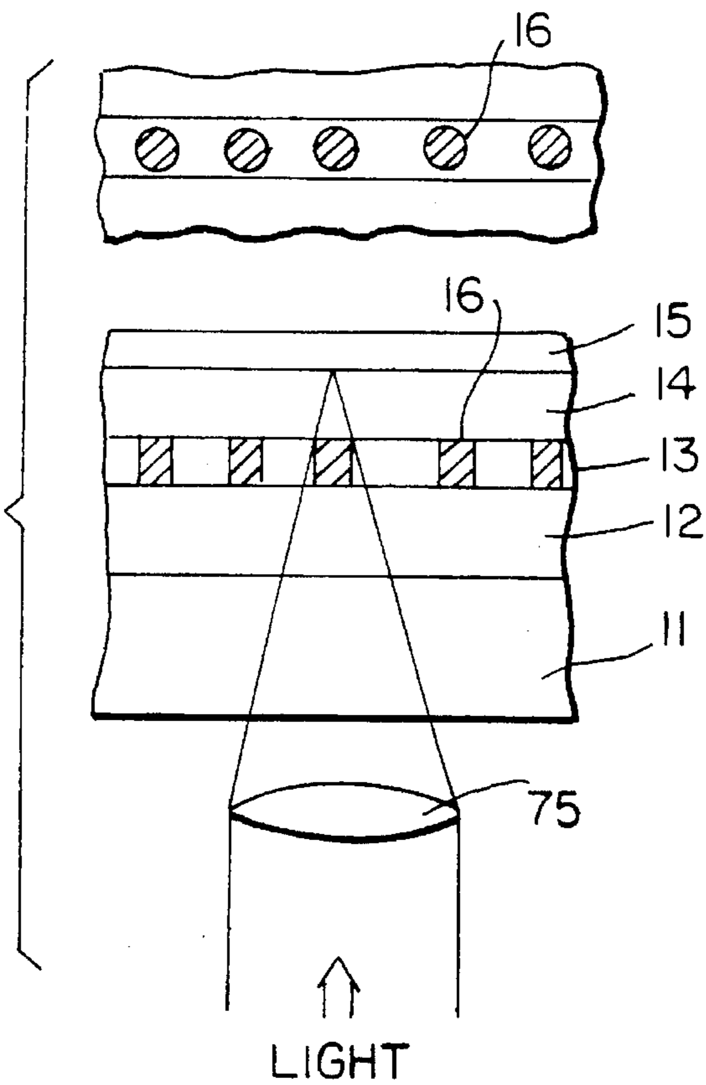
FIG. 1 PRIOR ART
