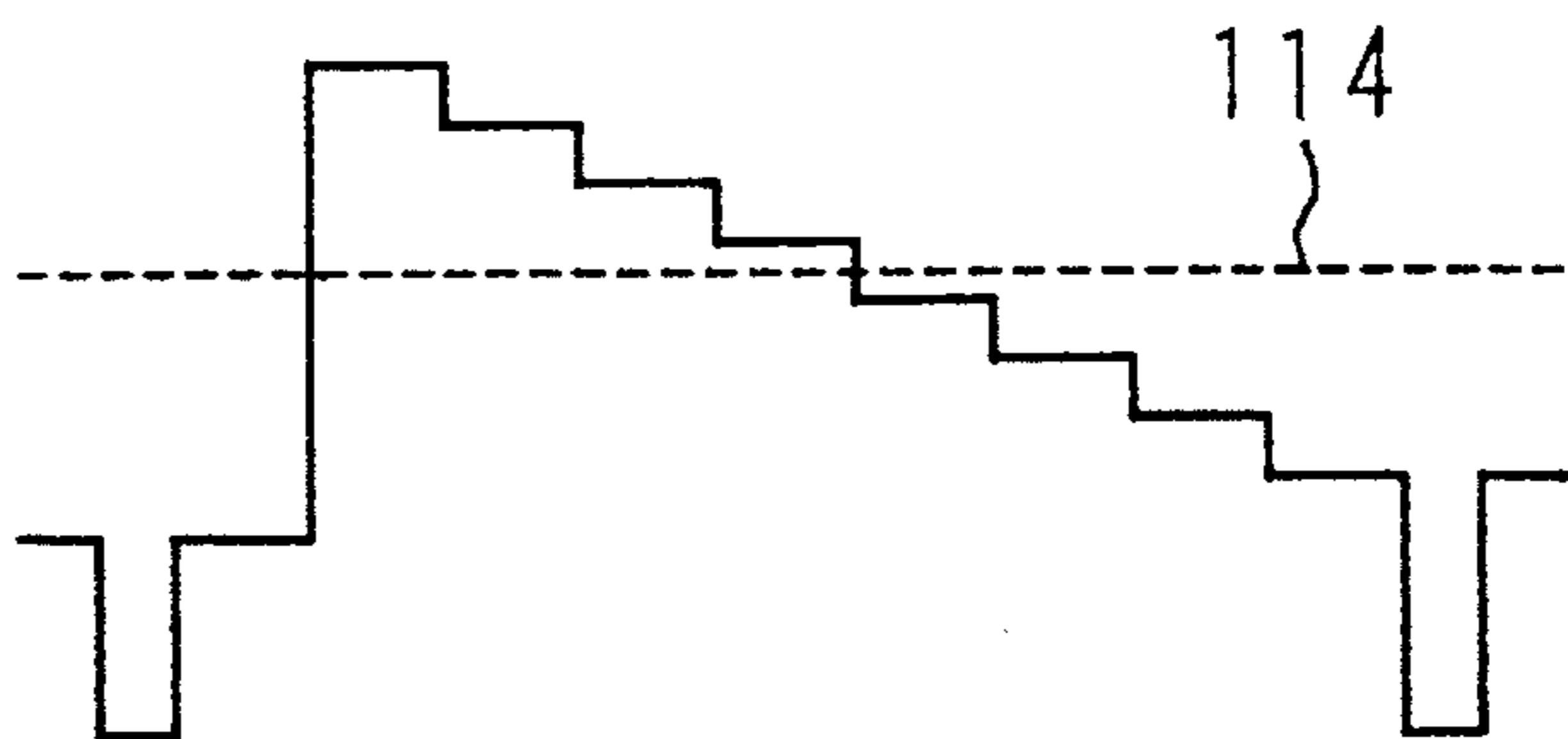
Fig. 29A LUMINANCE SIGNAL Y
