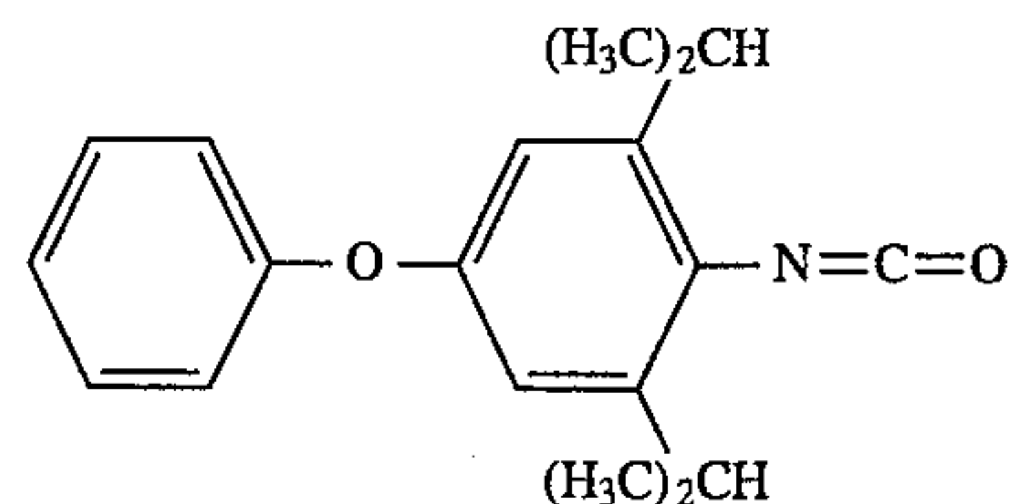
4-phenoxy-2,6-diisopropylphenyl isocyanate
