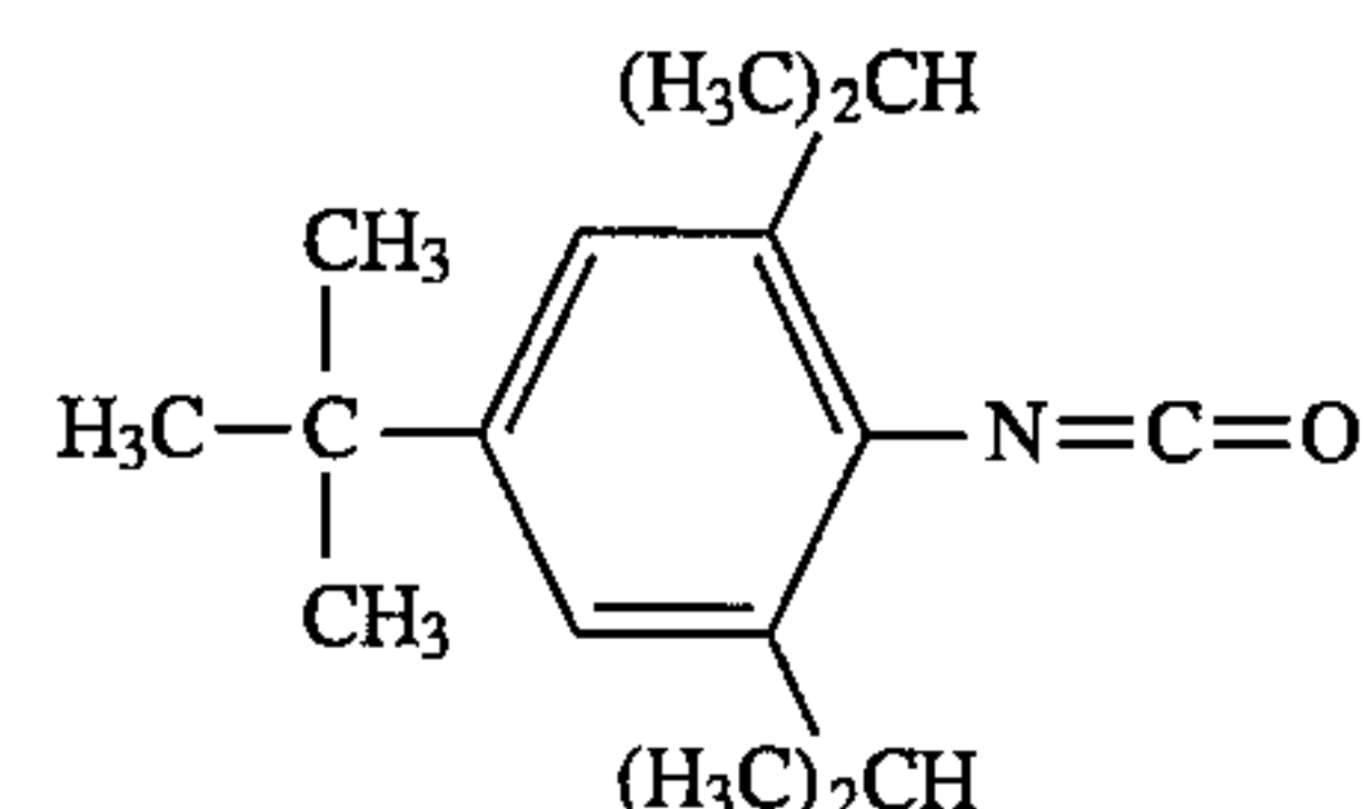
4-tert-butyl-2,6-diisopropylphenyl isocyanate
