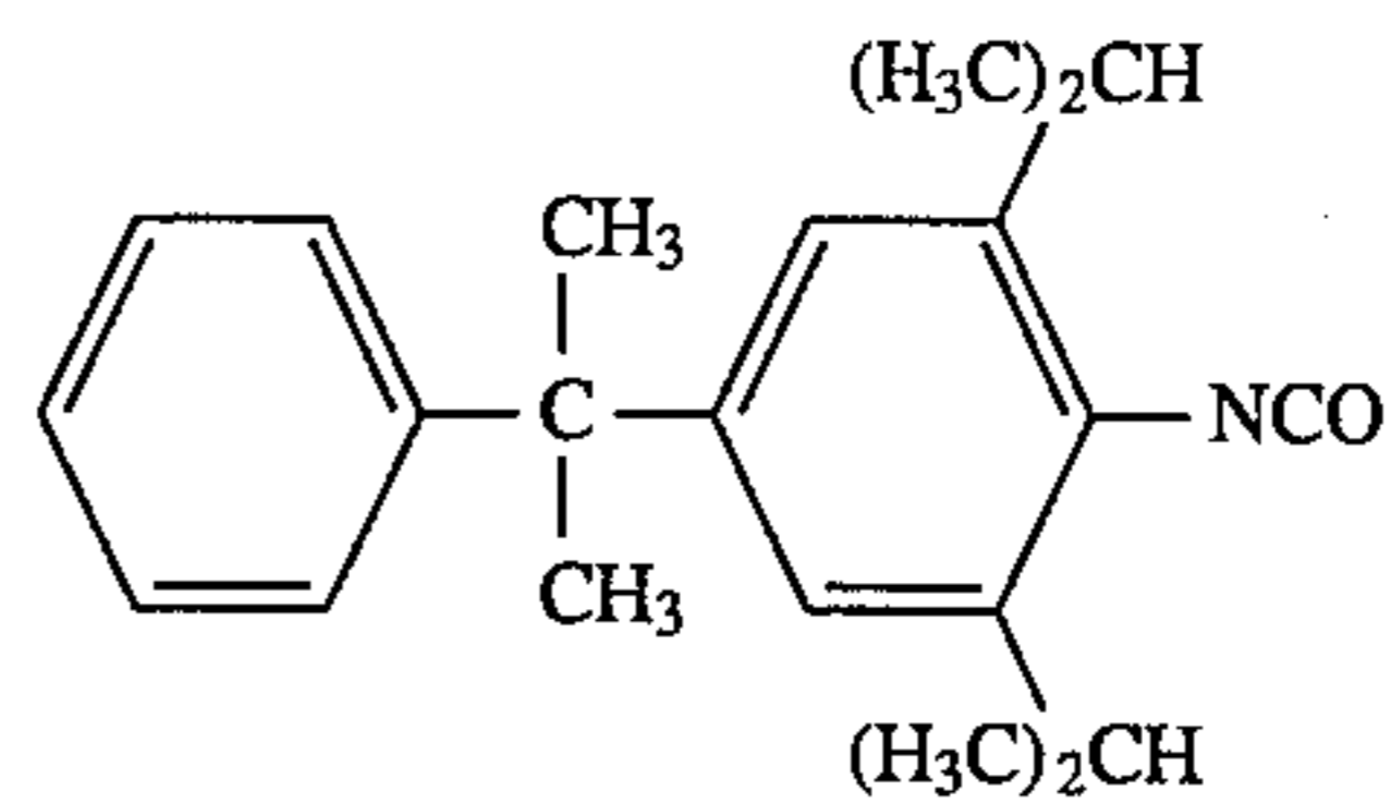
4-(1-methyl-1-phenylethyl)-2,6-diisopropylphenyl isocyanate
