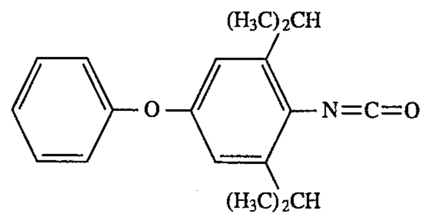
4-phenoxy-2,6-diisopropylphenyl isocyanate
