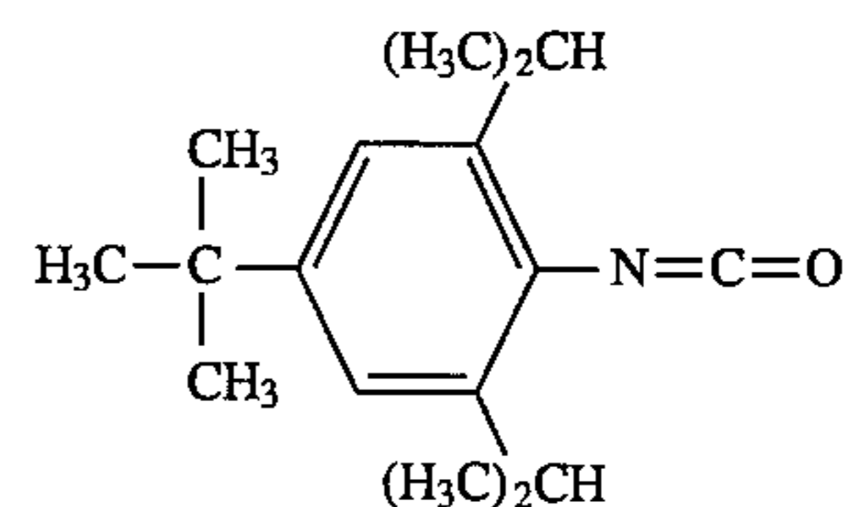
4-tert-butyl-2,6-diisopropylphenyl isocyanate
