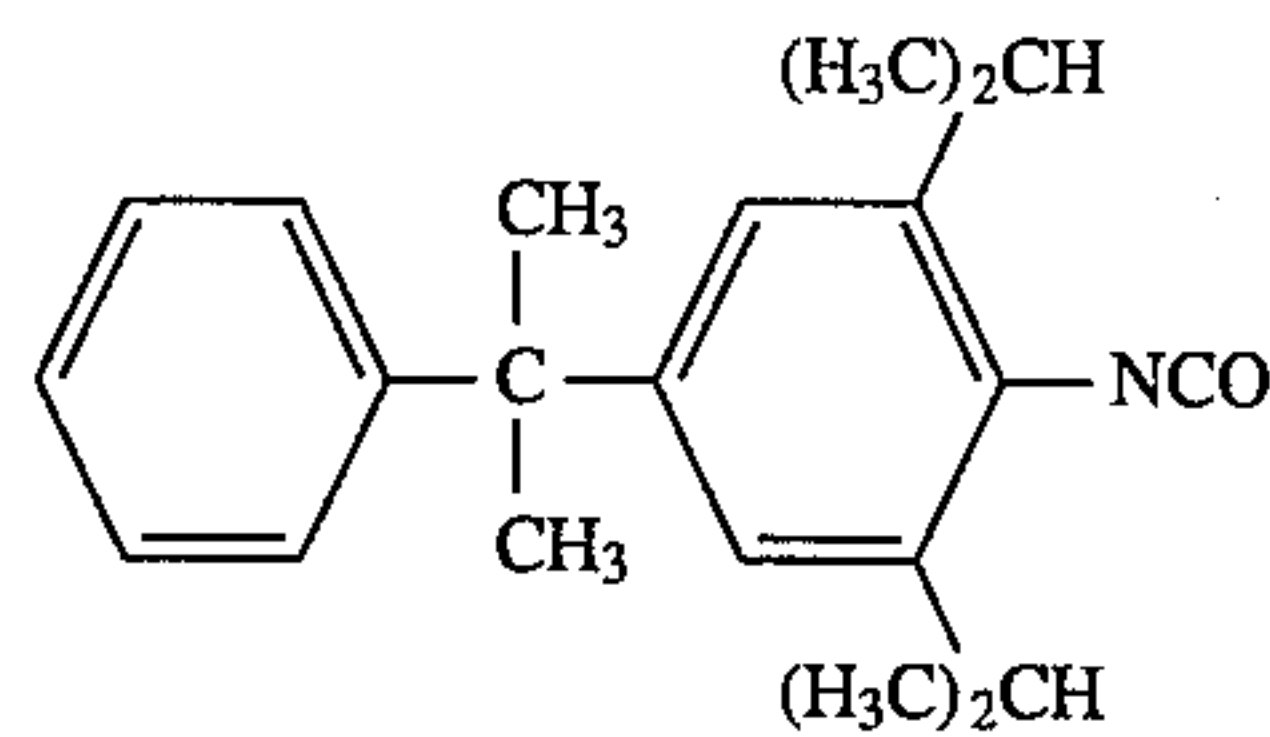
4-(1-methyl-1-phenylethyl)-2,6-diisopropylphenyl isocyanate
