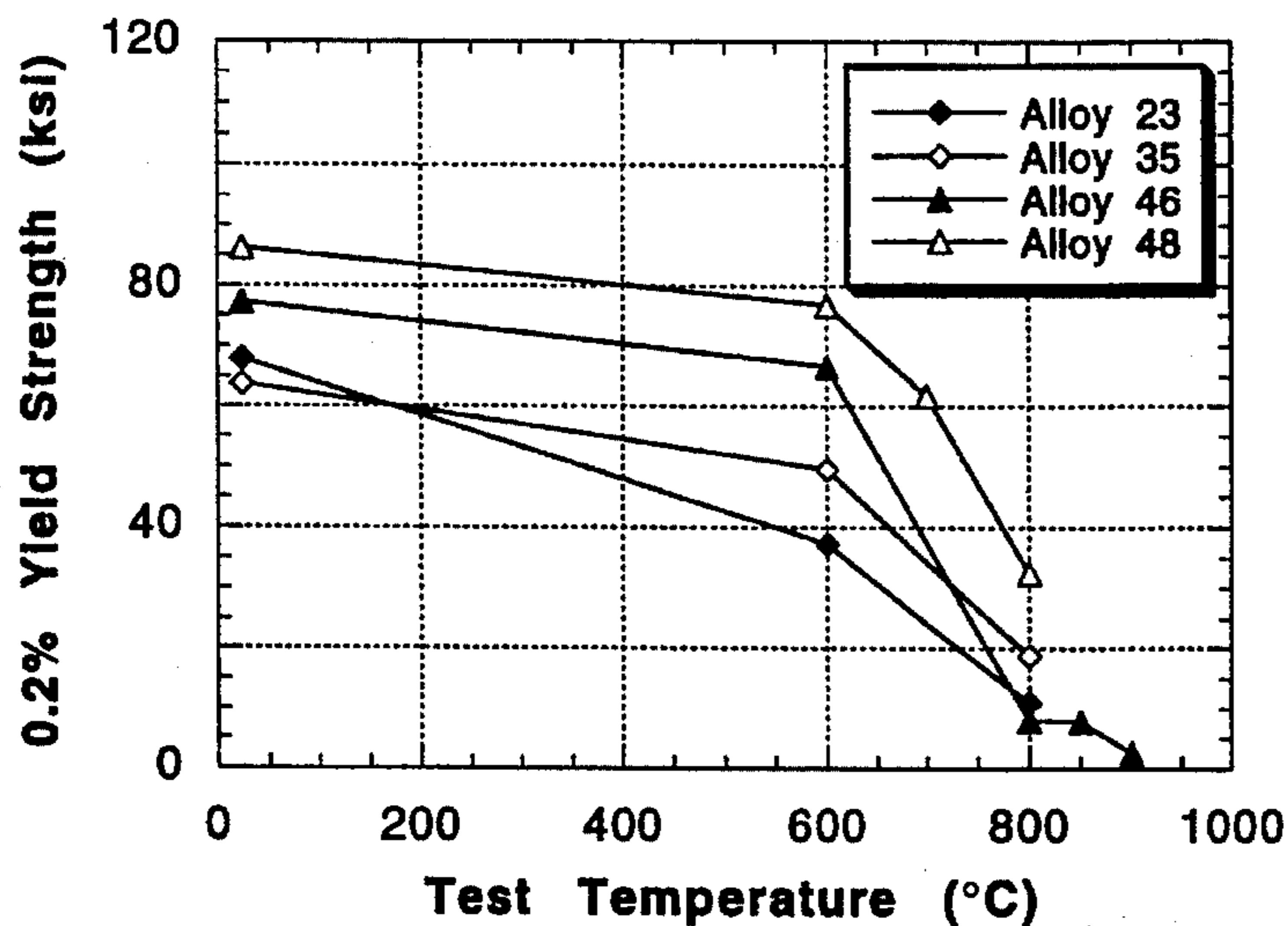
Tensile Data Comparison
