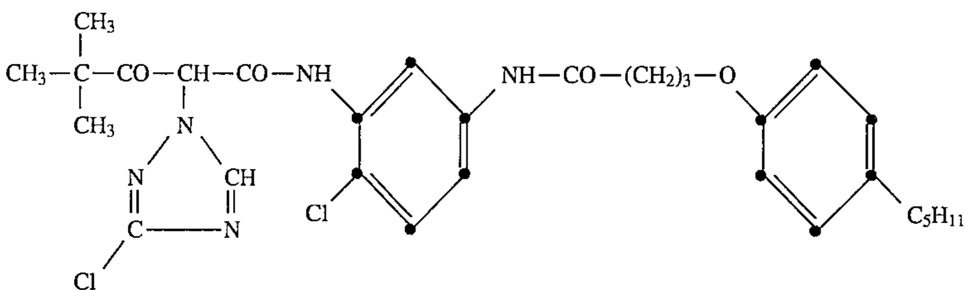
Coupler C:
