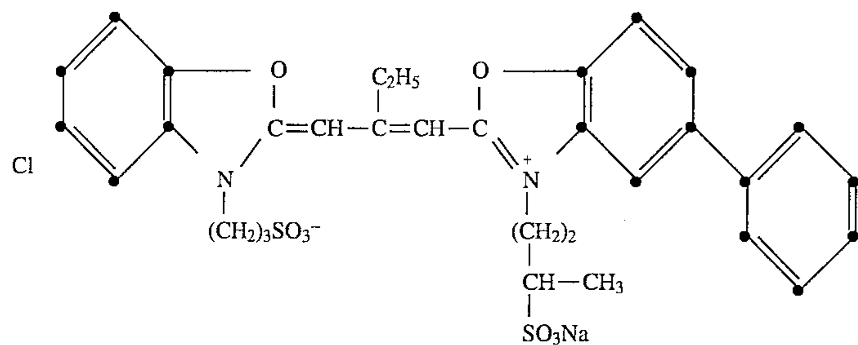
Sensitizing Dye III:
