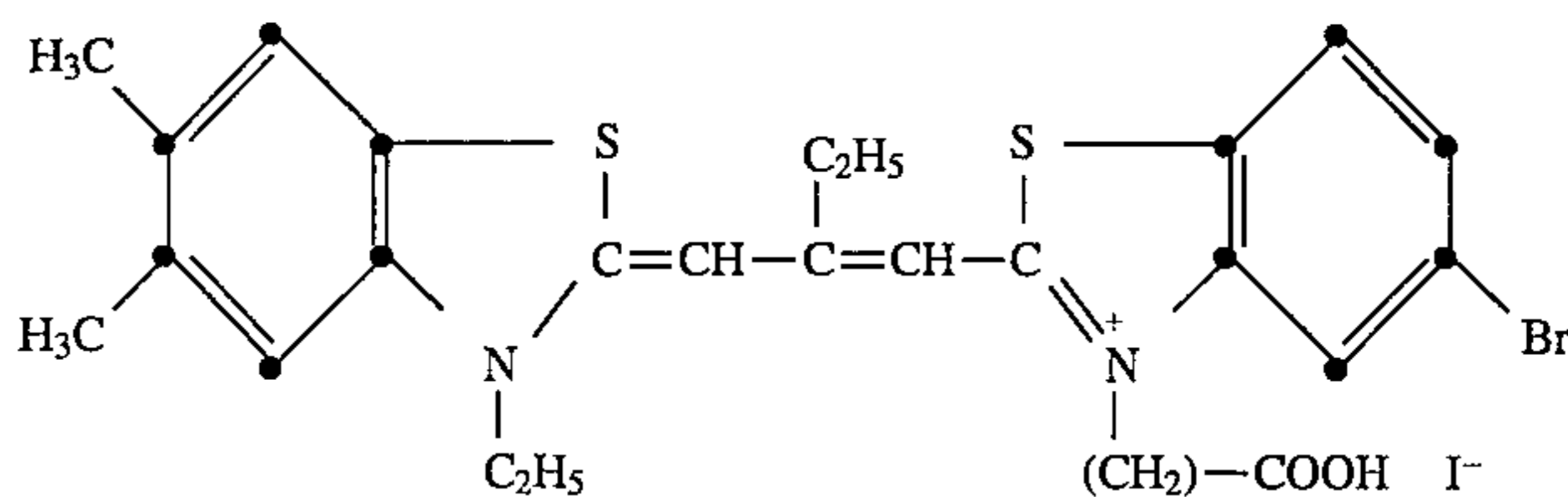
Sensitizing Dye II:
