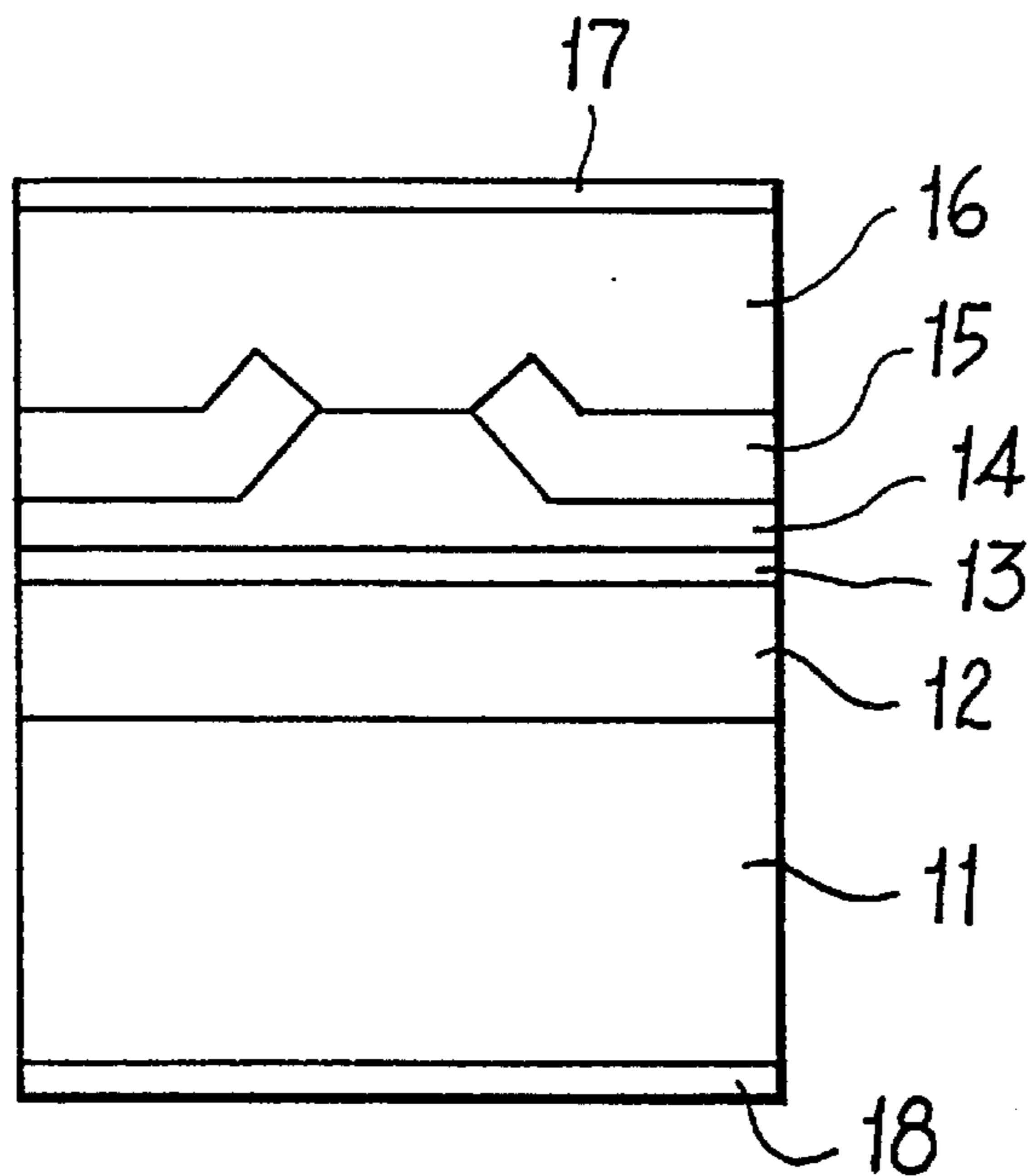
Fig. 2 (Prior Art)
