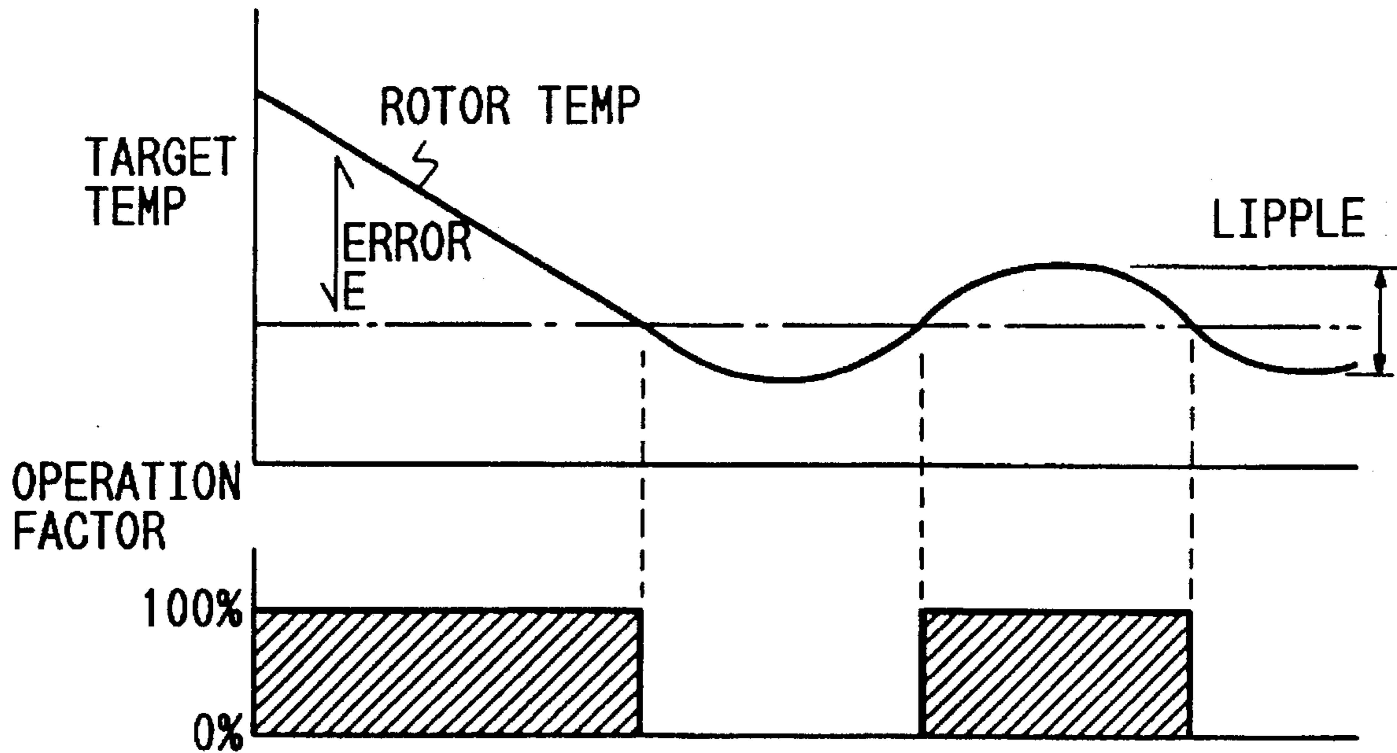
FIG. 9 PRIOR ART
