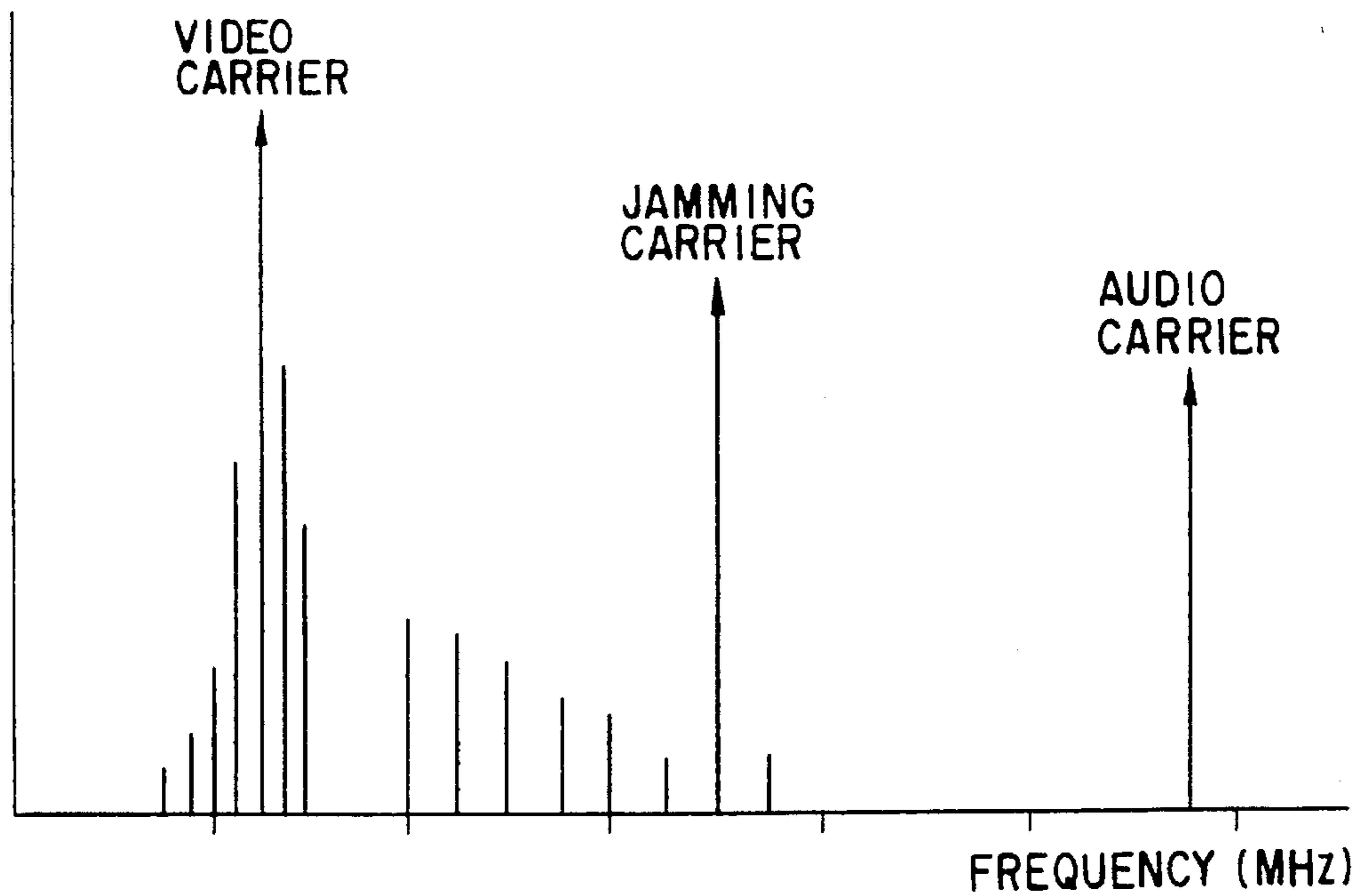
TV CHANNEL CARRIER SPECTRUM INCLUDING JAMMING SIGNAL
