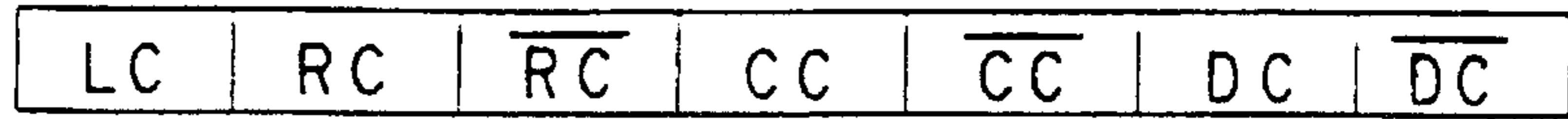
RCU TRANSMISSION FORMAT (RF)
