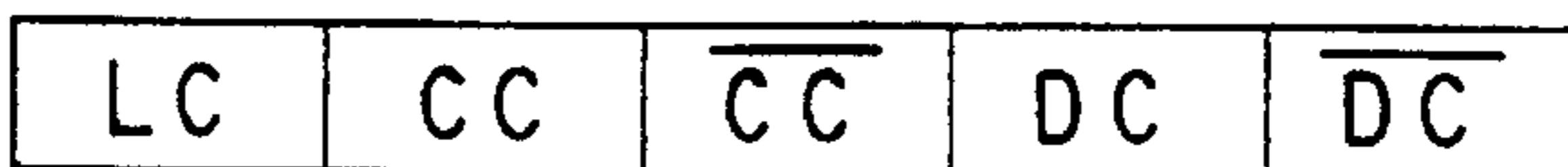
RCU INFRARED FORMAT (IR)
