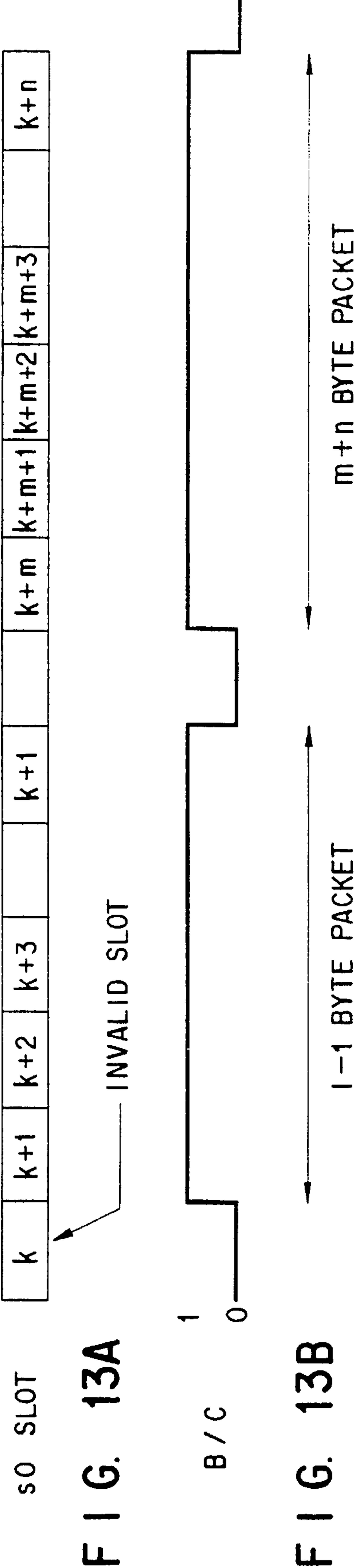
CONTROL PACKET EFFECTIVE SLOT IDENTIFICATION EXTRACTION OF CONTROL SLOT & DATA SLOT
