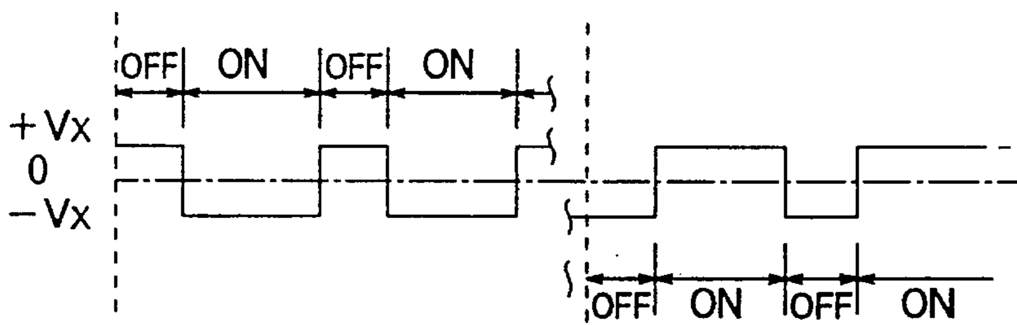
DATA SIGNAL WAVEFORM
