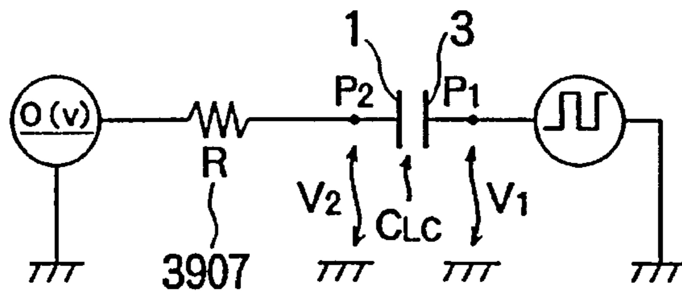
FIG. 39 (b) (PRIOR ART)
