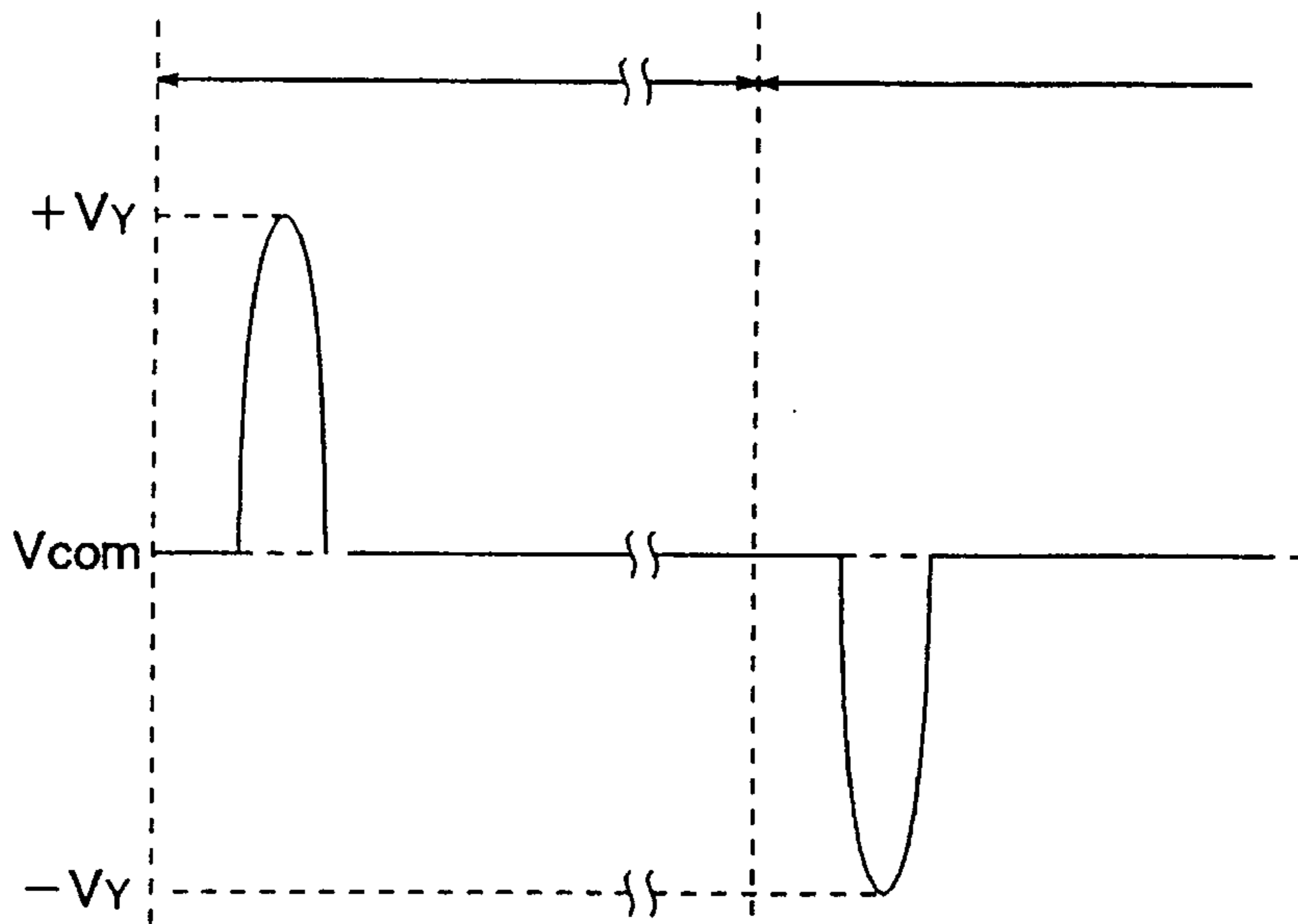
SCANNING SIGNAL POTENTIAL CONTROL TERMINAL
