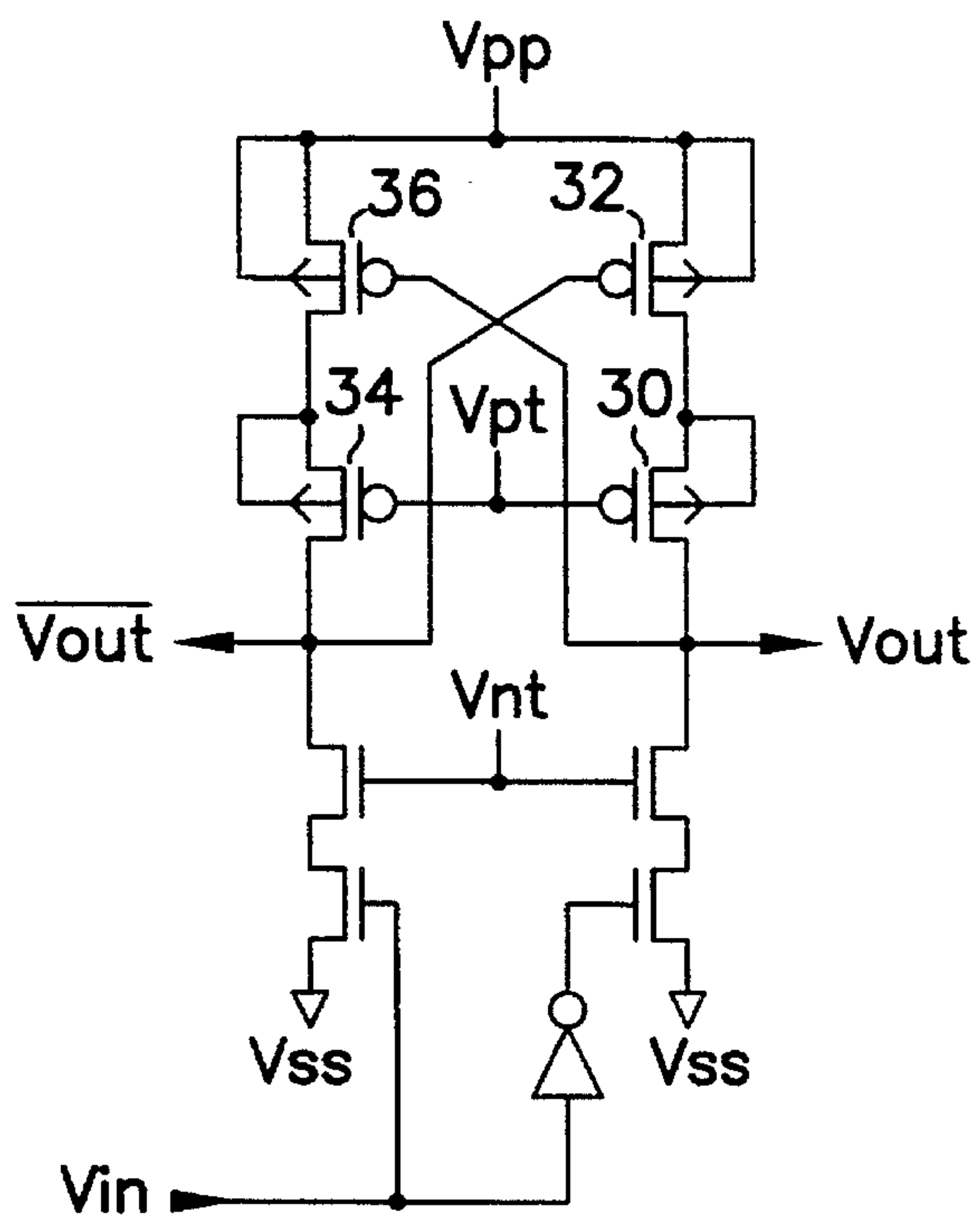
FIG. 2 (PRIOR ART)
