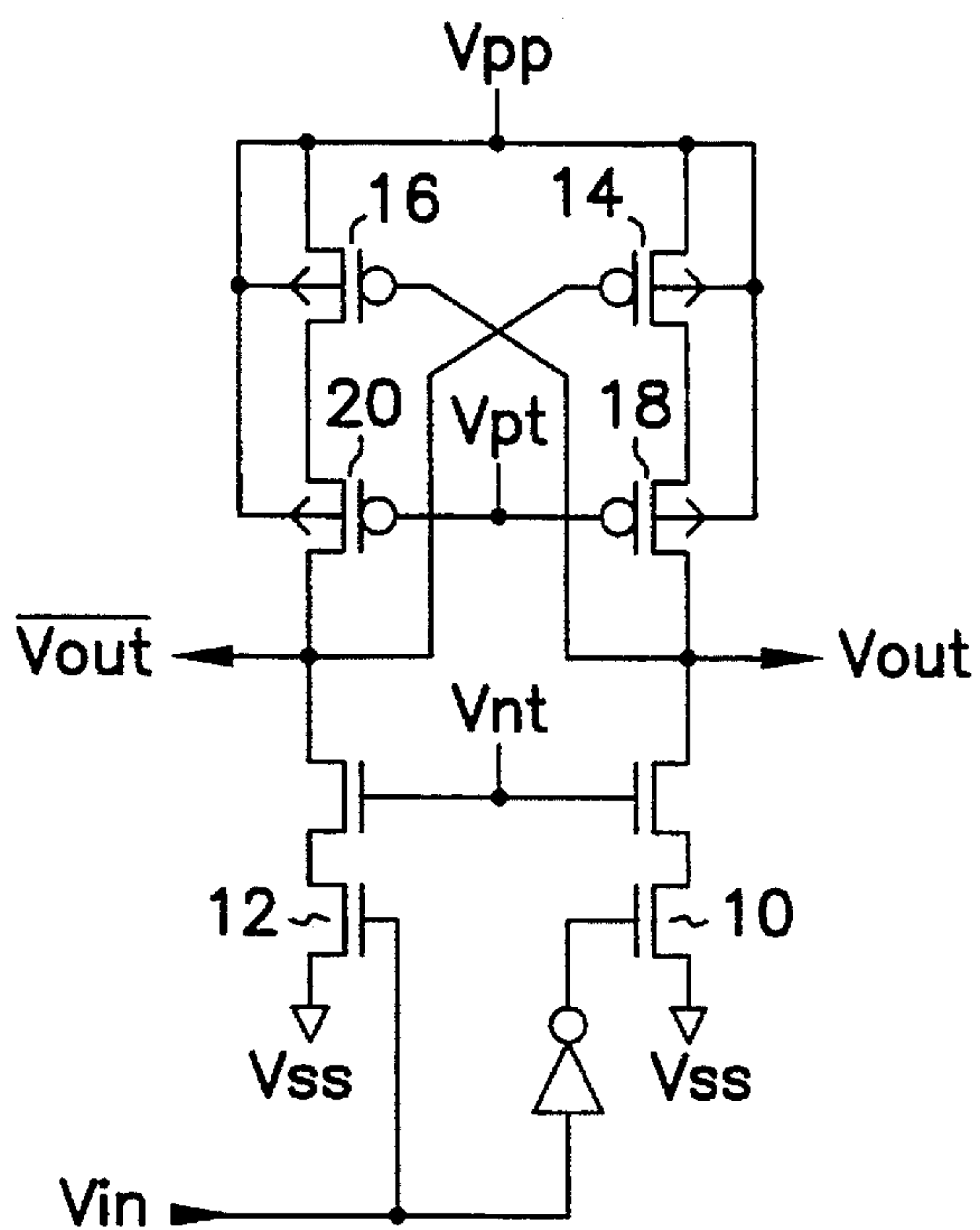
FIG. 1 (PRIOR ART)
