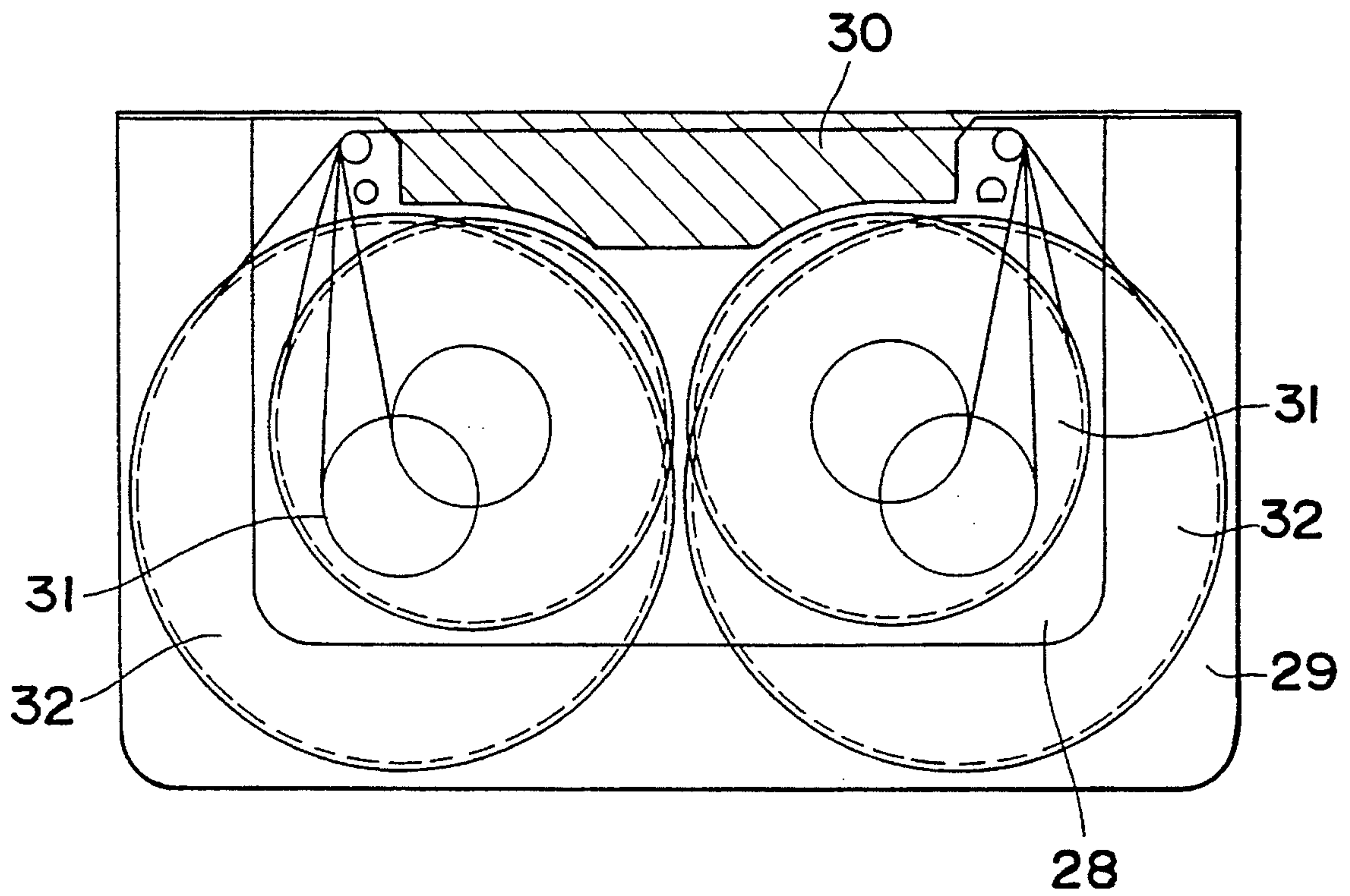
Fig. 7 PRIOR ART
