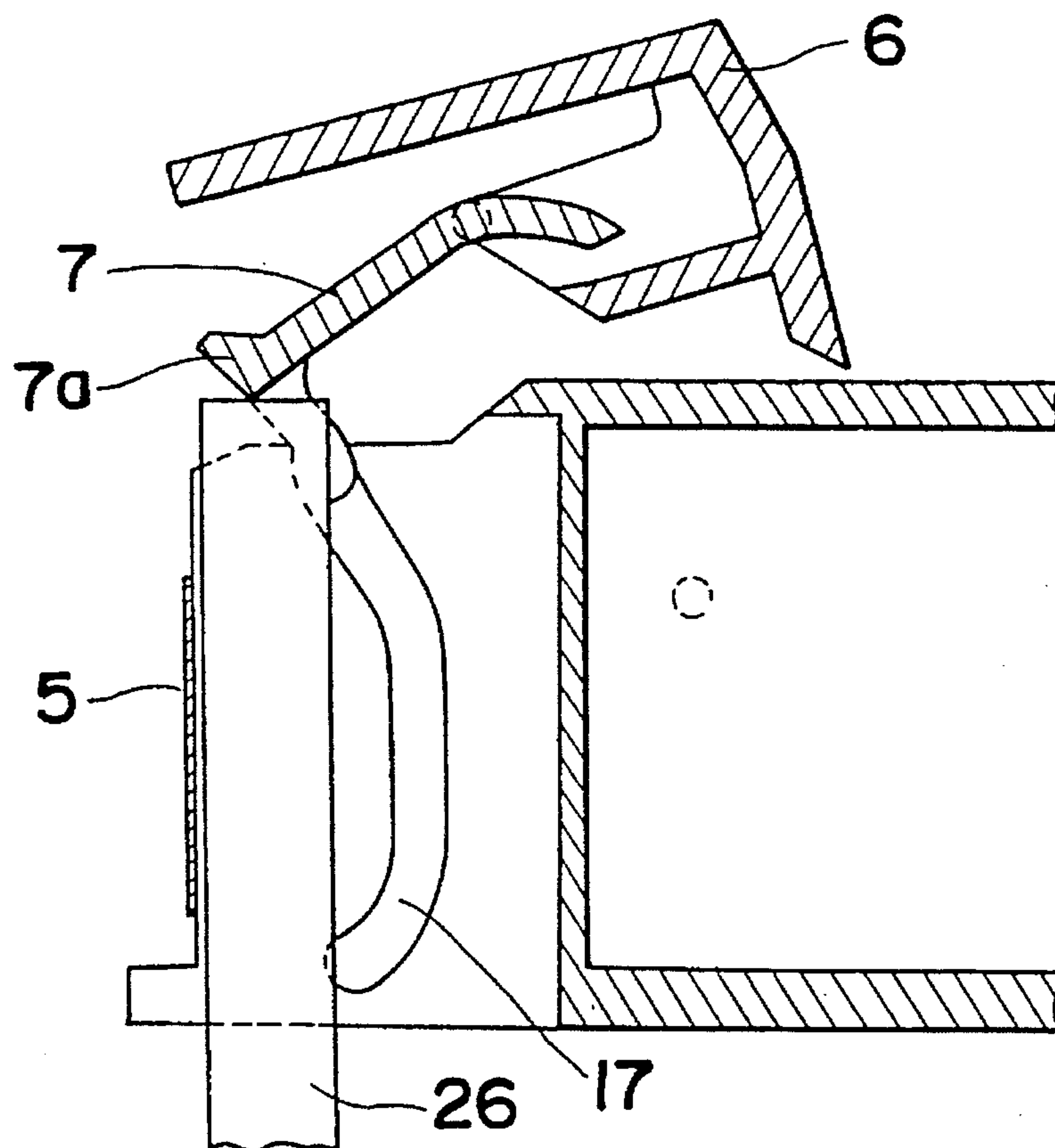
Fig. 6 PRIOR ART
