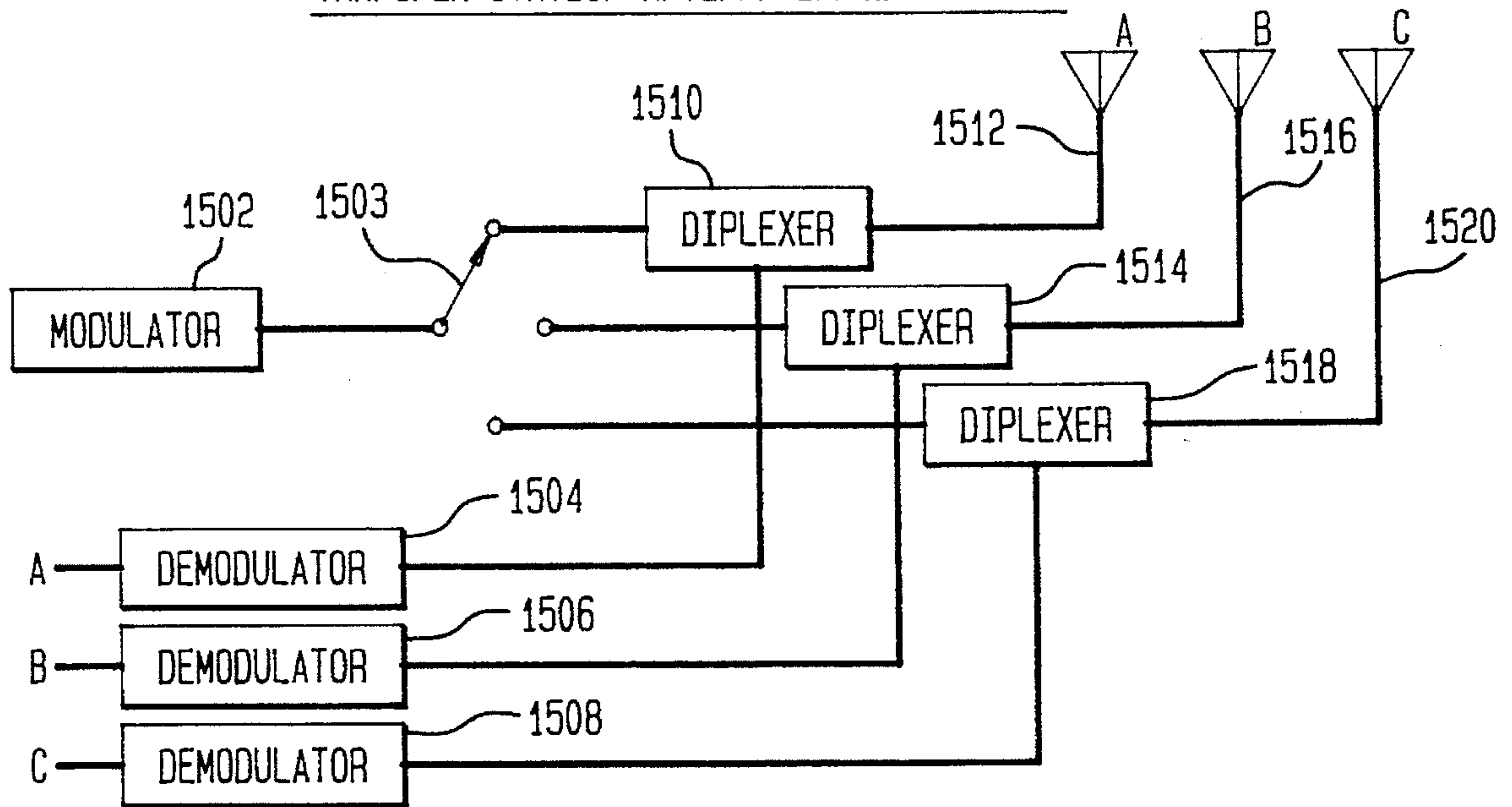
TRANSFER STATION ANTENNA IMPLEMENTATION
