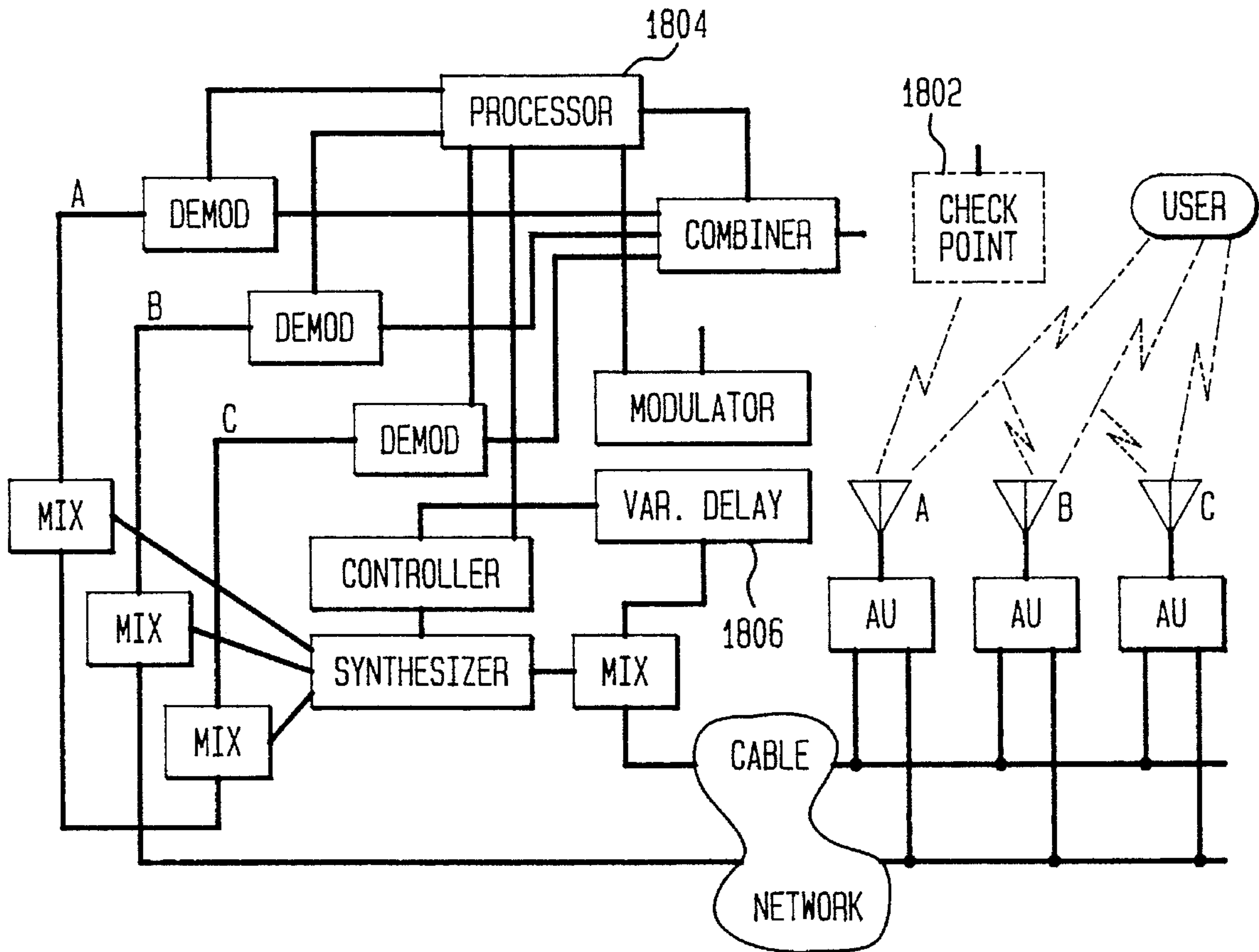
TIME CALIBRATION FOR DISTRIBUTED ANTENNA IMPLEMENTATION
