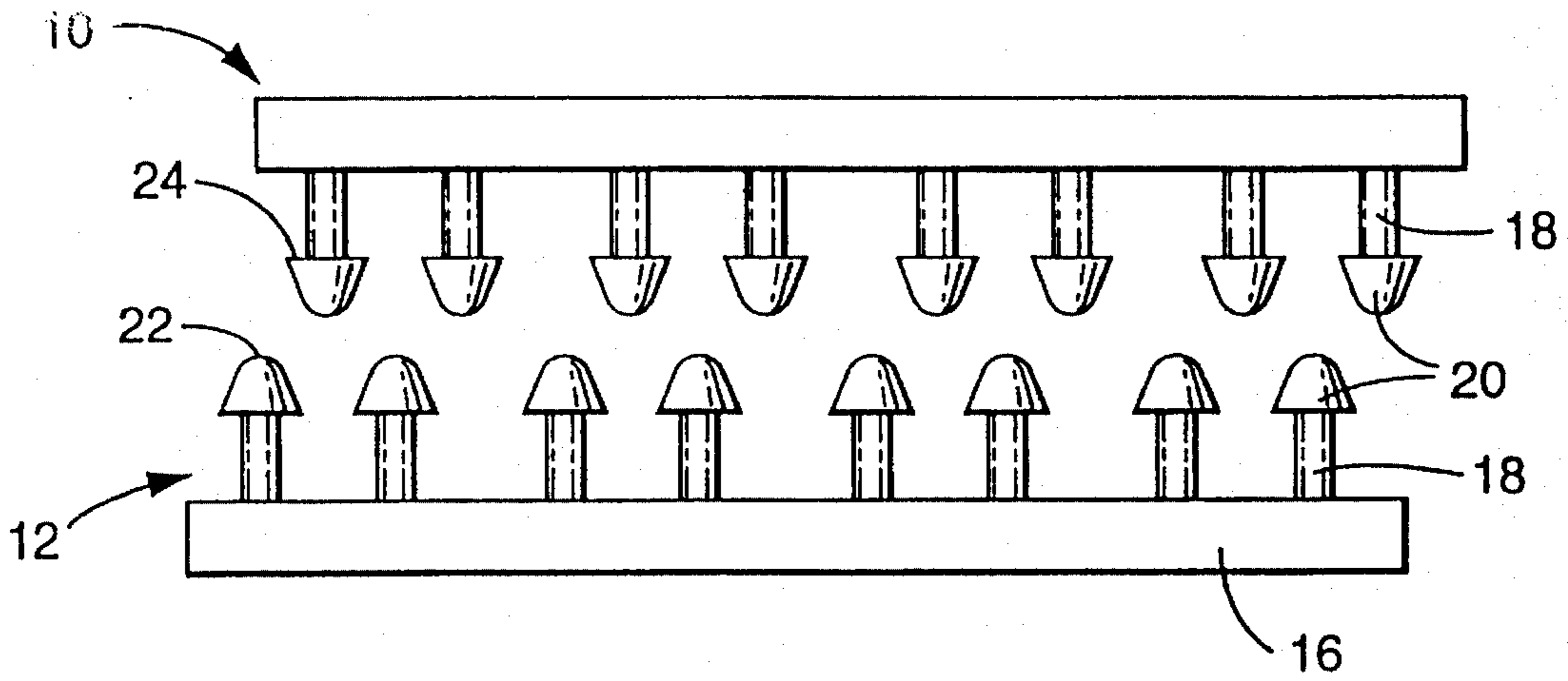
Fig. 1 PRIOR ART
