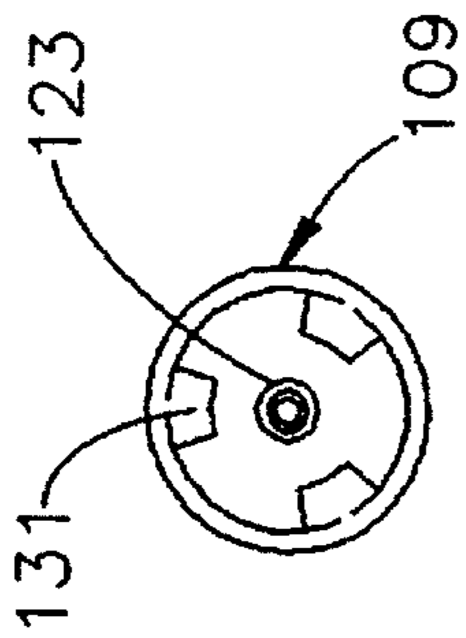
SECT. 32-32
