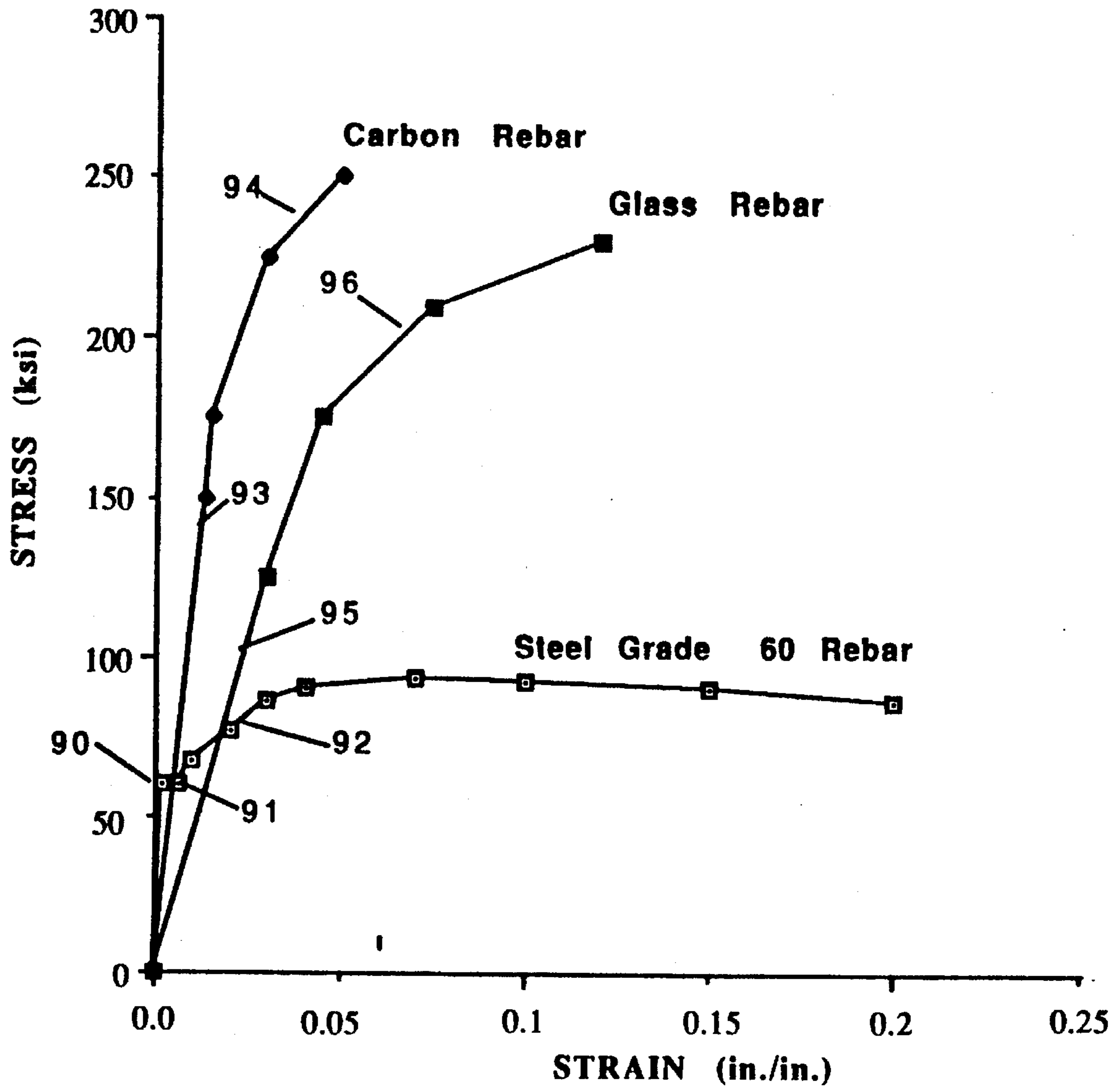
Fig. 7 Stress - Strain Curve
