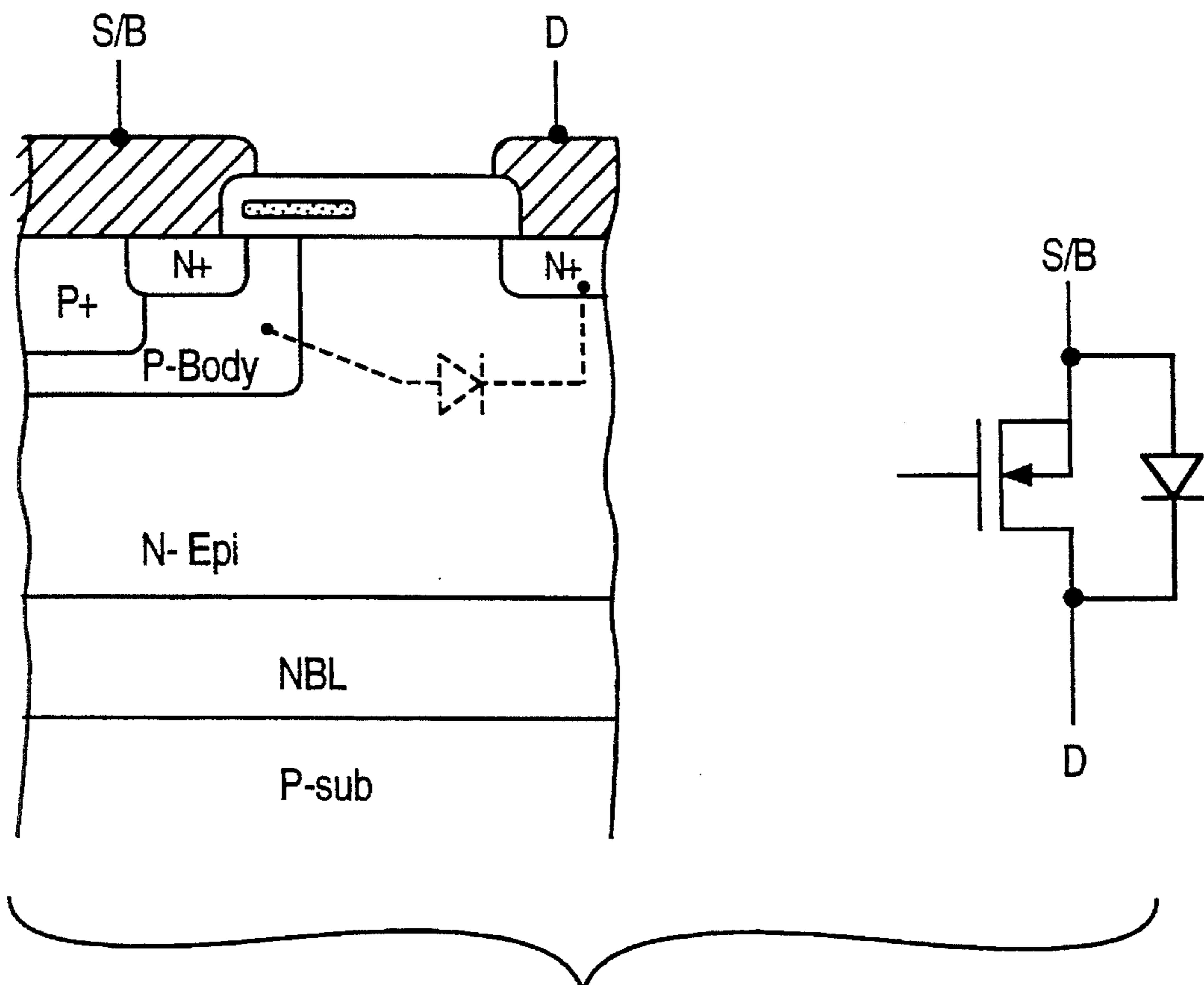
FIG. 5D Prior Art
