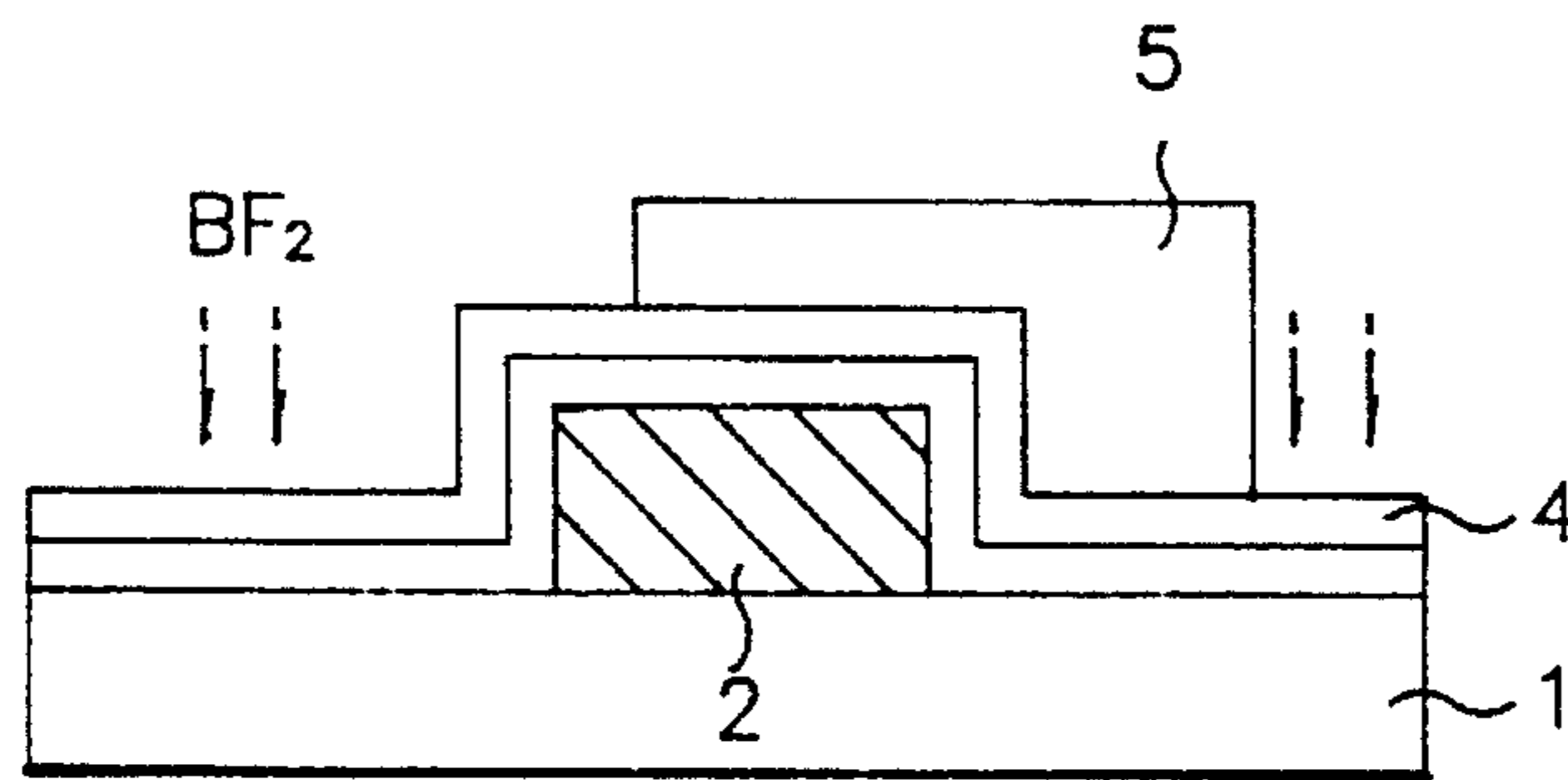
FIG. 1c PRIOR ART
