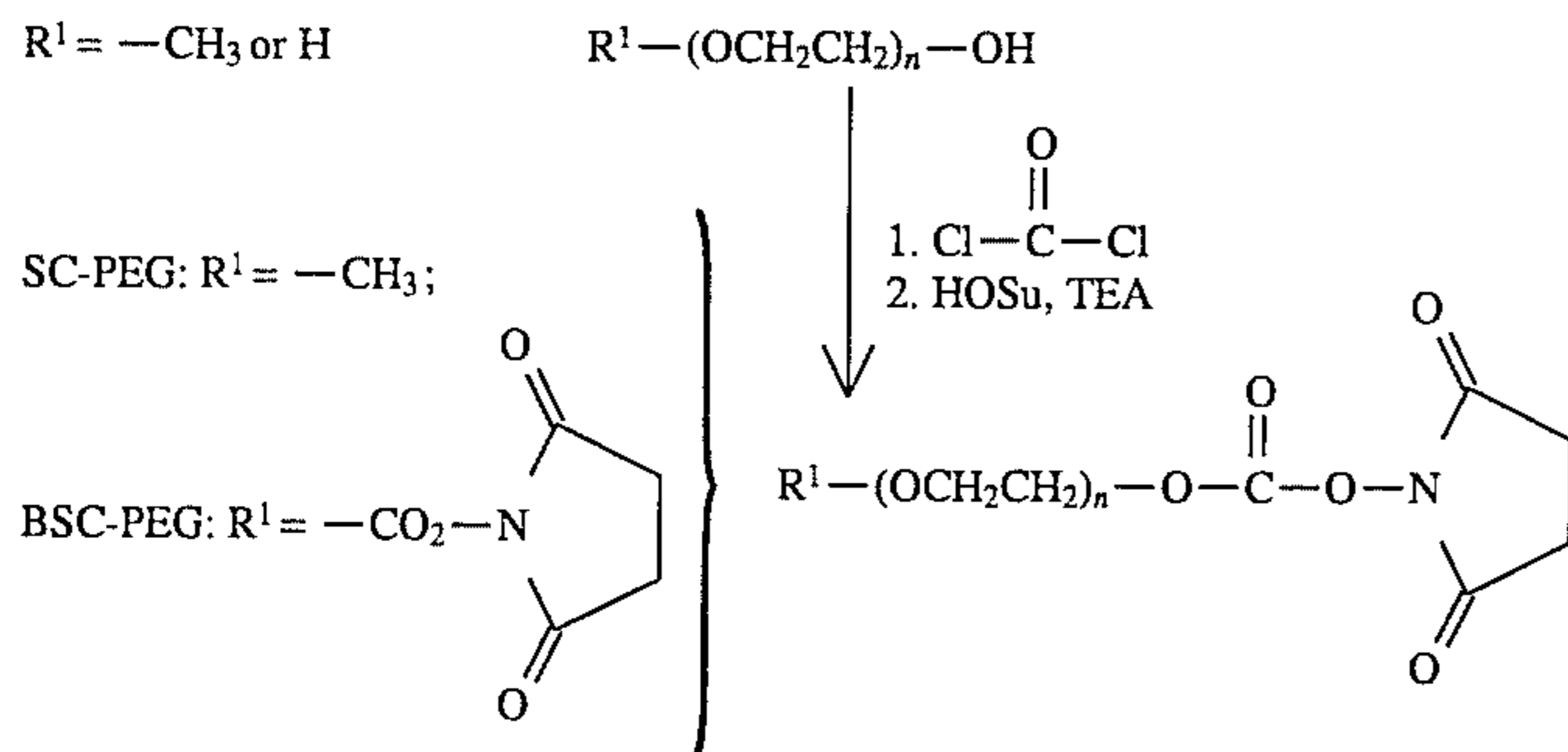
Scheme 3: Synthesis of N-succinimide carbonate derivatives of poly(ethylene glycol).
