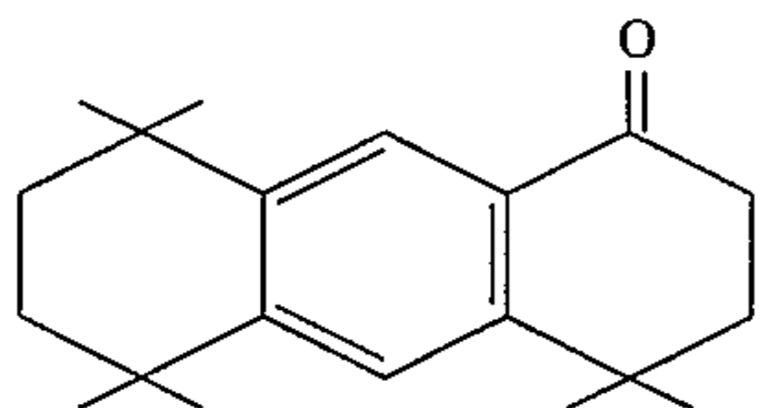
3,4,5,6,7,8-Hexahydro-4,4,5,5,8,8-hexamethyl-1(2H)anthracenone
