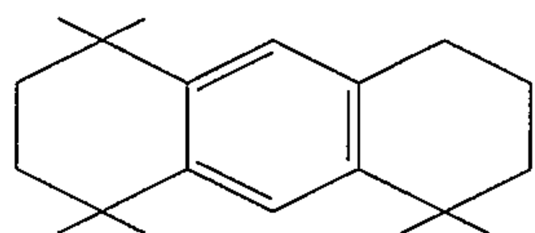
1,2,3,4,5,6,7,8-Octahydro-1,1,4,4,5,5-hexamethylanthracene
