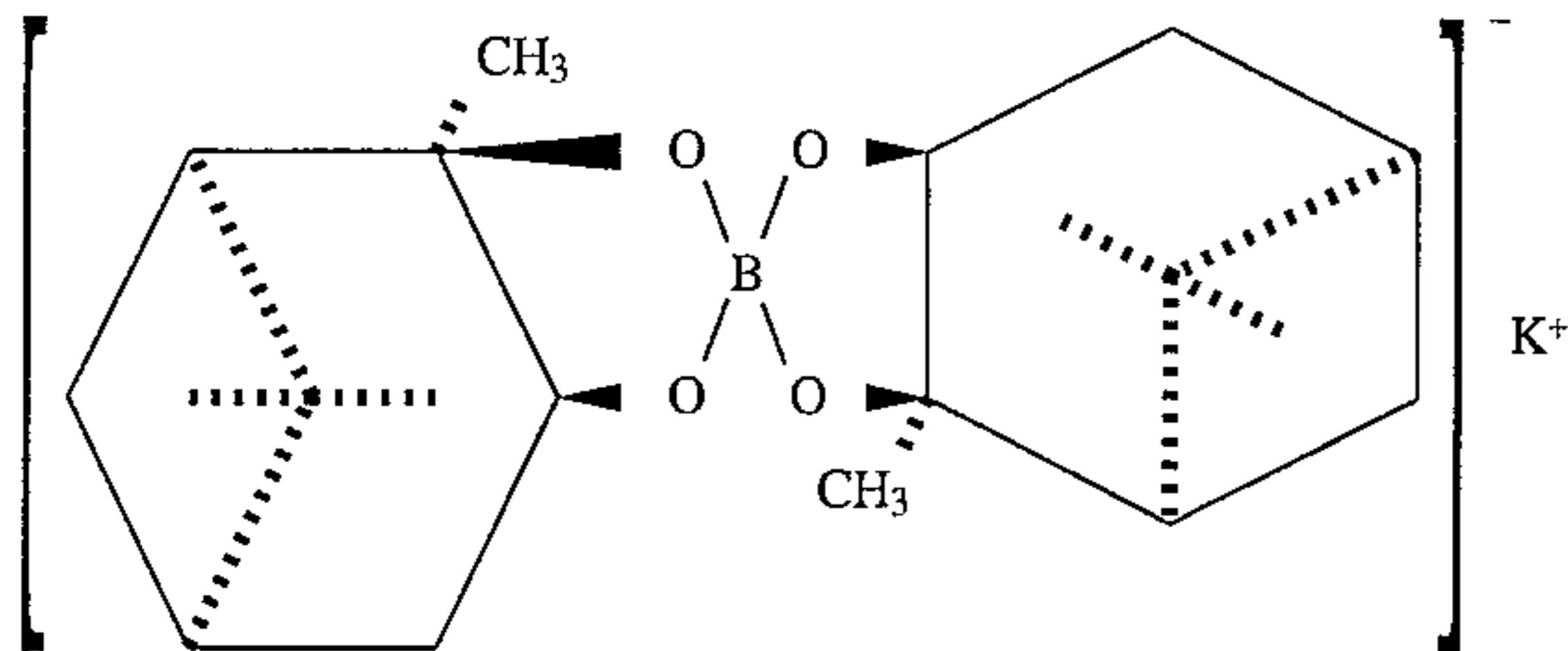
dipinaneboron, the form in which pinanediol is released from reaction 10
