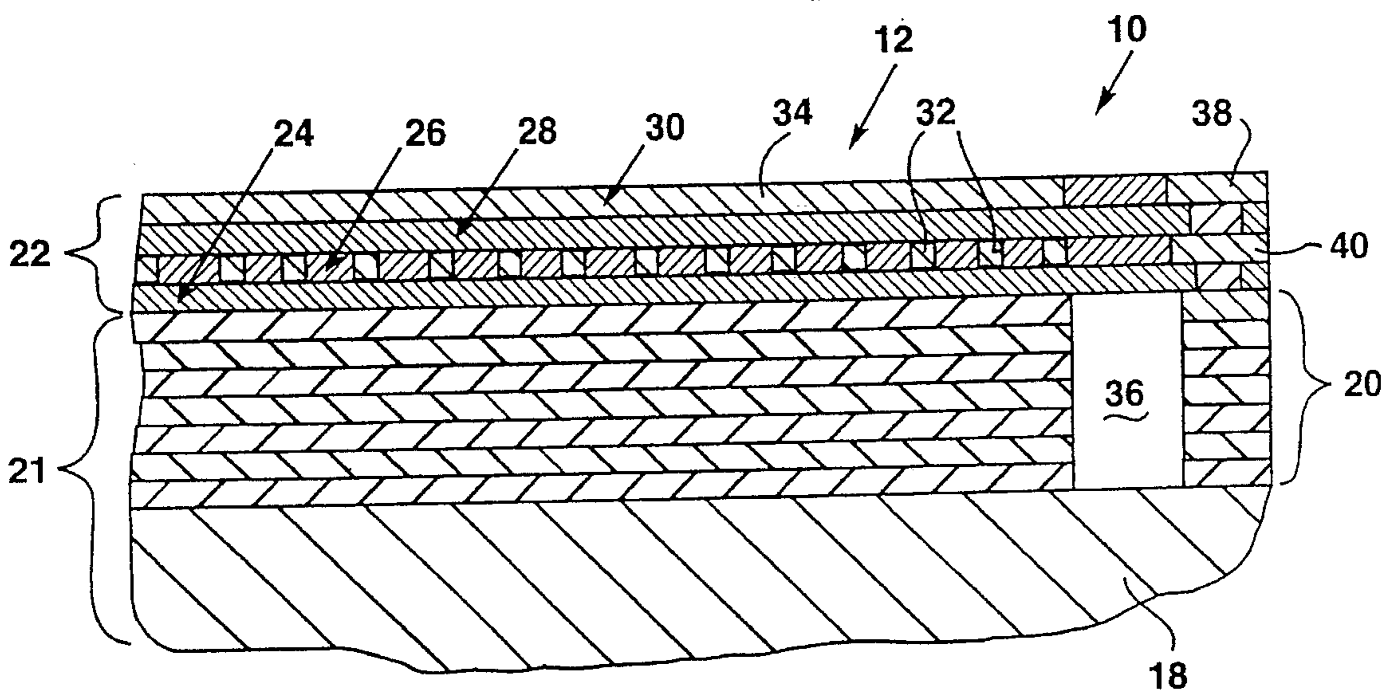
FIG. 2 (PRIOR ART)
