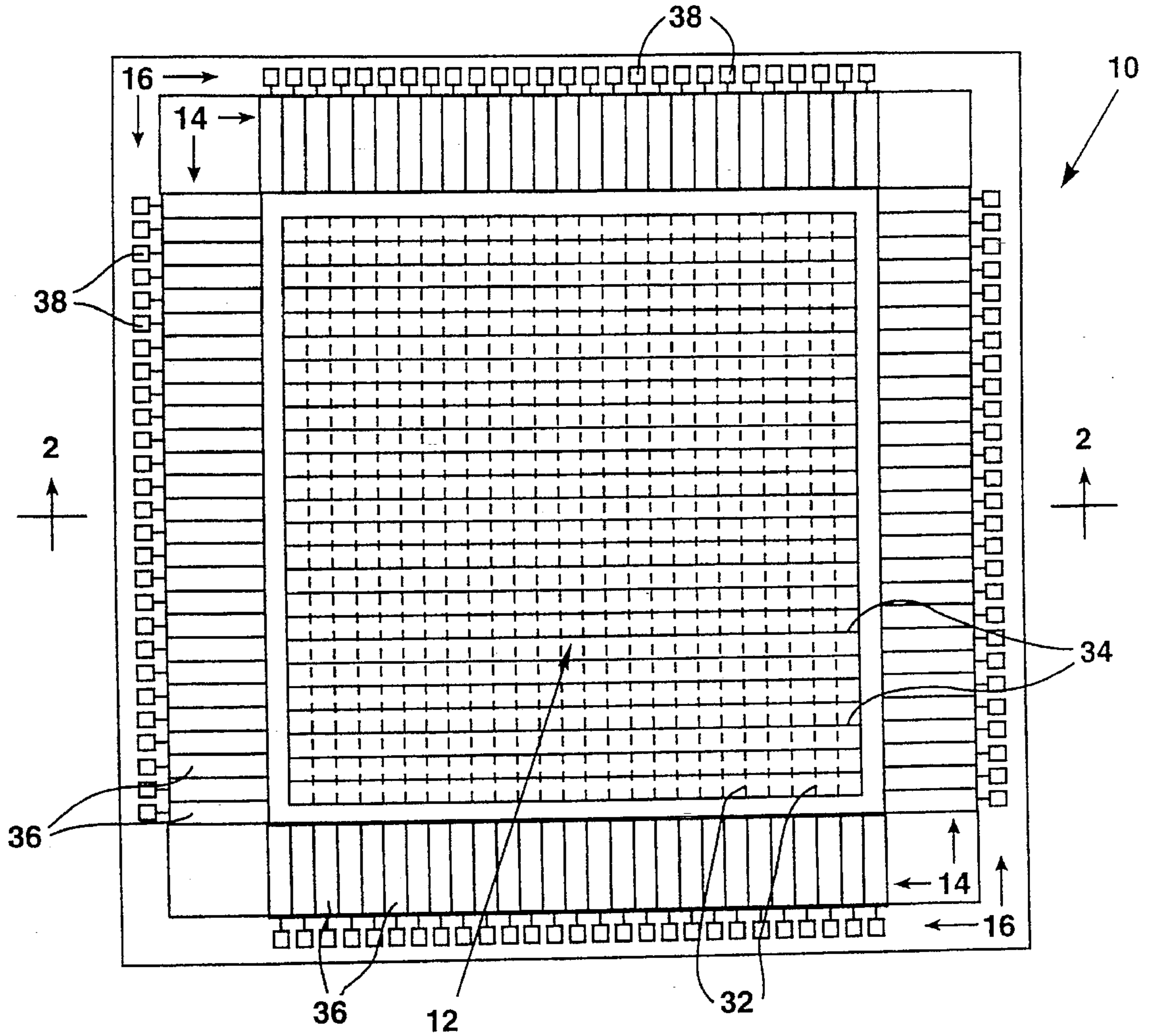
FIG. 1 (PRIOR ART)
