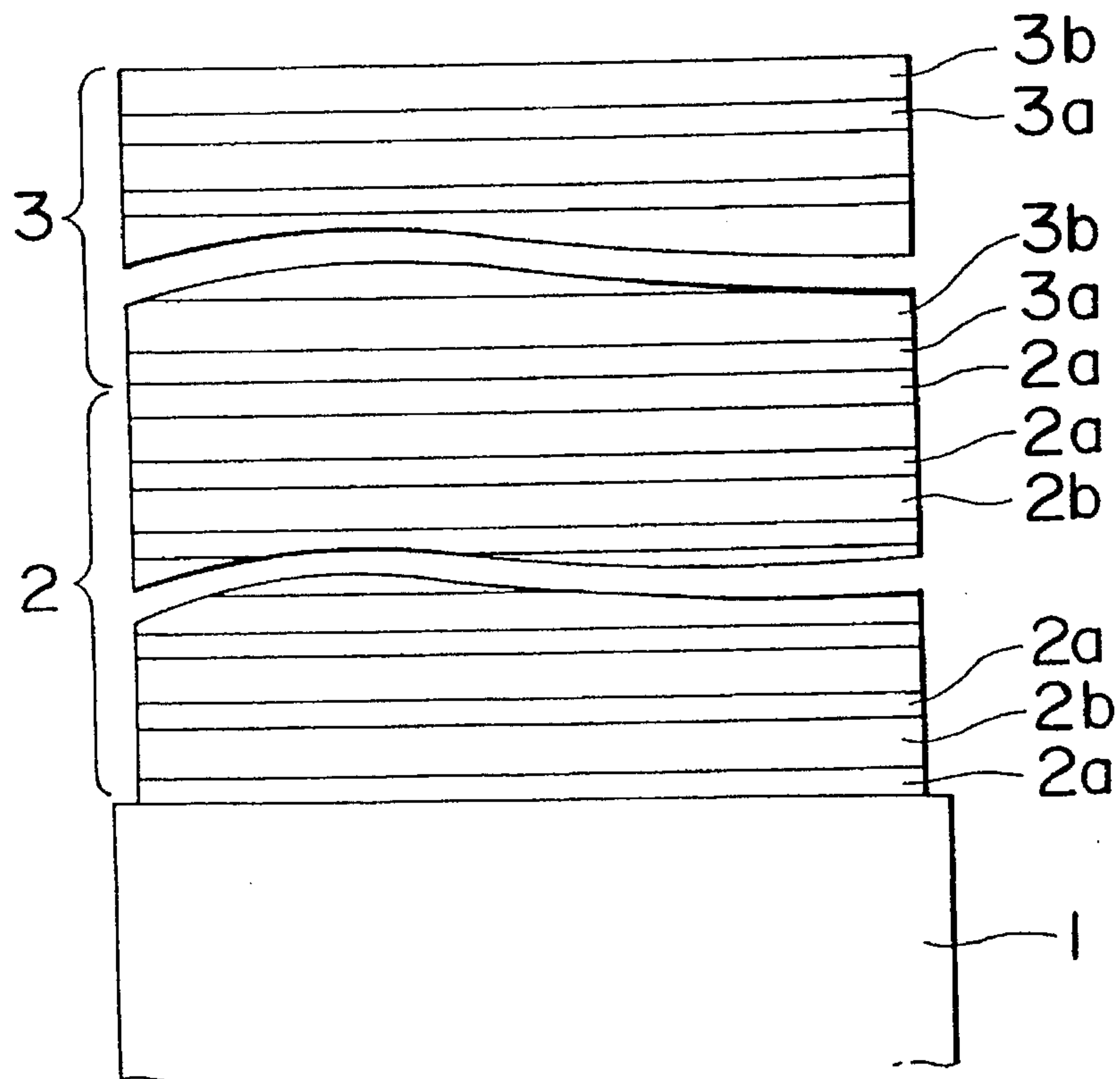
FIG. 4 PRIOR ART
