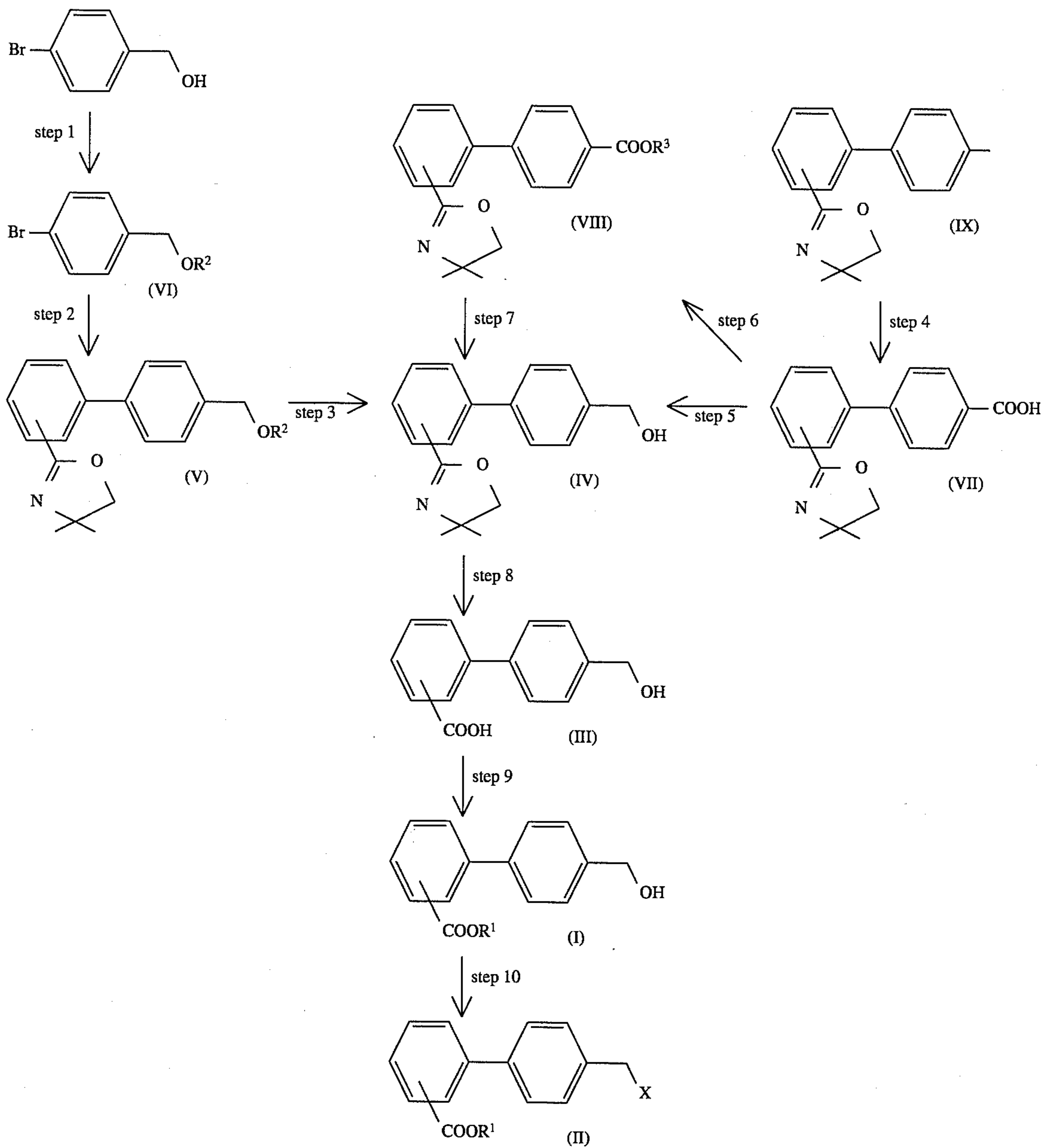
Reaction Scheme-8
