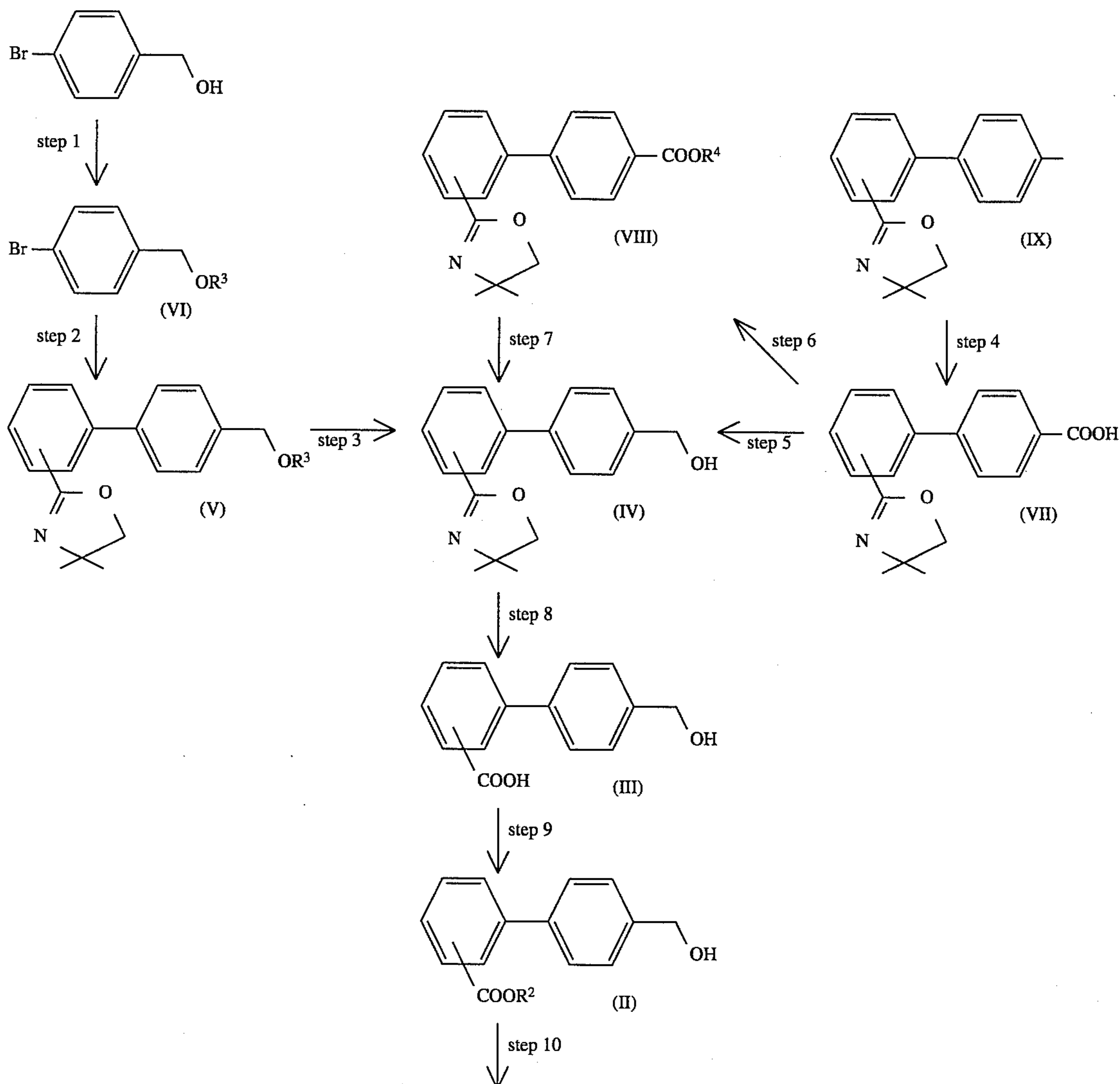
Reaction Scheme-7
