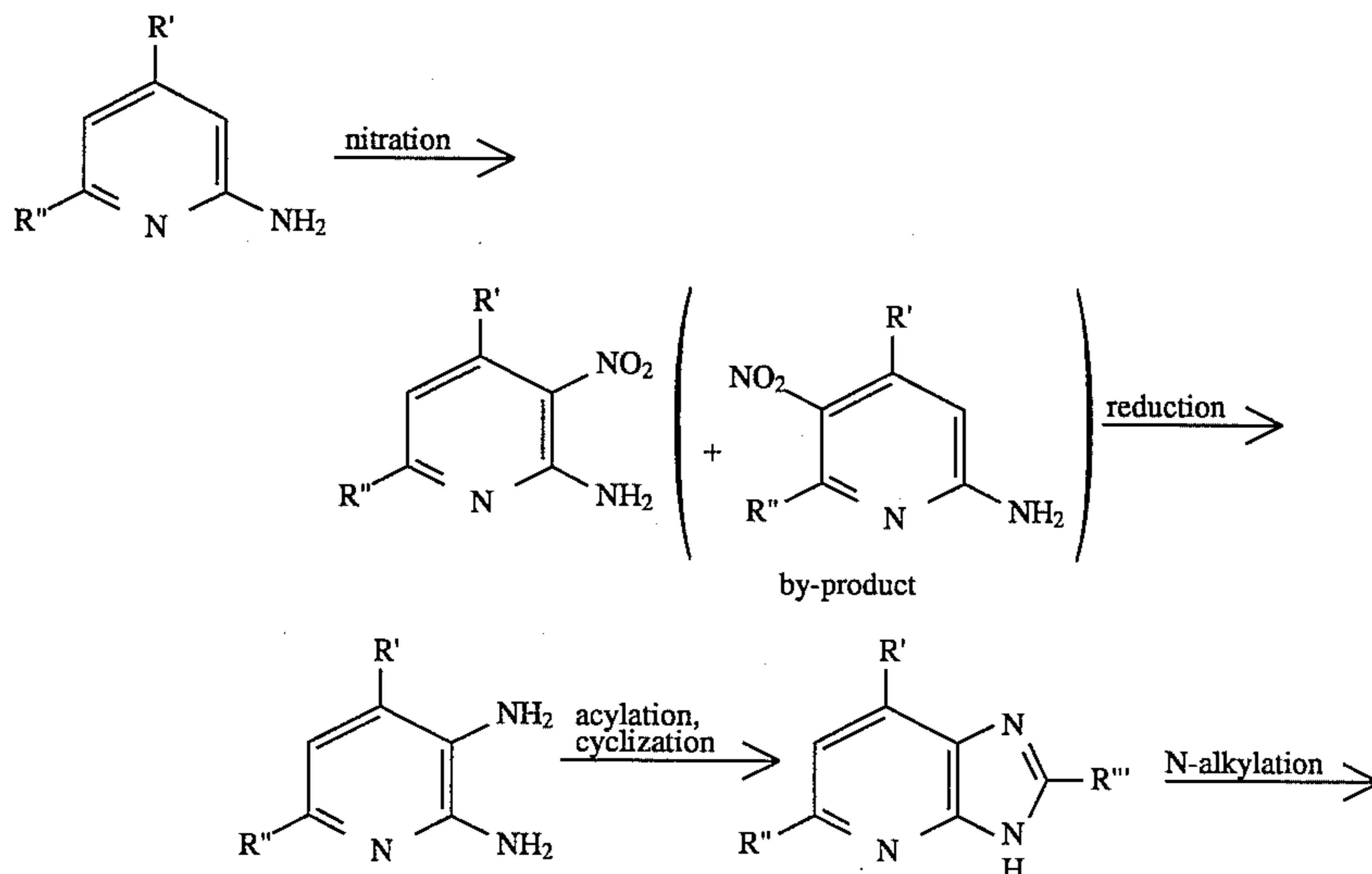
Reaction Scheme-1
