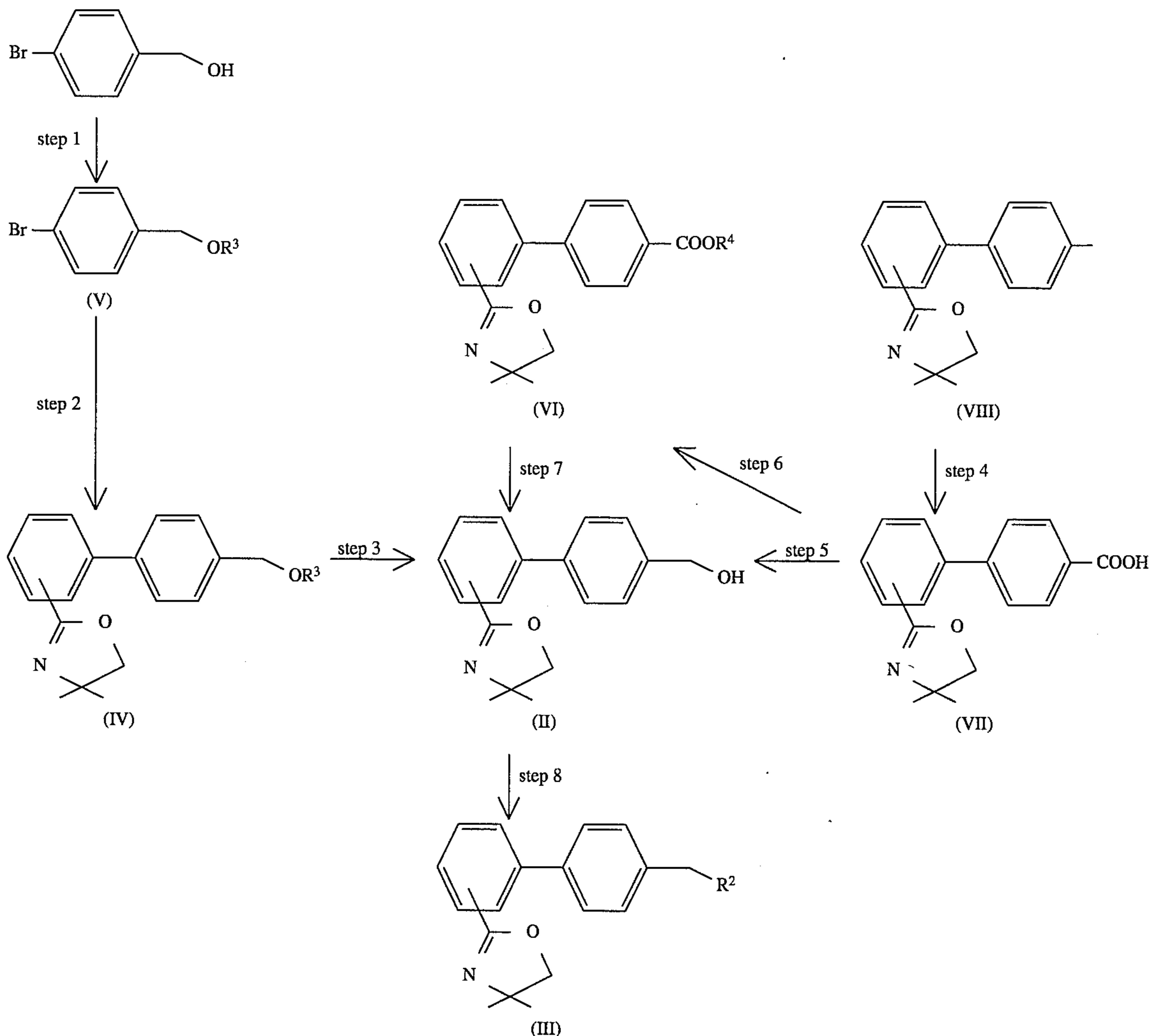
Reaction Scheme-6
