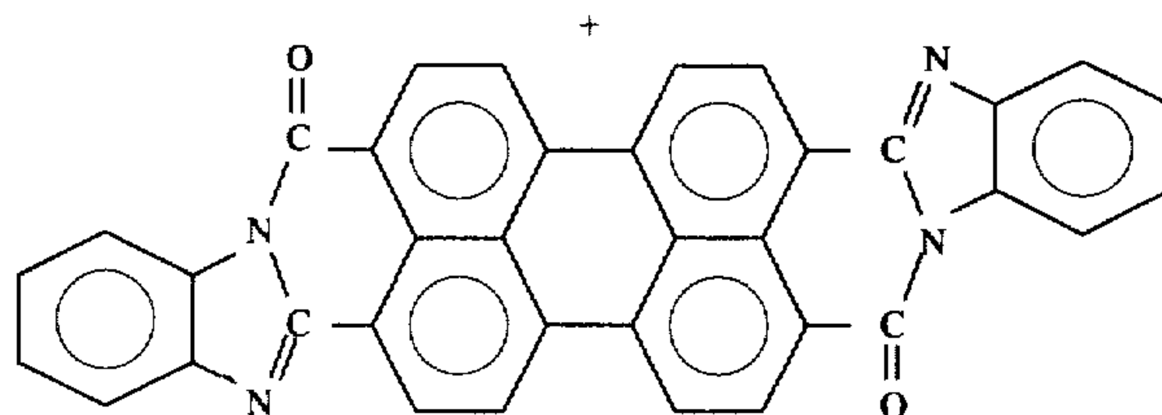
bisbenzimidazo(2,1-a-1',1'-b)anthra(2,1,9-def:6,5,10-d'e'f')disoquinoline-6,11-dione
