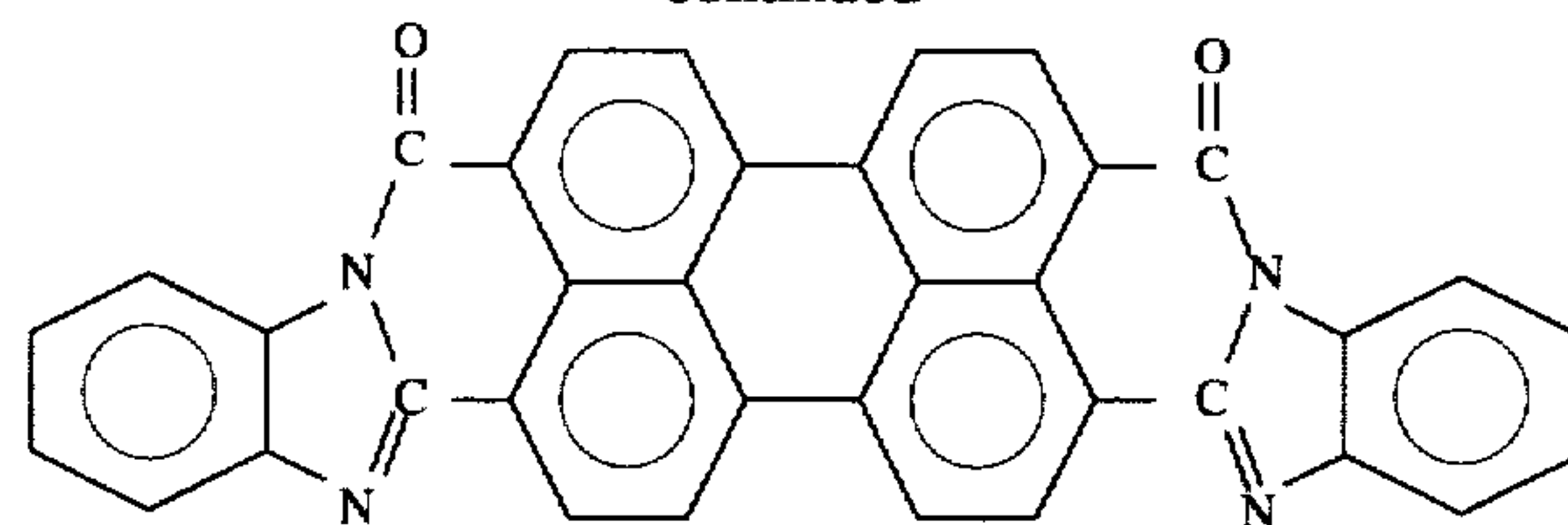
bisbenzimidazo(2,1-a-1',1'-b)anthra(2,1,9-def:6,5,10-d'e'f')disoquinoline-6,11-dione
