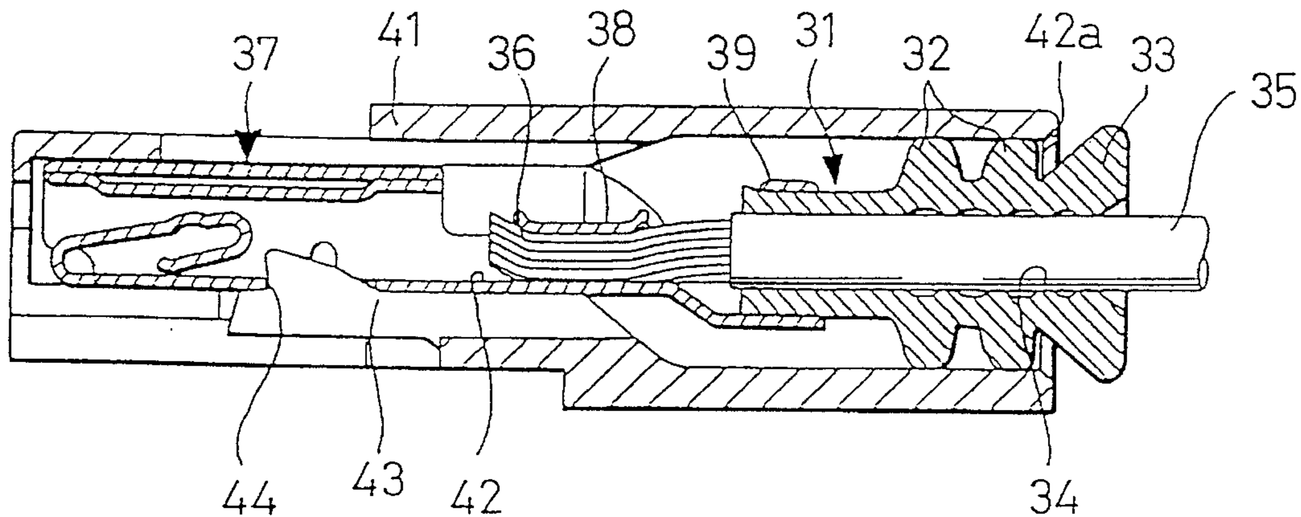
FIG. 5 PRIOR ART
