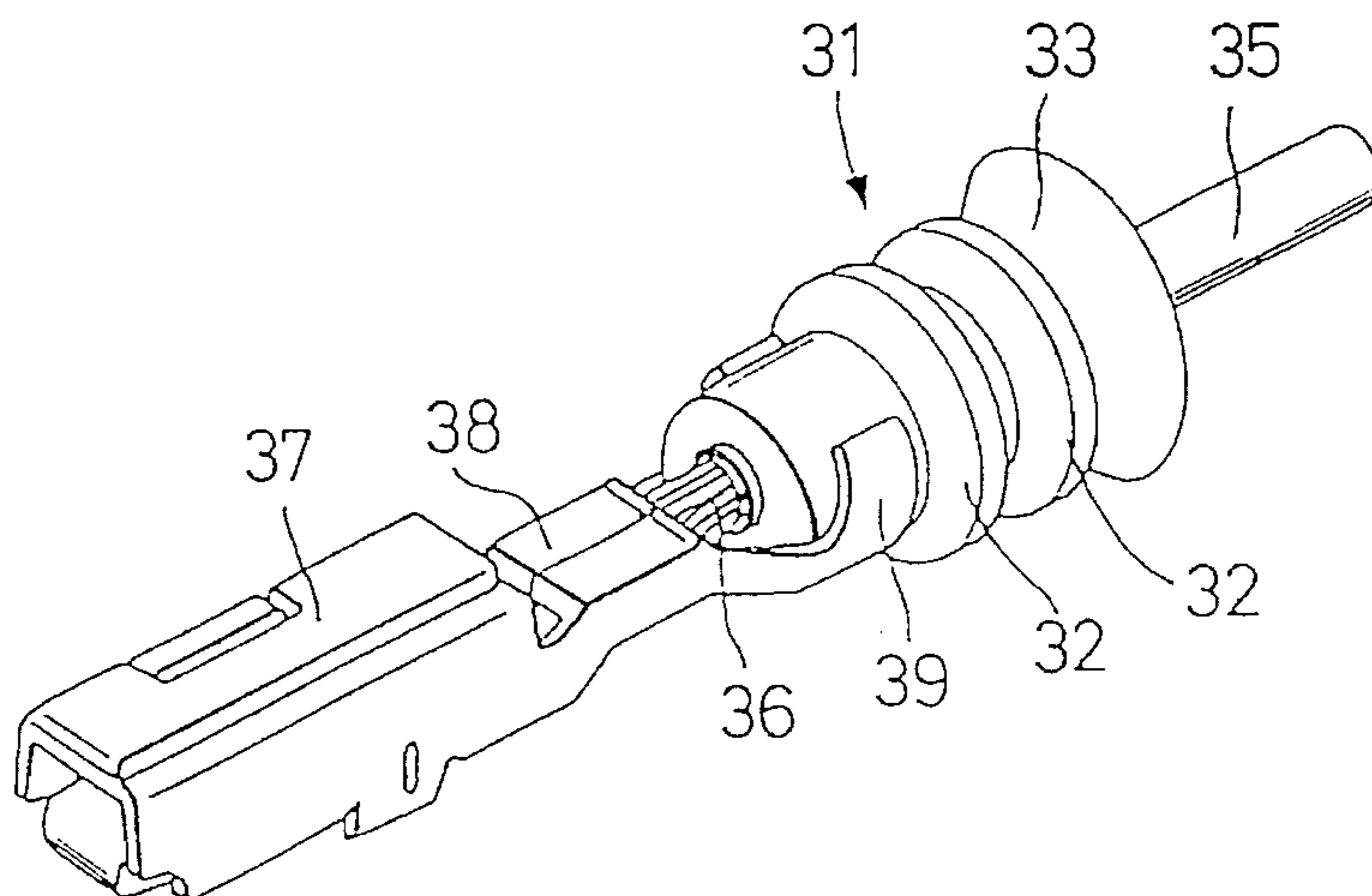
FIG. 4 PRIOR ART
