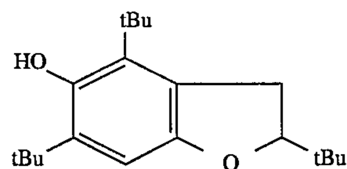
Comparative Compound 4
