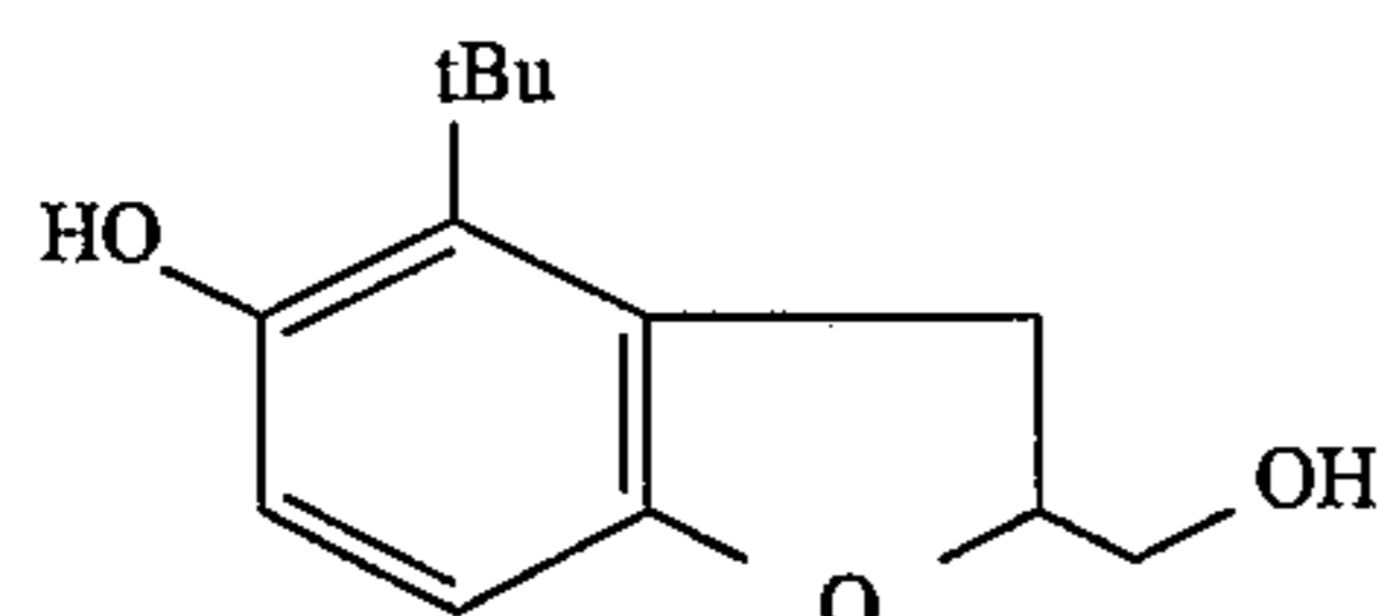
Comparative Compound 3
