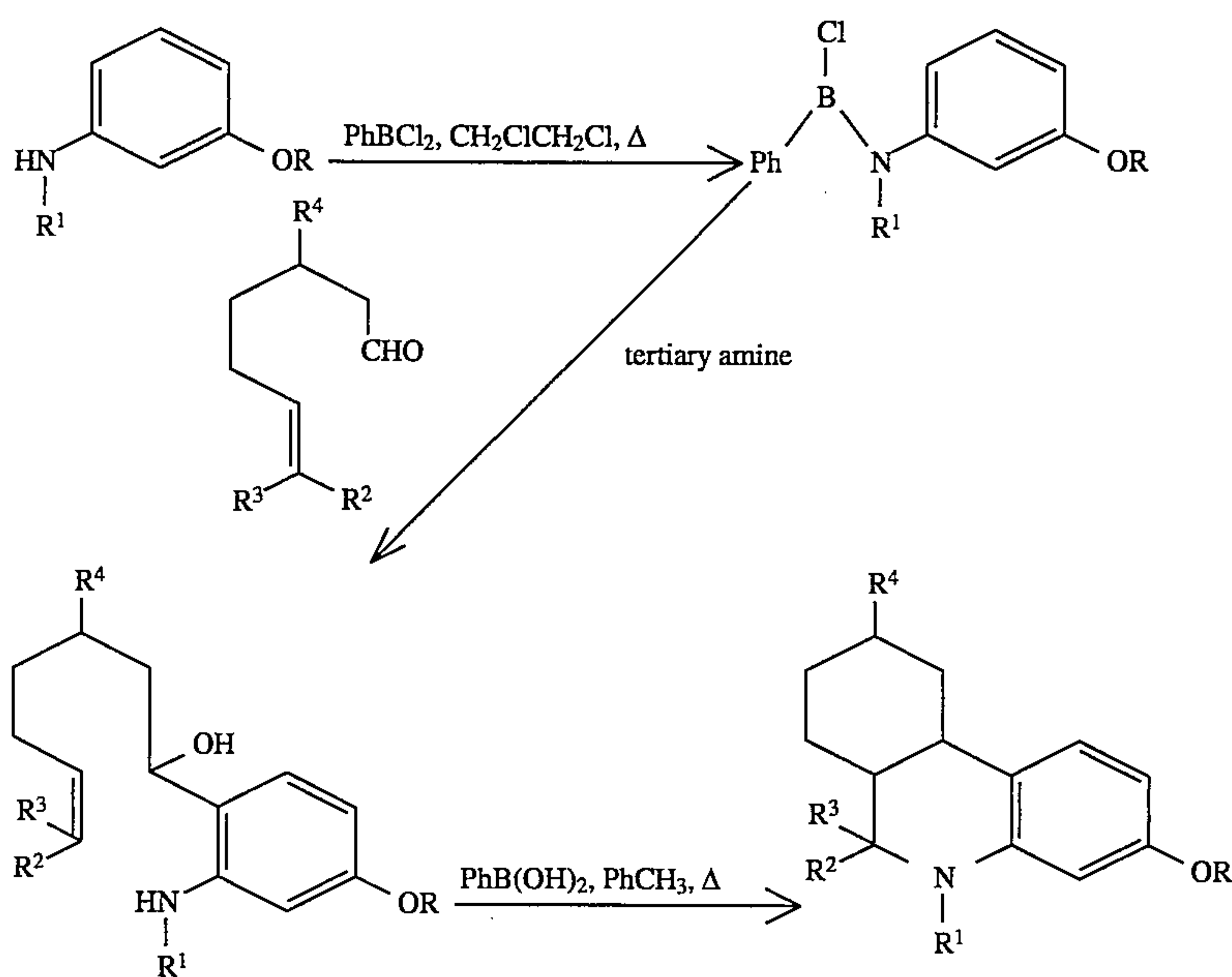
SCHEME 1
