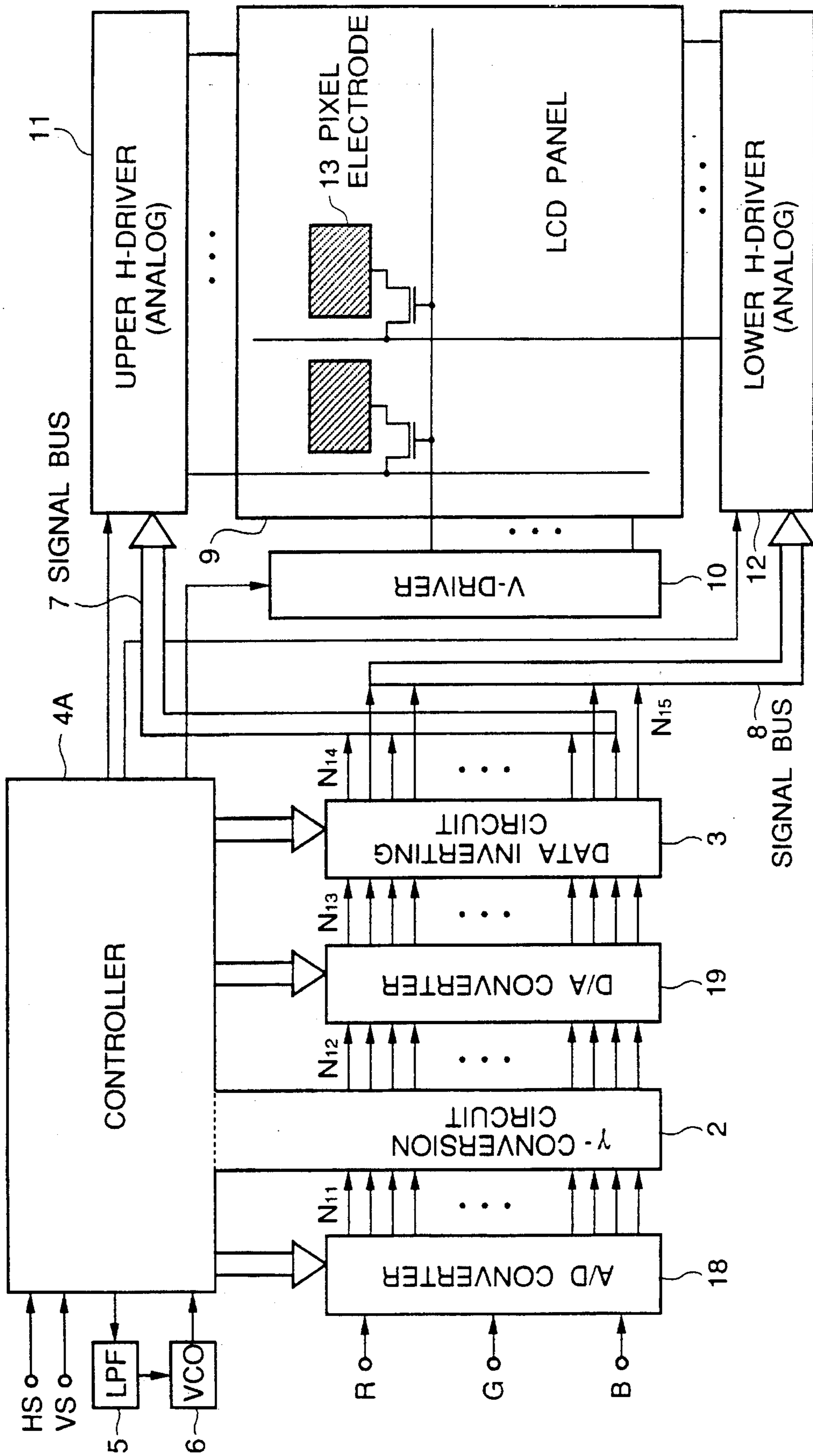
FIGURE 1 PRIOR ART
