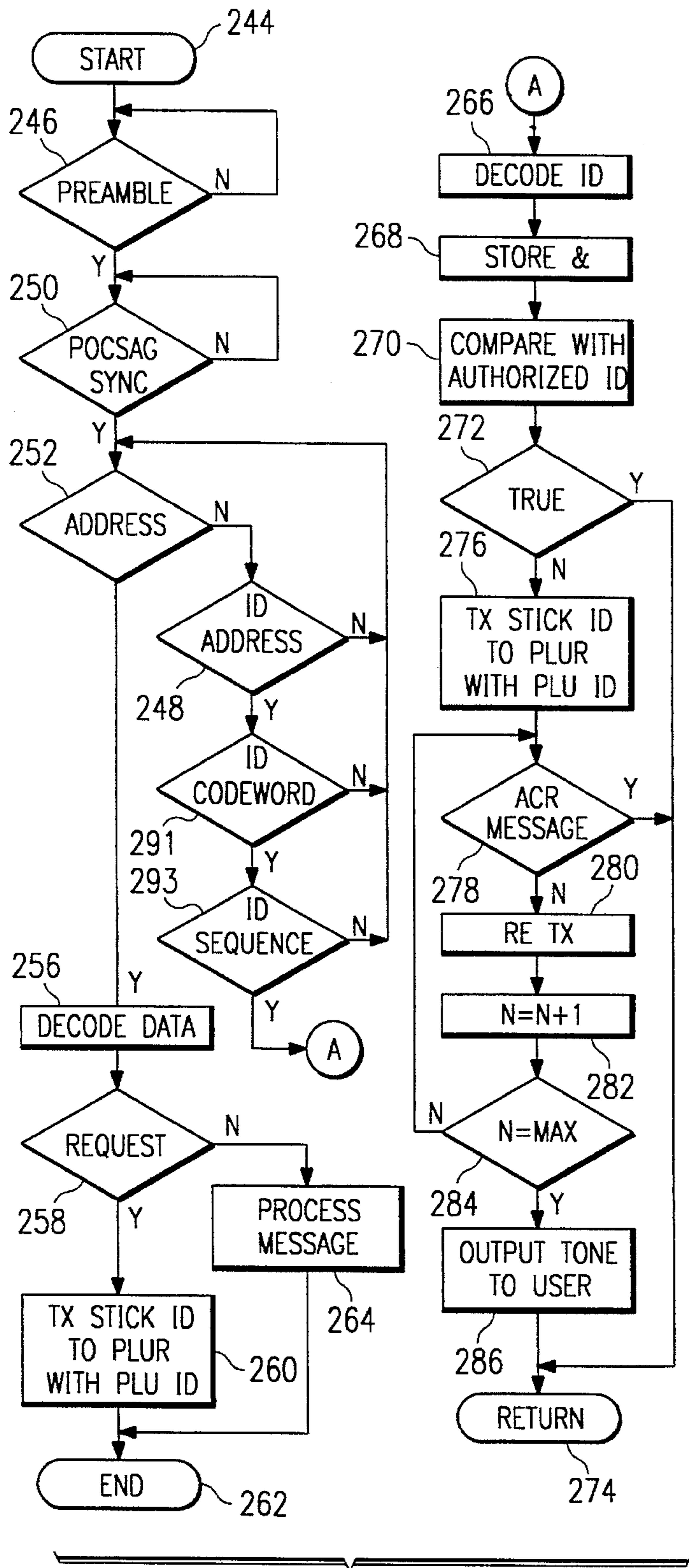
FIG. 9 PLU FLOW CHART
