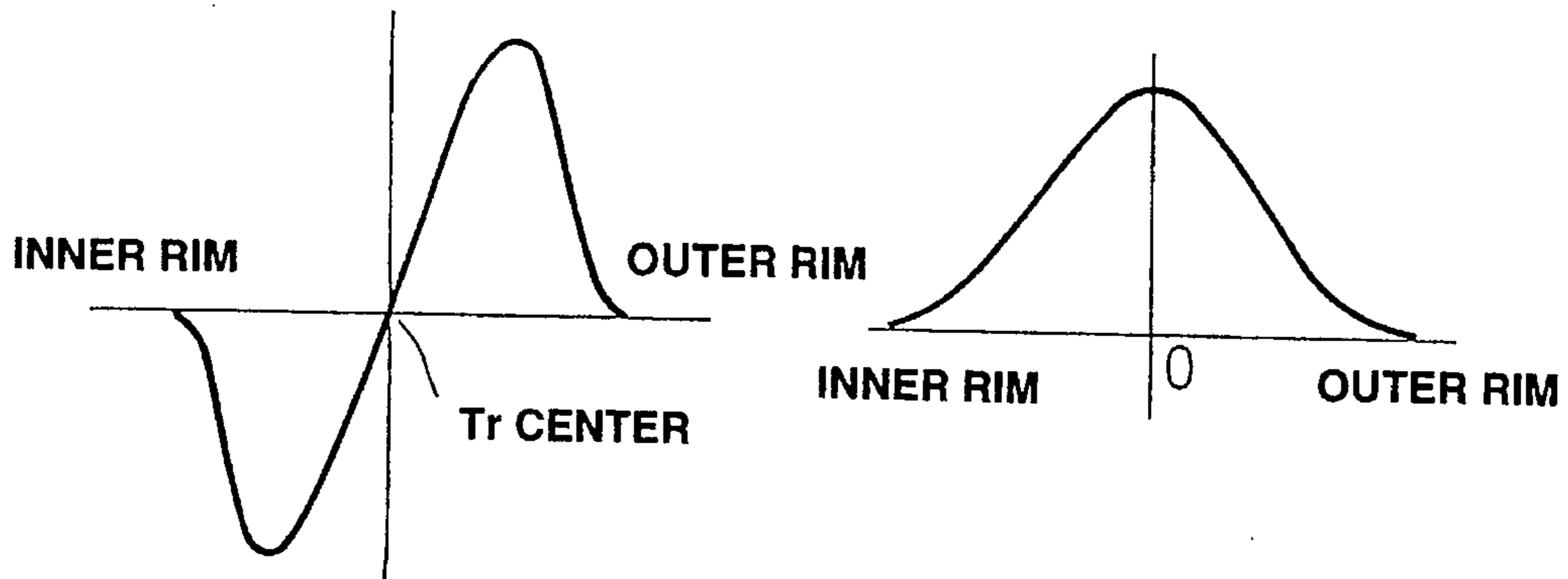
FIG. 19(a) PUSH-PULL SIGNAL
