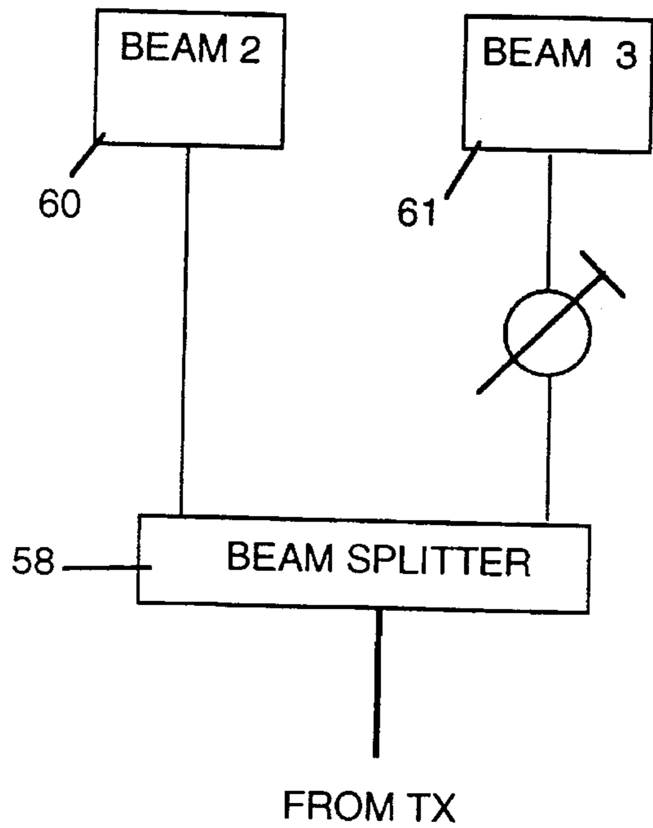
Fig. 14 (b) QUADRATURE
