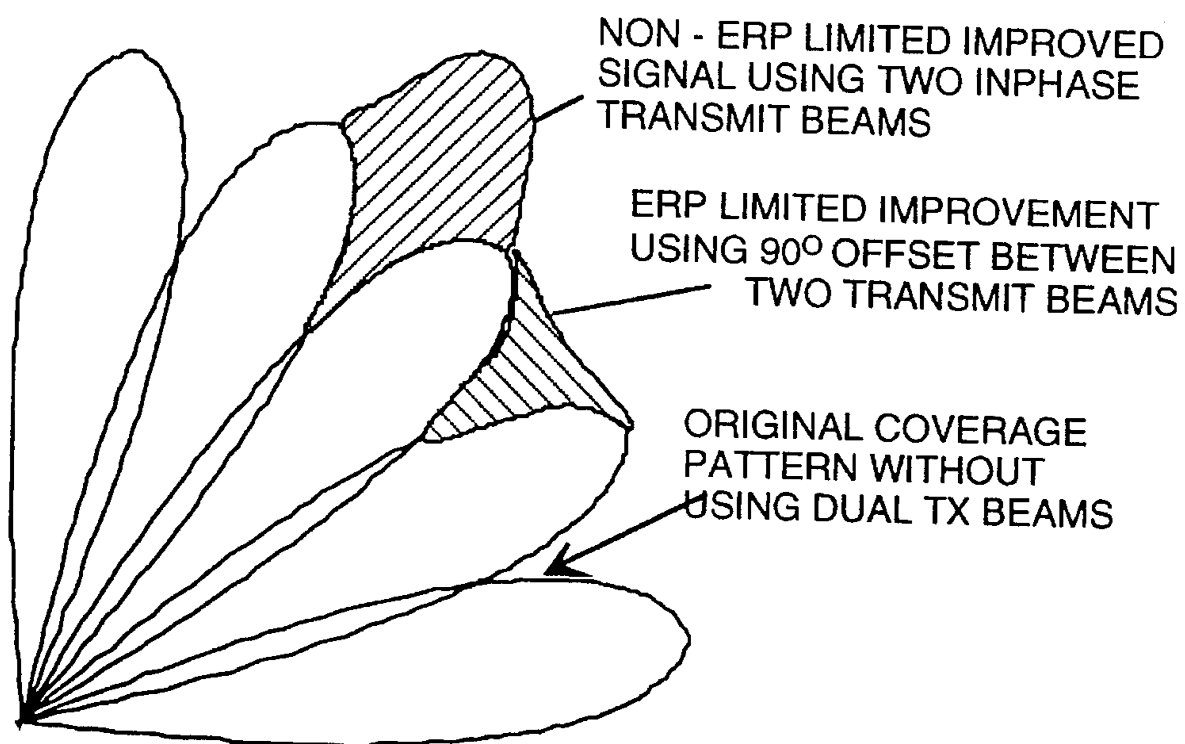
Fig. 14 (c)
