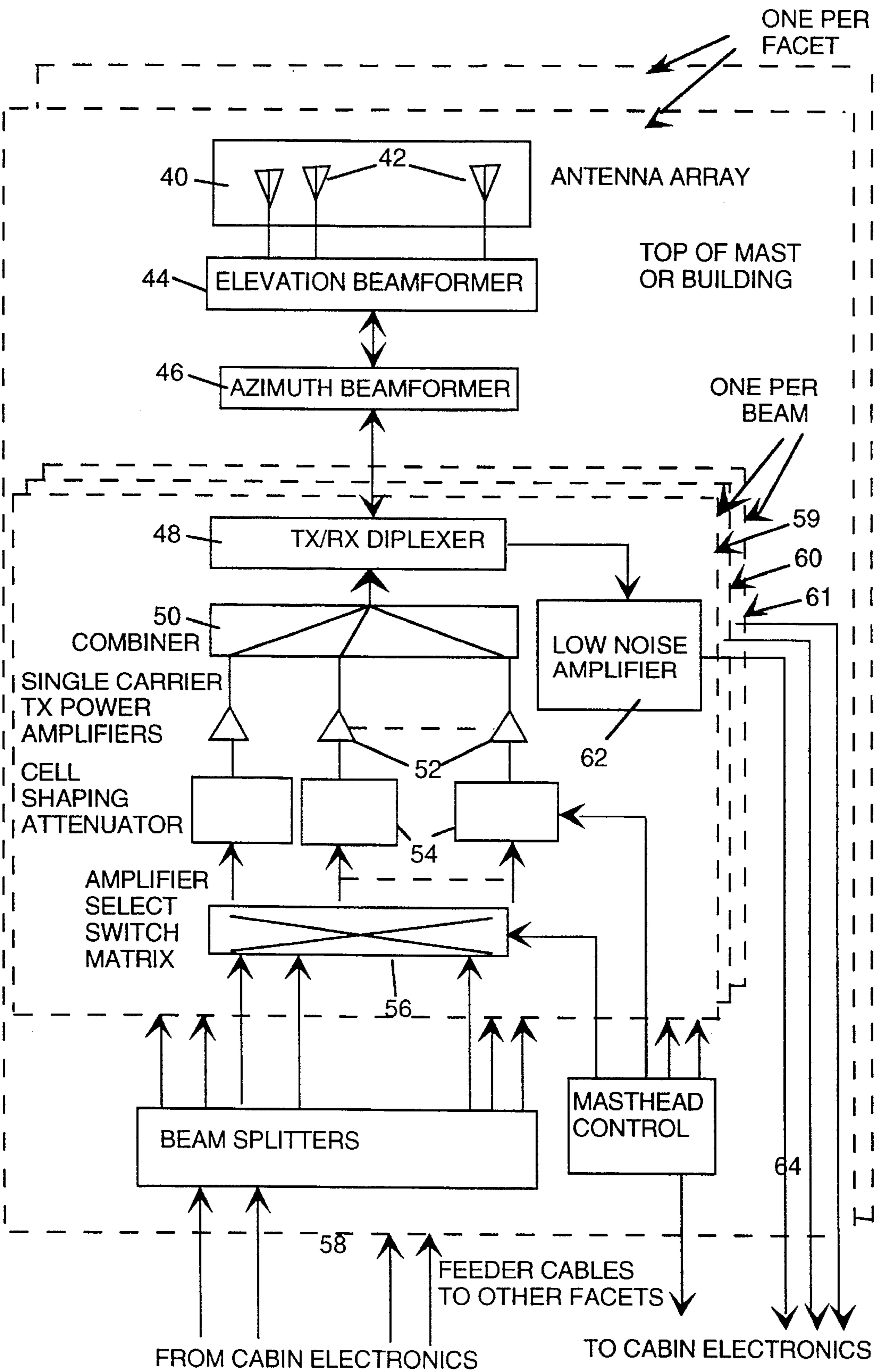
Fig. 6 (a)
