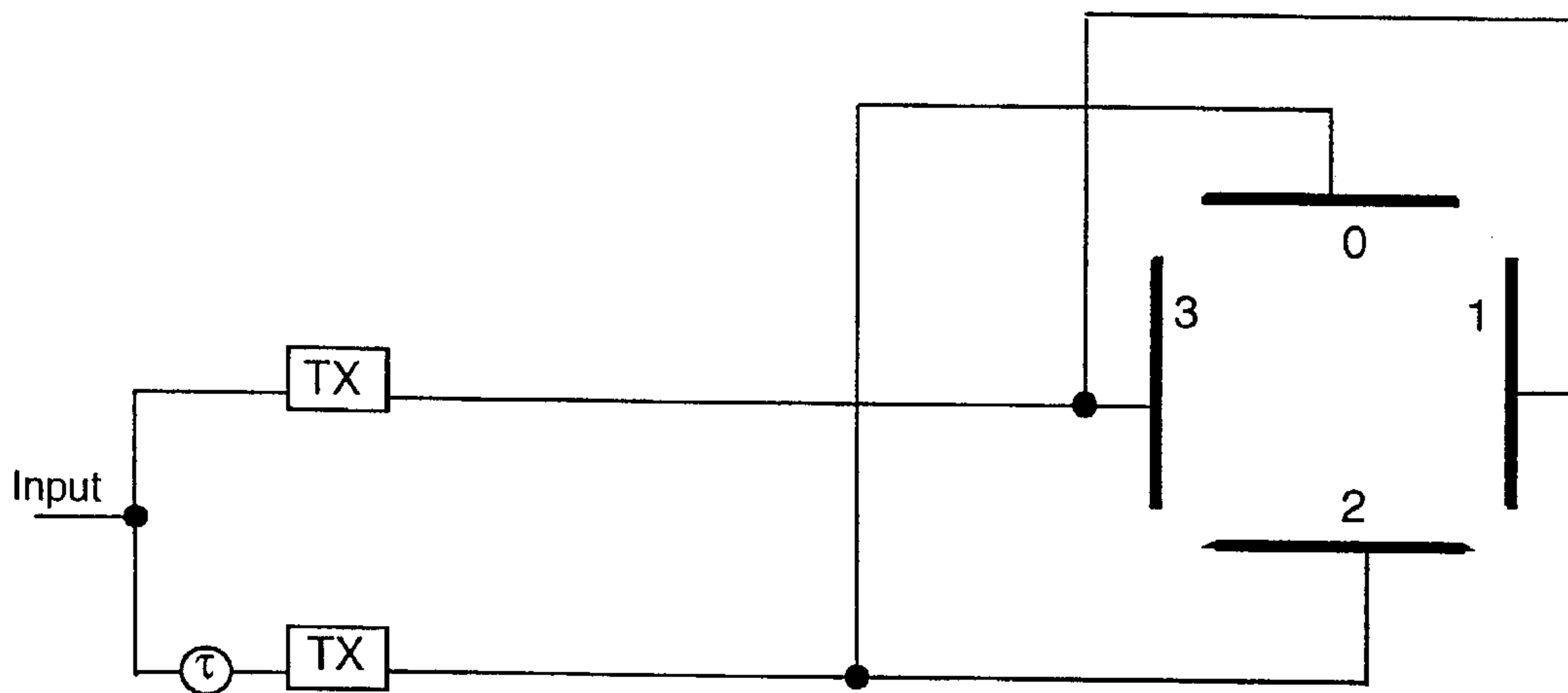
Fig. 12 (c)
