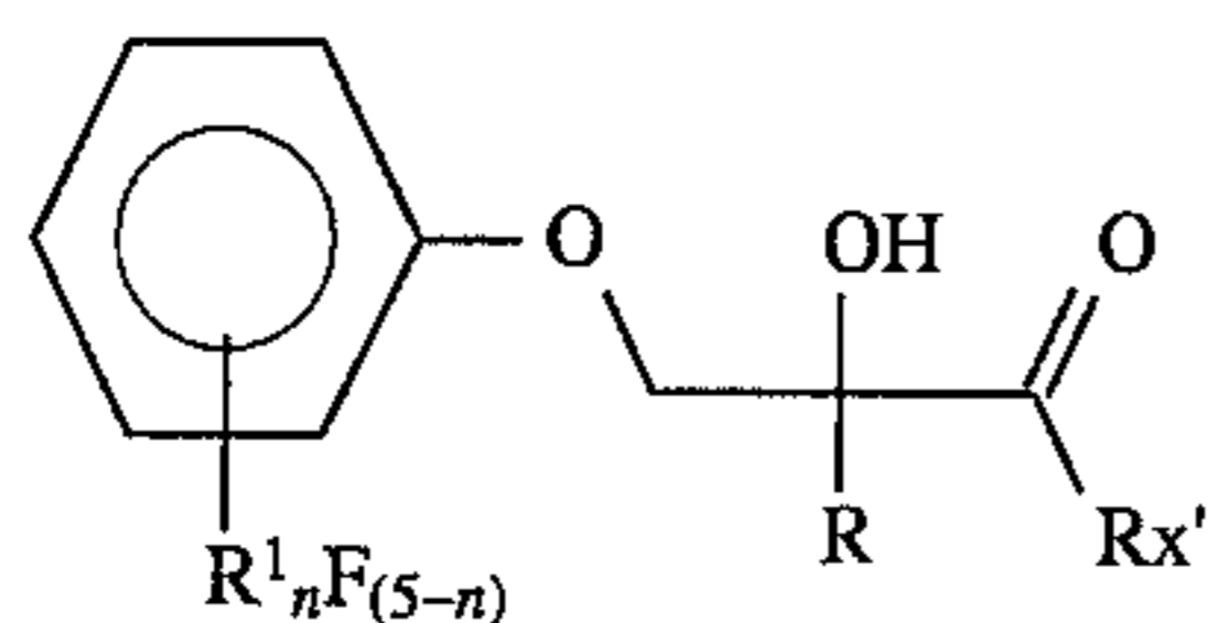
\alpha -Hydroxyketos 68
