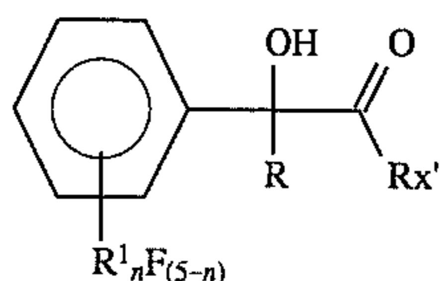
\alpha -Hydroxyketos 72
