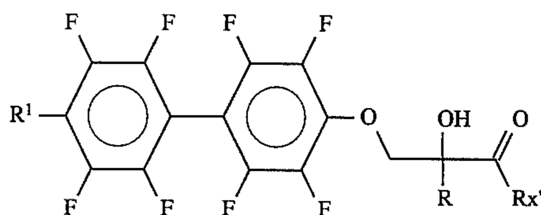
\alpha -Hydroxyketos 76
