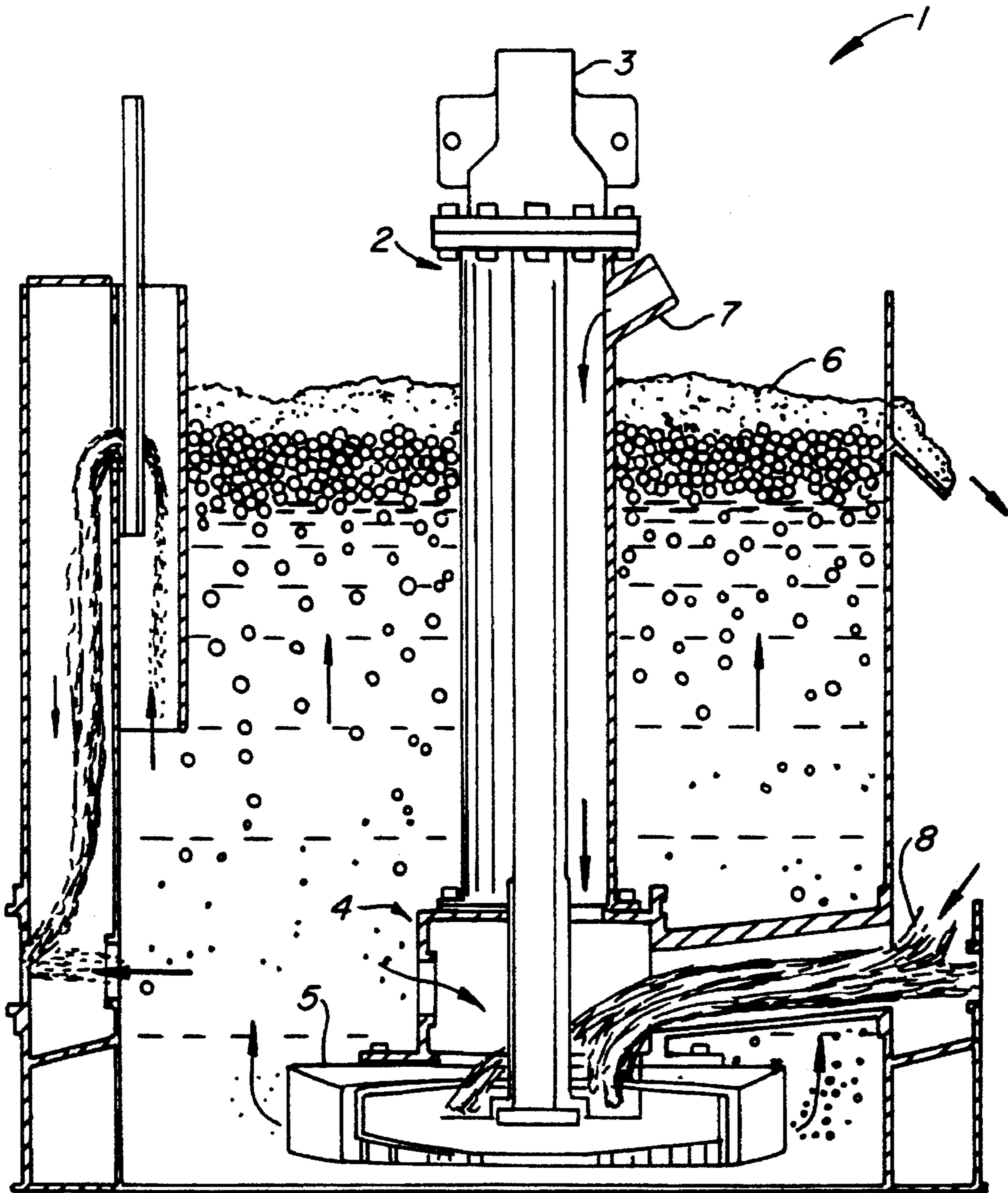
FIG. 1. PRIOR ART
