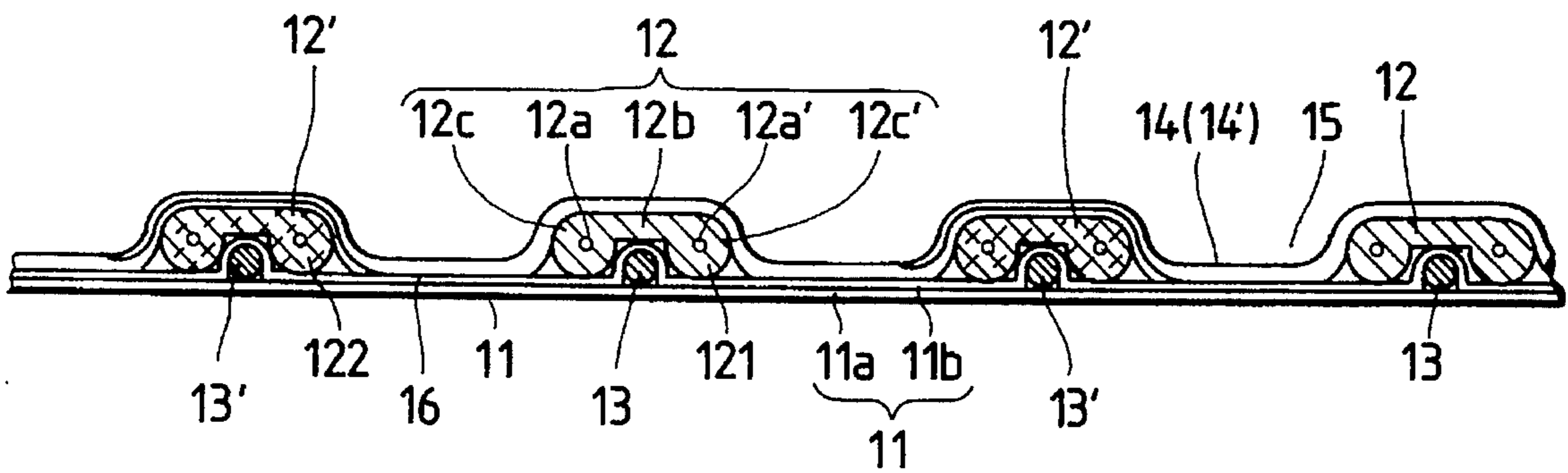
FIG. 8 PRIOR ART
