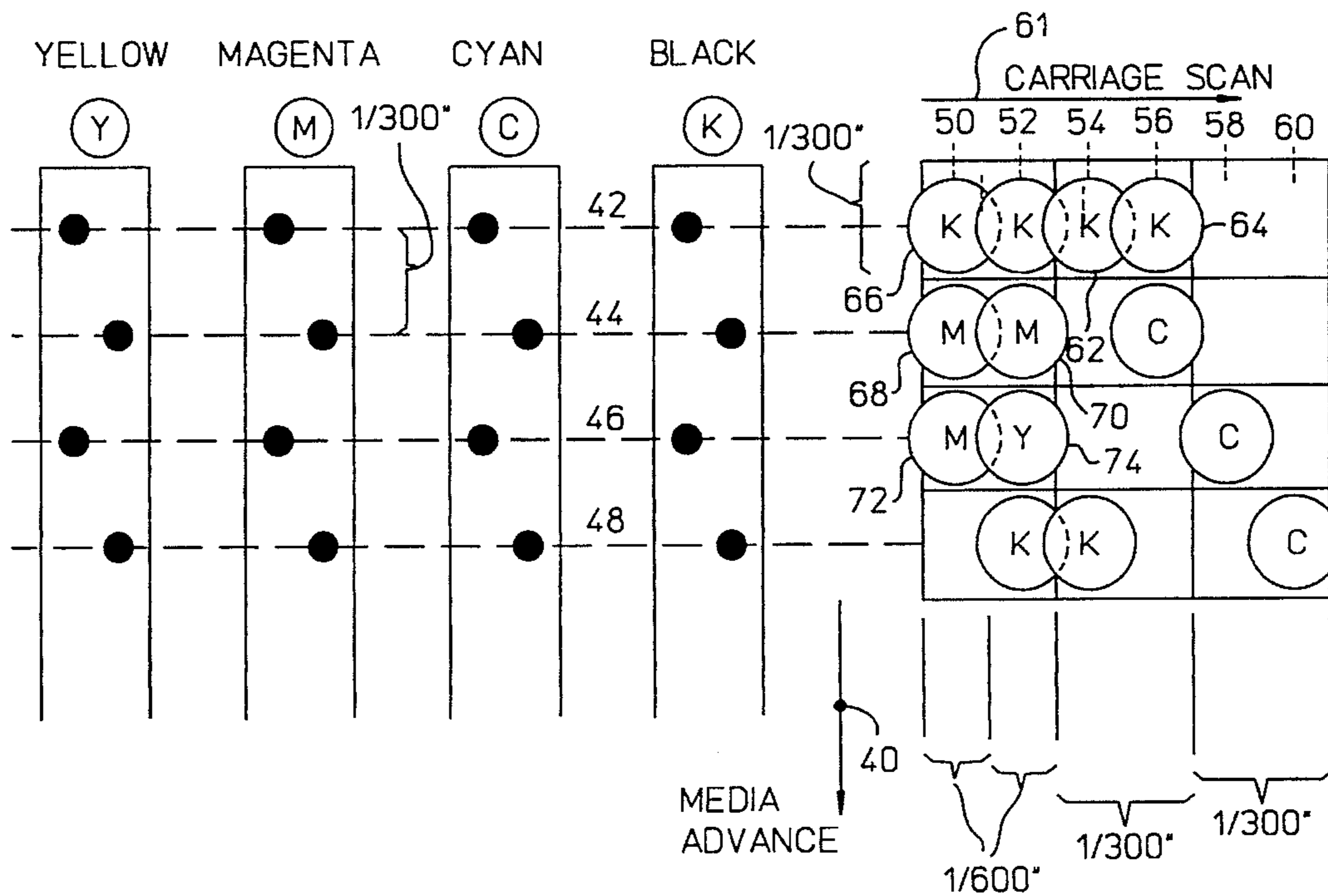
TOP VIEW OF PRINT CARTRIDGES
