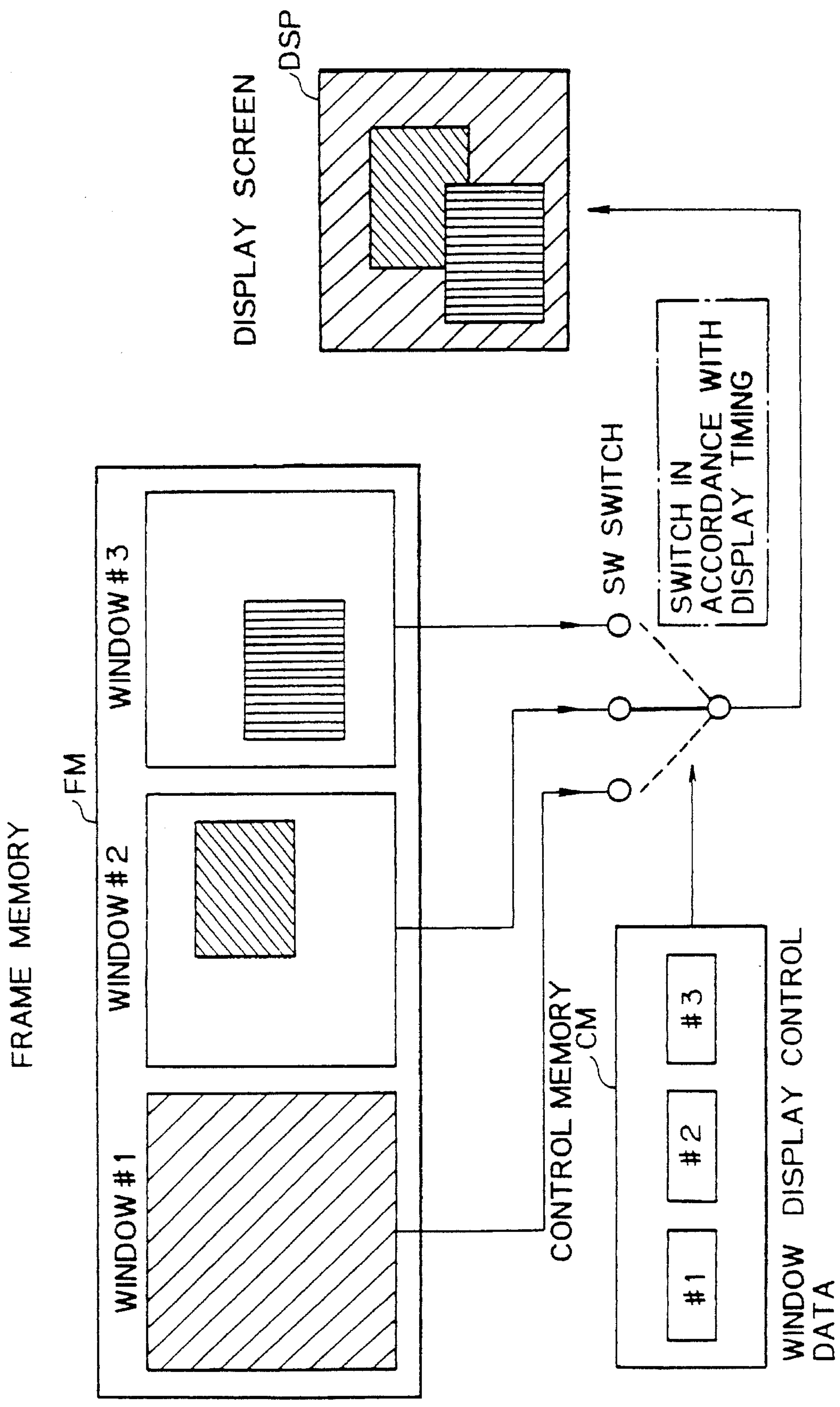
Fig. 23 PRIOR ART
