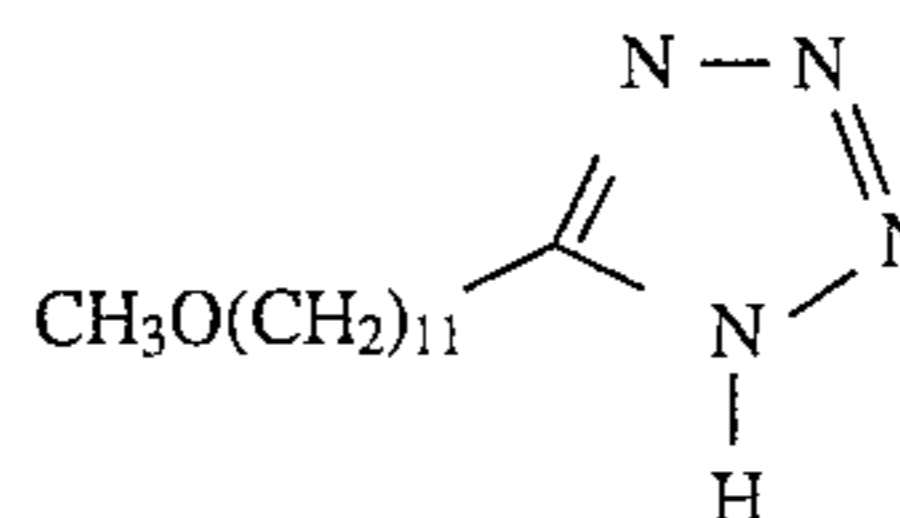
5-(11-Methoxyundecyl)-1H-tetrazole
