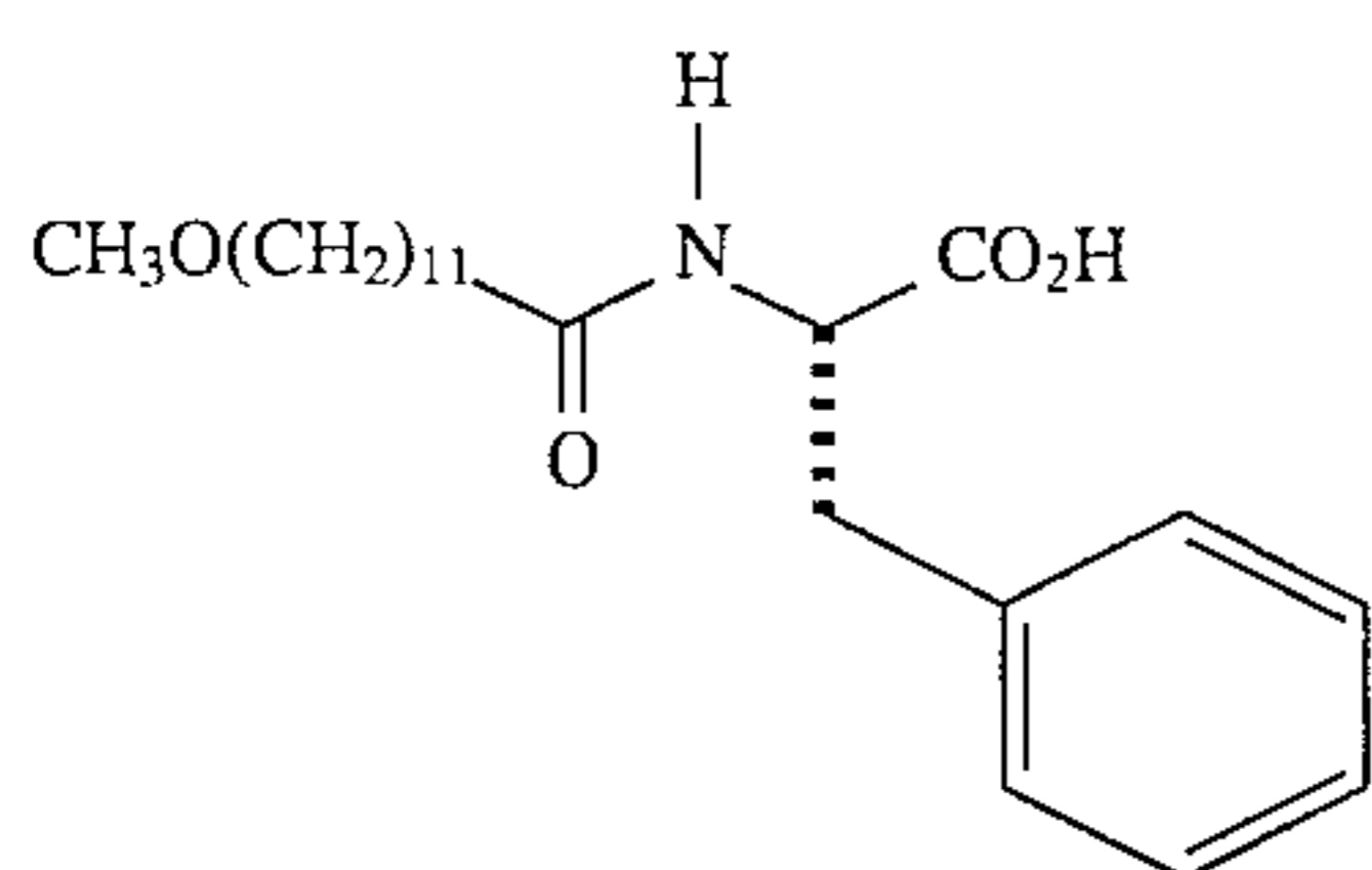
N-(12-Methoxy-1-oxododecyl)-L-phenylalanine
