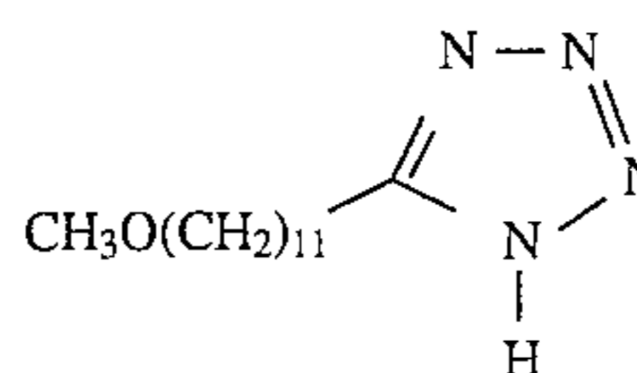
5-(11-Methoxyundecyl)-1H-tetrazole
