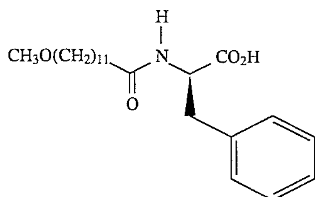
N-(12-Methoxy-1-oxododecyl)-D-phenylalanine
