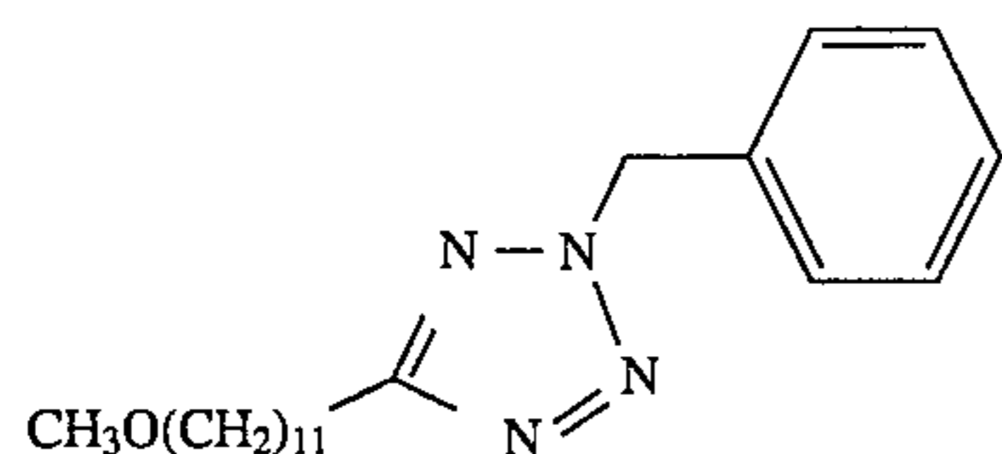
5-(11-Methoxyundecyl)-1-(phenylmethyl)-1H-tetrazole
