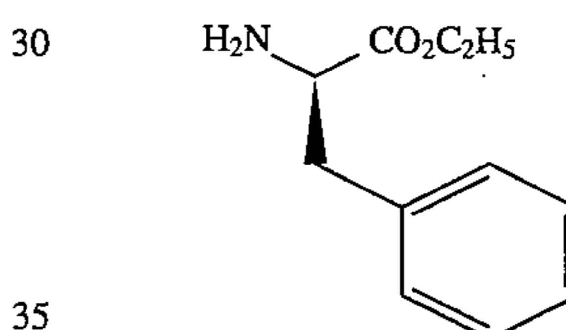
D-Phenylalanine Ethyl ester p-Toluenesulfonate
