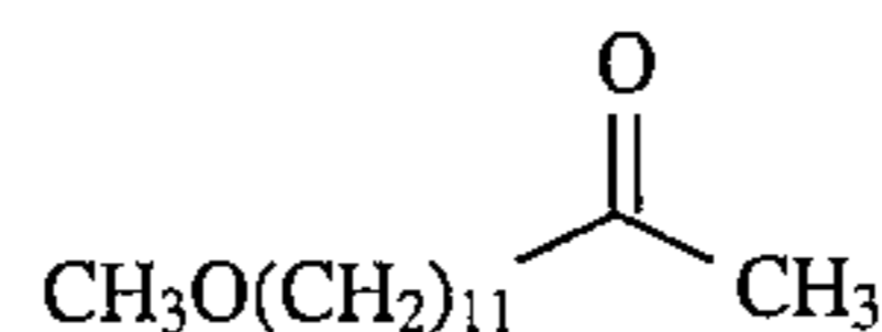
13-Methoxy-2-tridecanone
