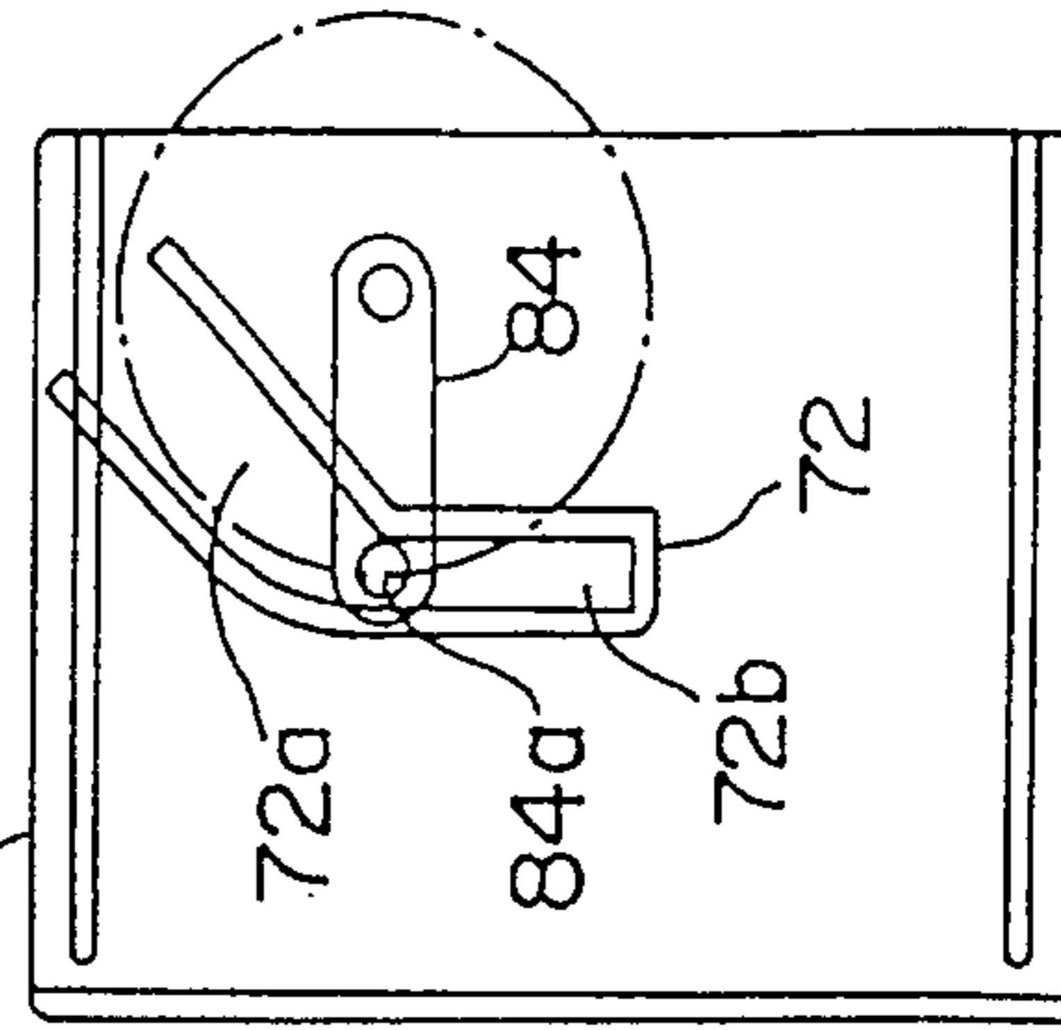
71 CHUCKING POSITION
