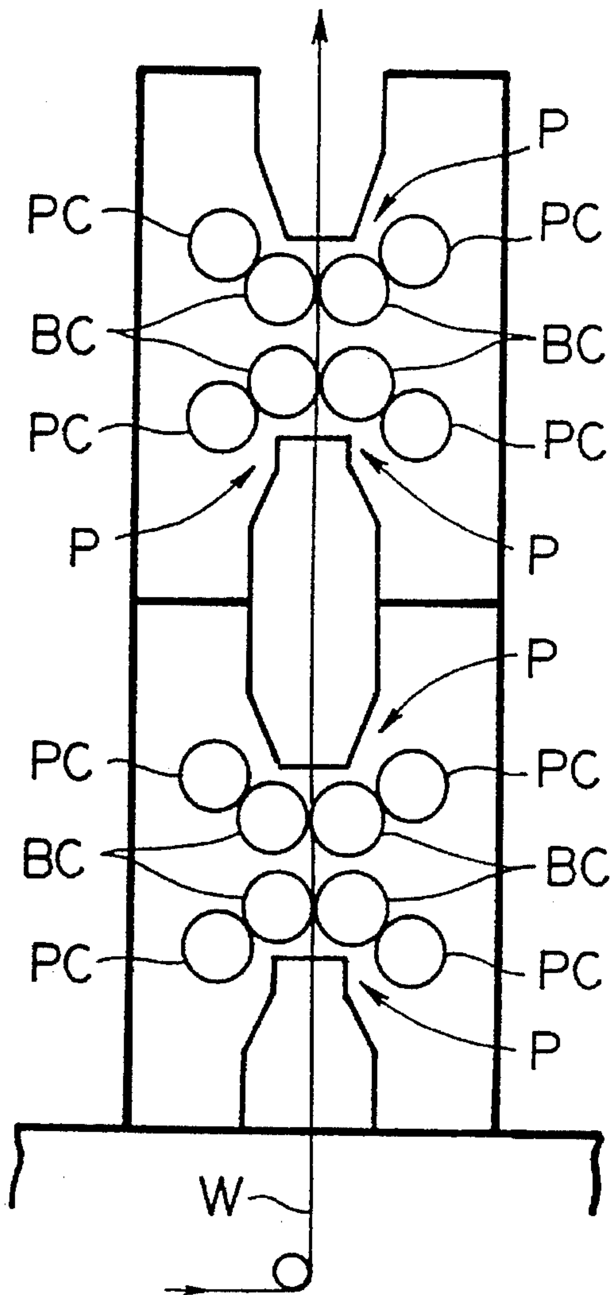
FIG. 5 PRIOR ART
